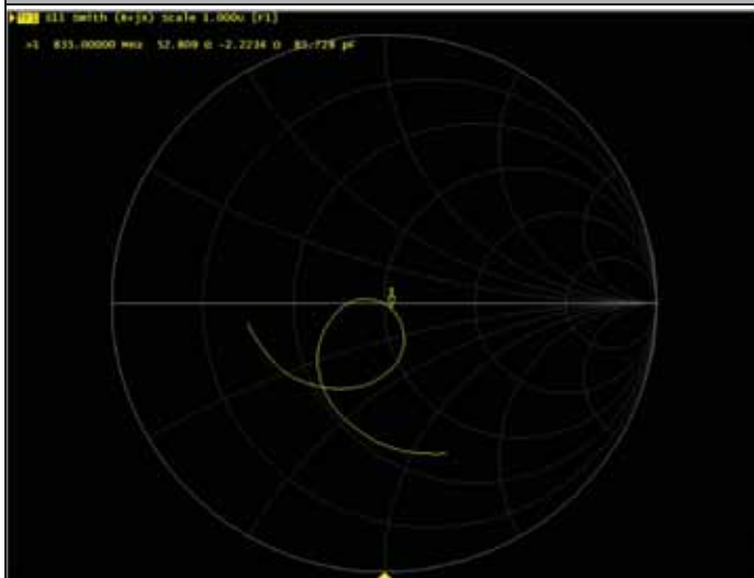
Impedance Test-Body
