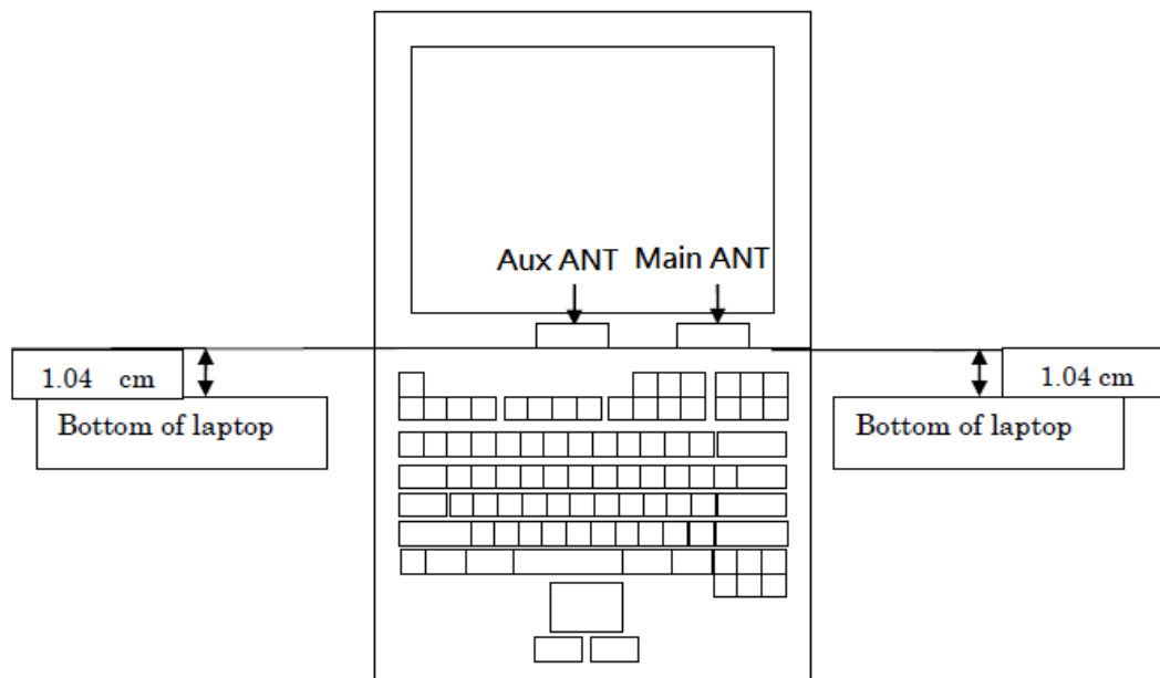
Fig.6 Antenna position of EUT (Front view)
