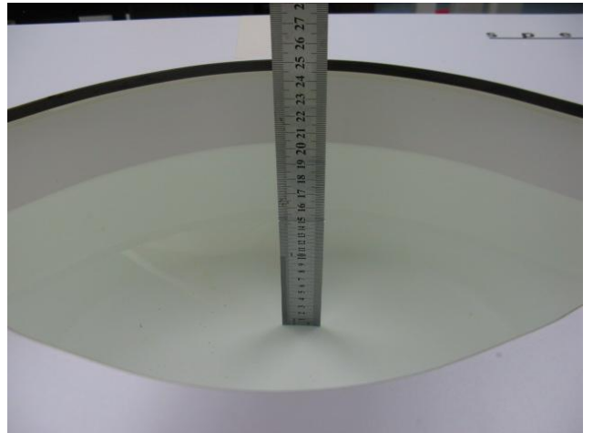
Photo 10: MSL 1900MHz depth (15.1cm)
