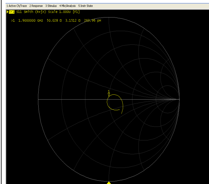
Impedance Test-Body
