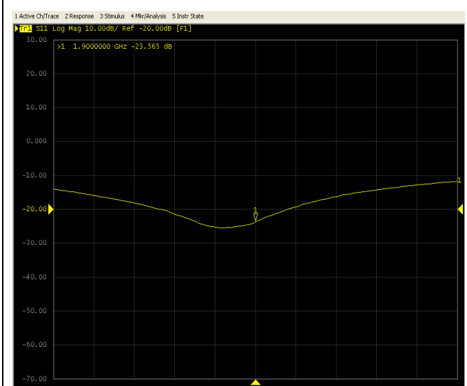
Return Loss Test-Body
