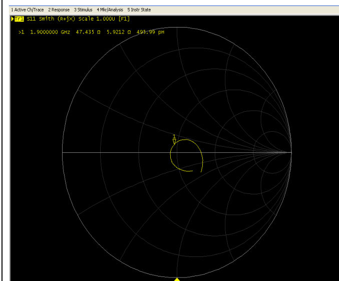
Impedance Test-Body
