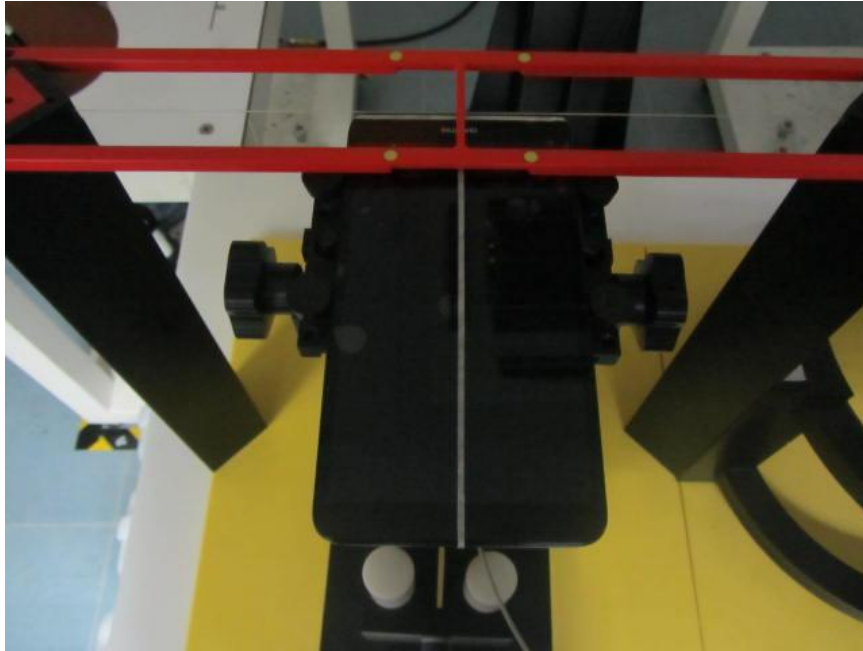
HAC T-coil test photo
