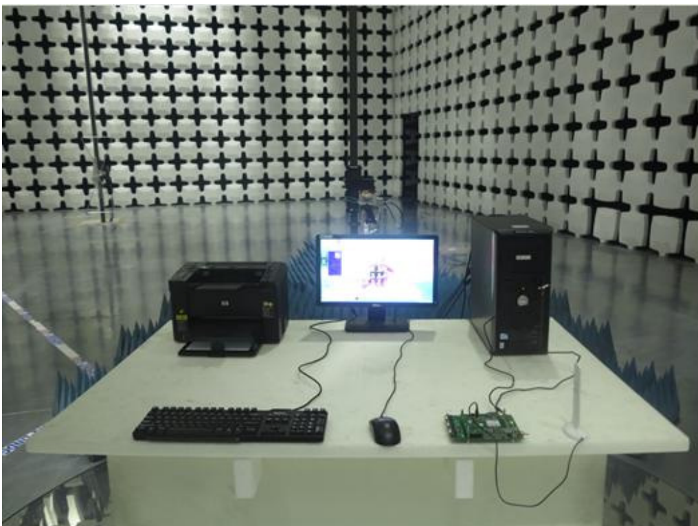
Radiated Emission (Part15B Usb mode) -1GHz-18GHz
