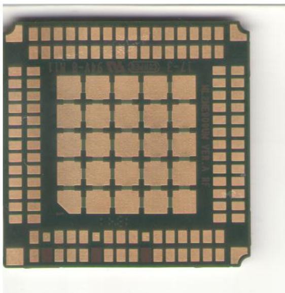
Figure1 EUT Appearance
