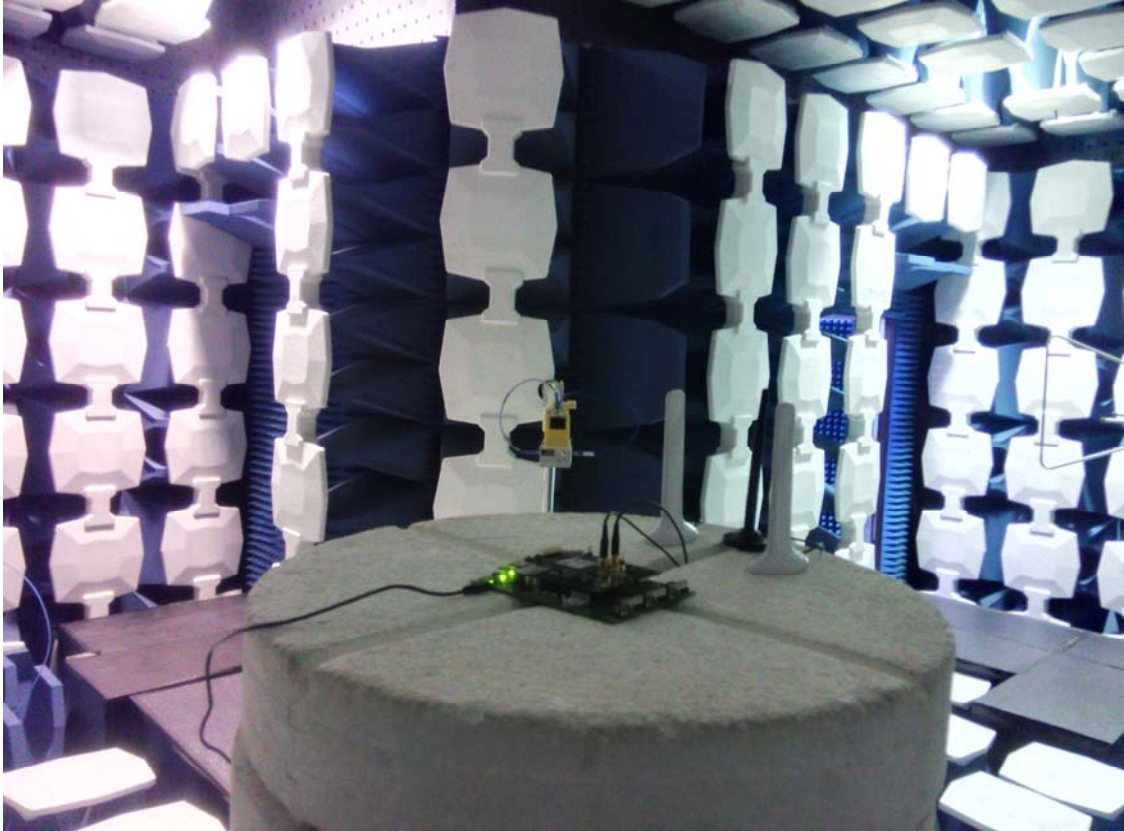
Radiated Spurious Emission (18GHz to26.5GHz)
