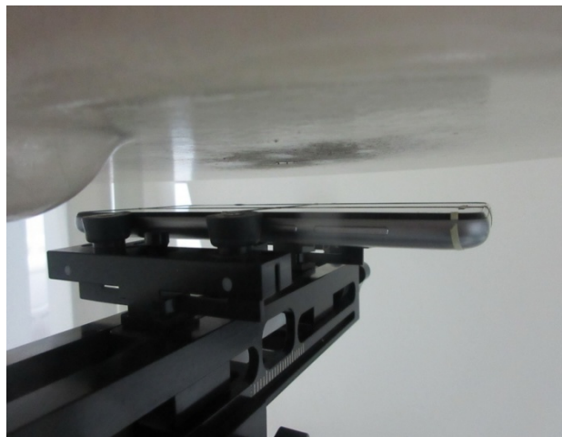
Photo 12: Front Face_15mm
