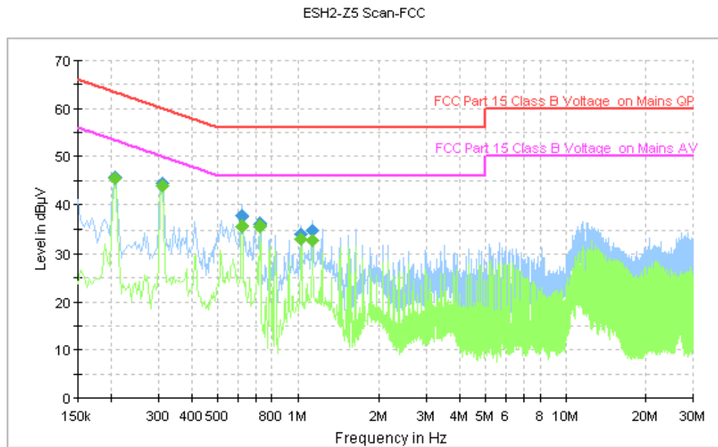
Figure A.29 Conducted Emission
