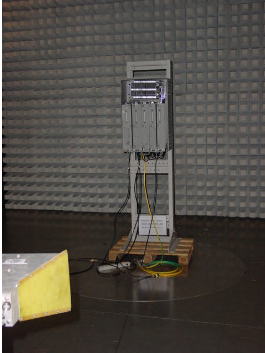
Photo ERP measurement 1 GHz – 10 GHz
