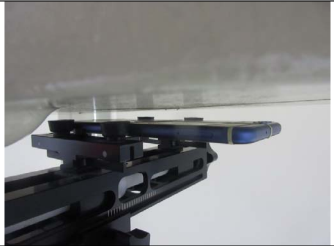
Photo 12: Rear Face_1cm
