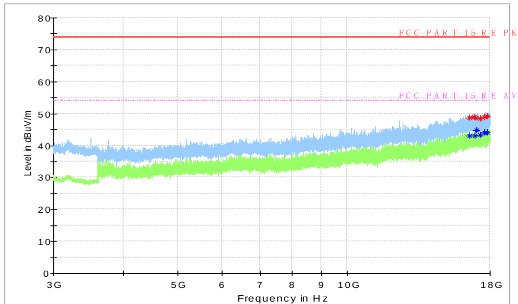
Figure A.72 Radiated Emission from 3GHz to 18GHz
