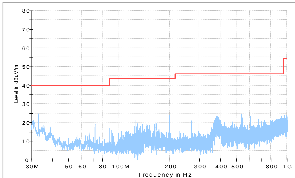
Figure A.85 Radiated Emission from 30MHz to 1GHz
