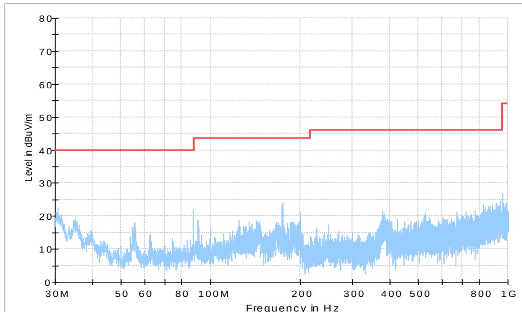
Figure A.67 Radiated Emission from 30MHz to 1GHz
