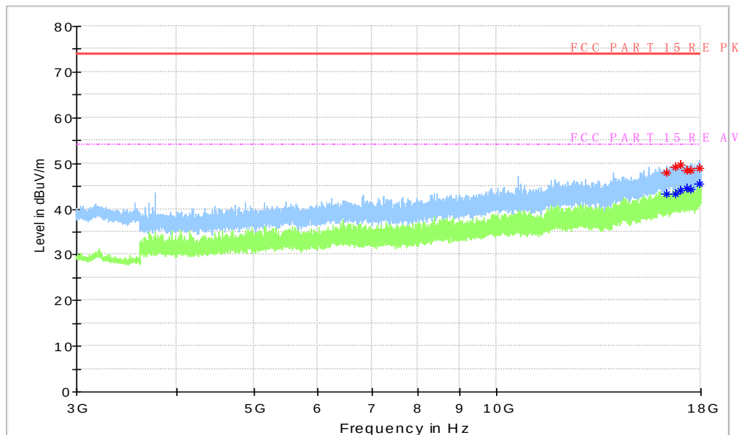
Figure A.87 Radiated Emission from 3GHz to 18GHz
