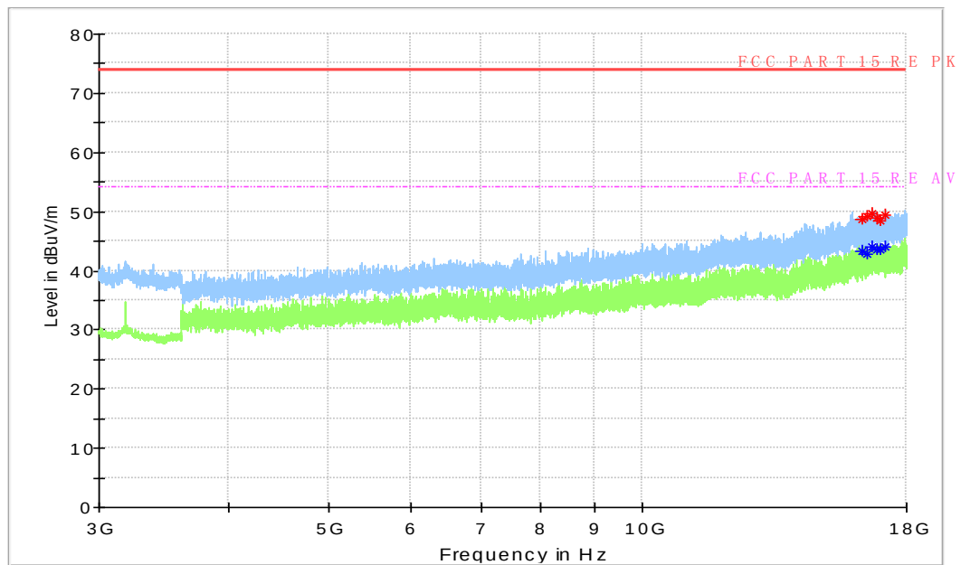
Figure A.81 Radiated Emission from 3GHz to 18GHz
