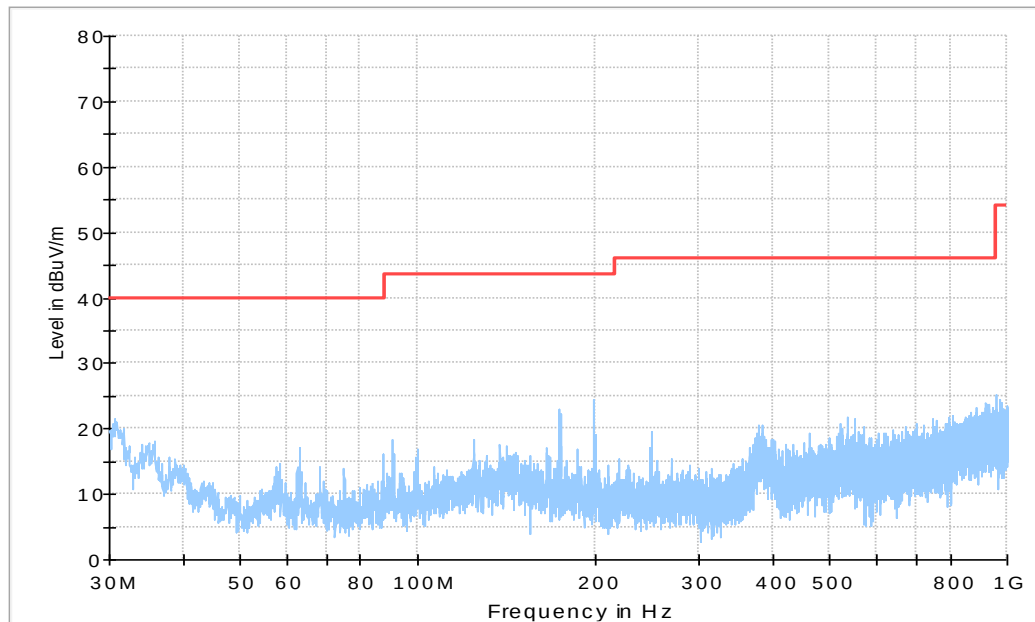
Figure A.70 Radiated Emission from 30MHz to 1GHz
