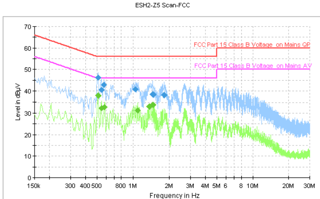
Figure A.113 Conducted Emission
