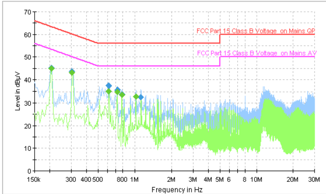
Figure A.142 Conducted Emission
