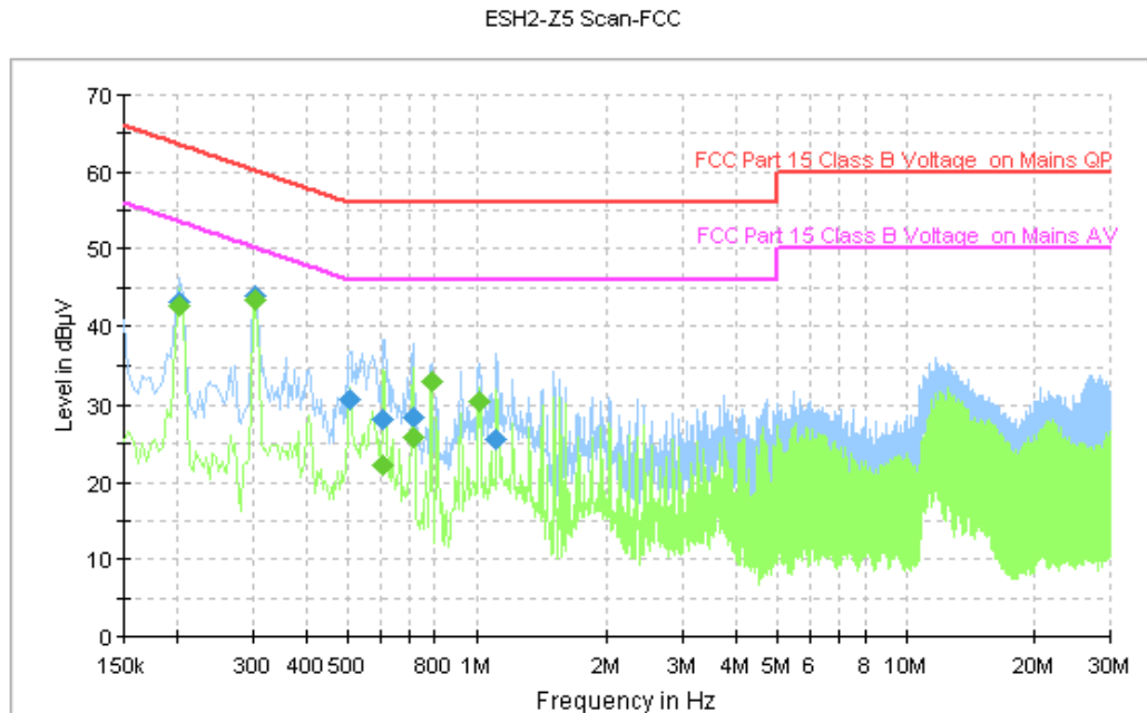
Figure A.130 Conducted Emission
