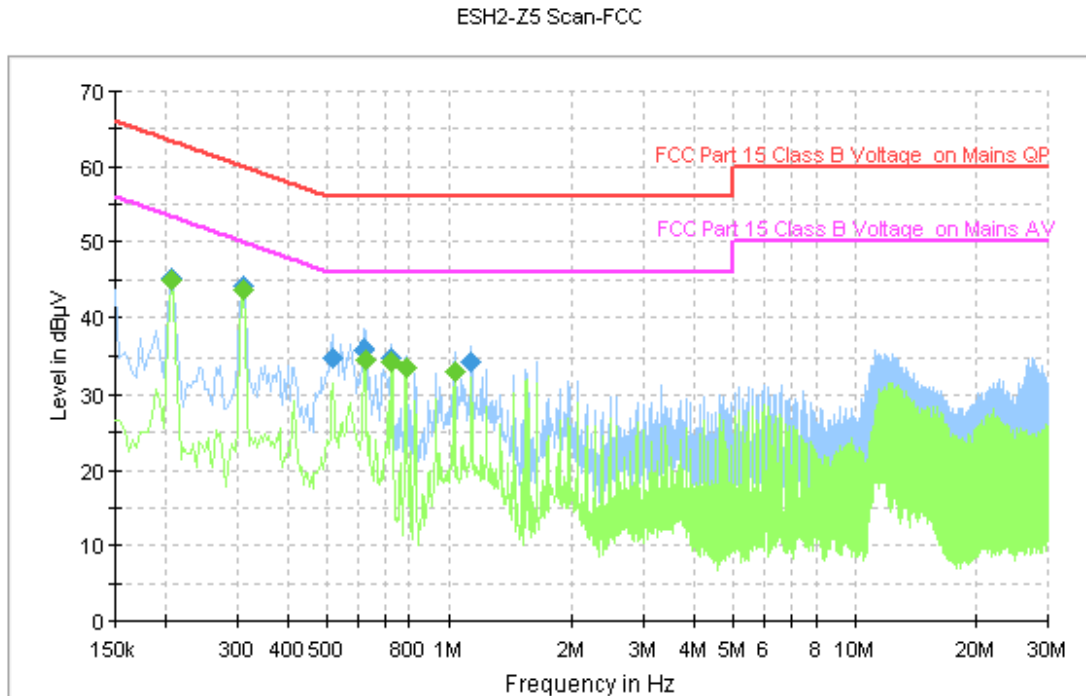
Figure A.146 Conducted Emission
