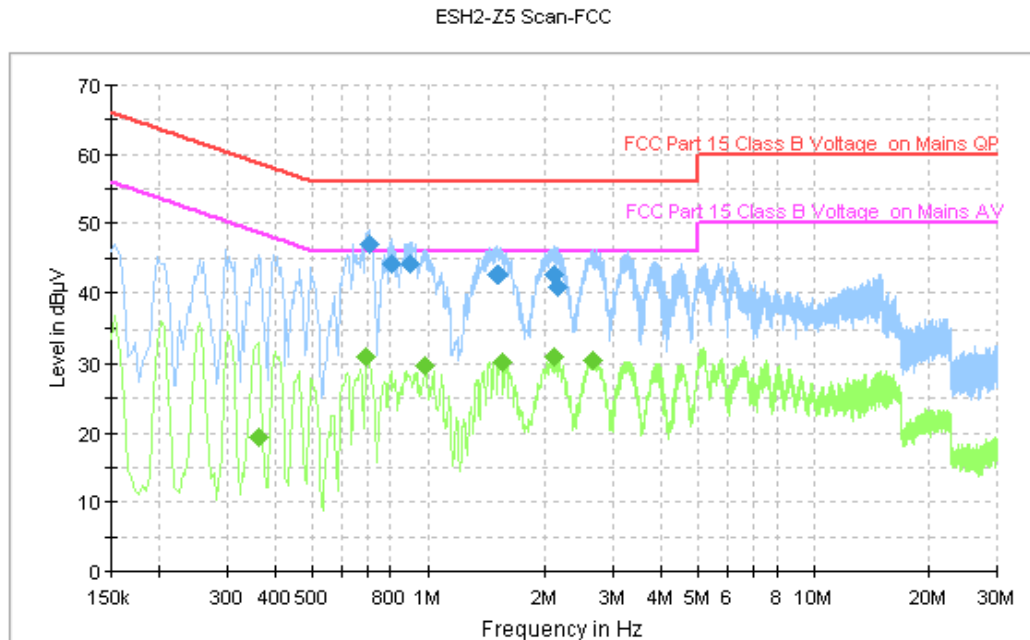
Figure A.124 Conducted Emission
