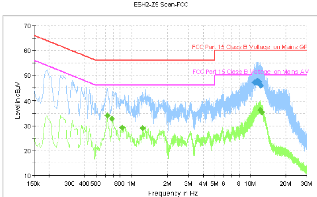
Figure A.116 Conducted Emission
