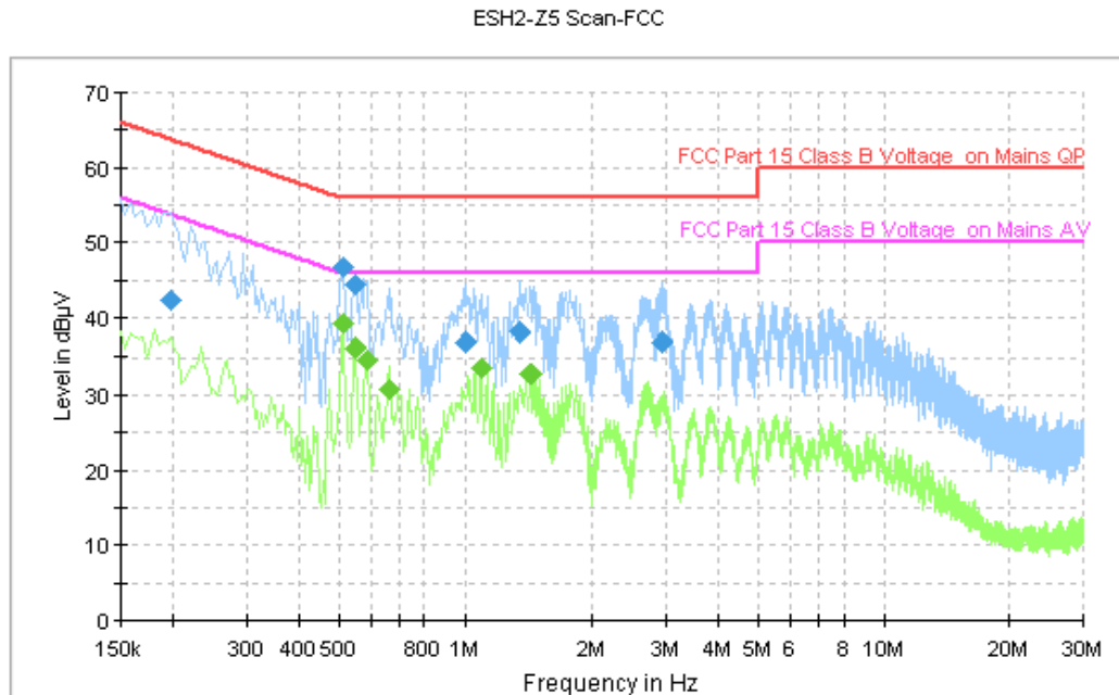
Figure A.114 Conducted Emission
