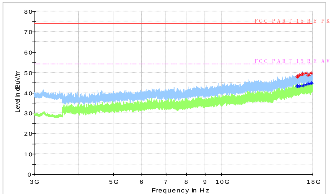
Figure A.78 Radiated Emission from 3GHz to 18GHz
