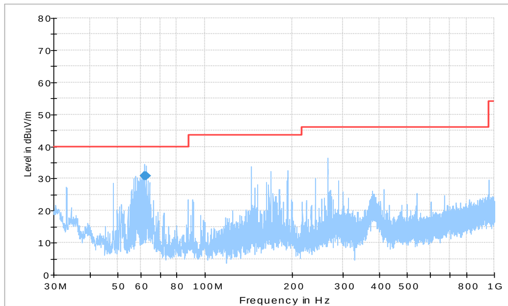
Figure A.64 Radiated Emission from 30MHz to 1GHz
