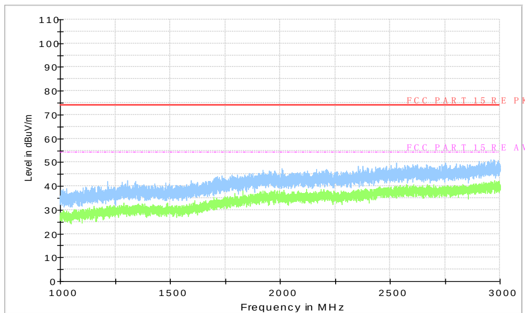
Figure A.71 Radiated Emission from 1Gz to 3GHz
