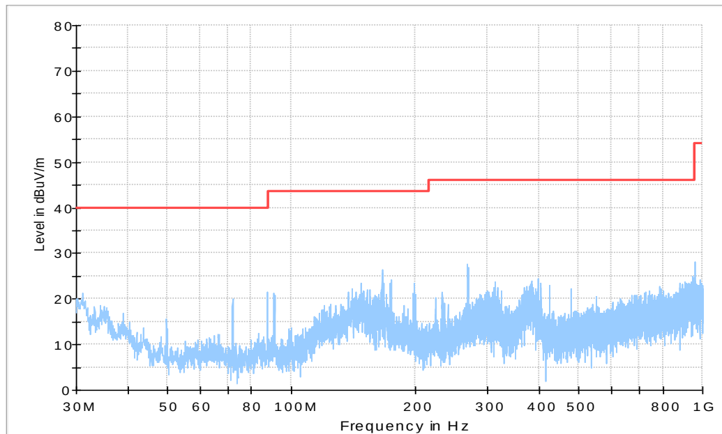
Figure A.88 Radiated Emission from 30MHz to 1GHz
