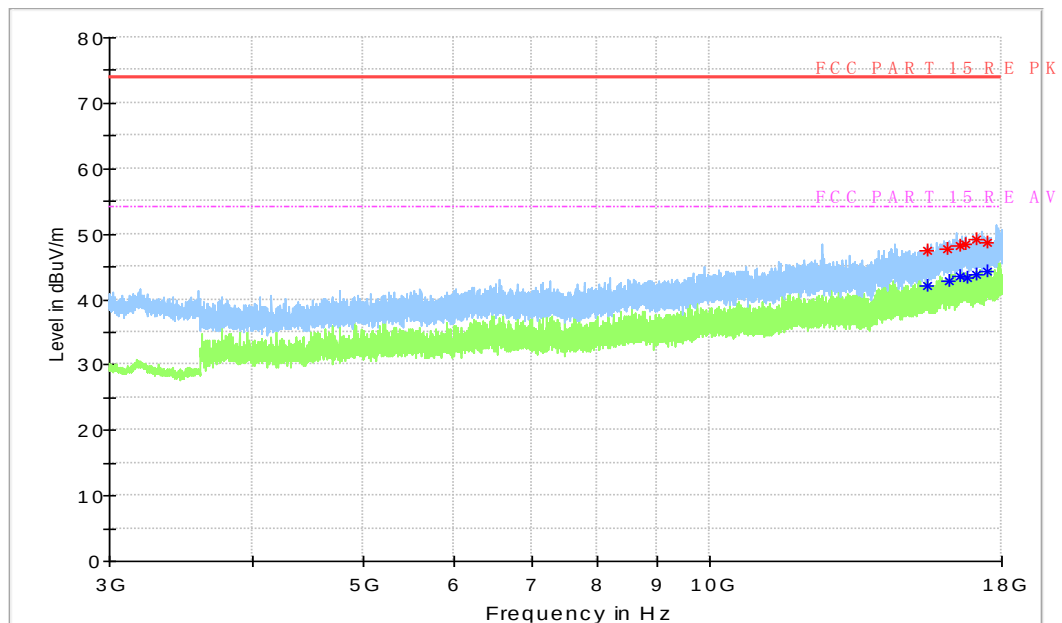
Figure A.66 Radiated Emission from 3GHz to 18GHz
