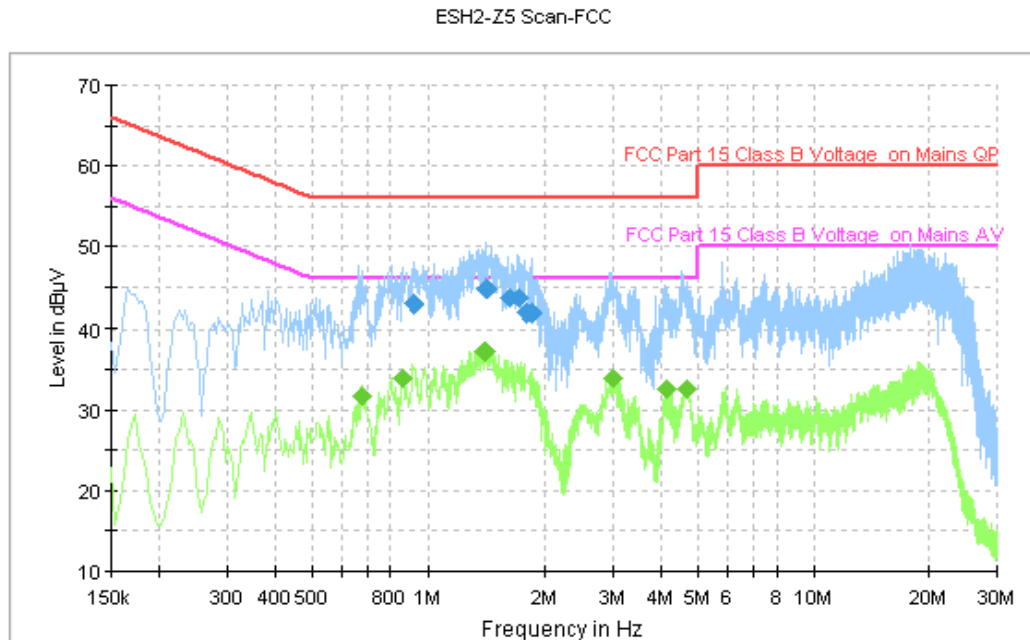
Figure A.105 Conducted Emission
