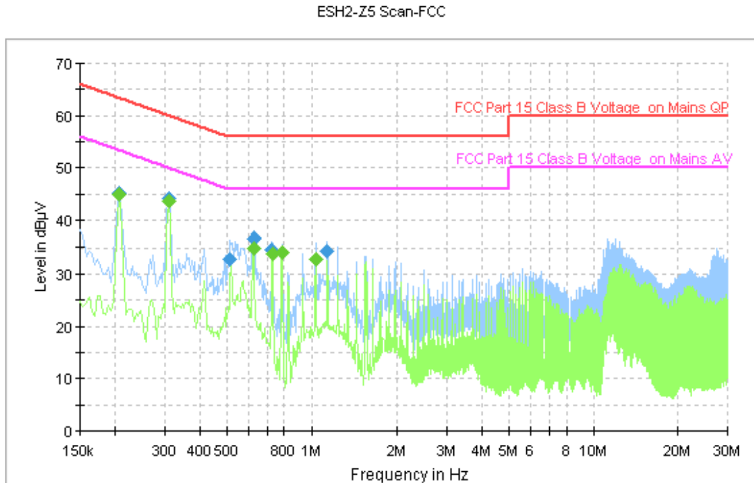
Figure A.149 Conducted Emission
