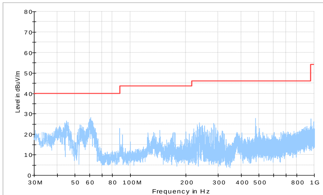
Figure A.73 Radiated Emission from 30MHz to 1GHz
