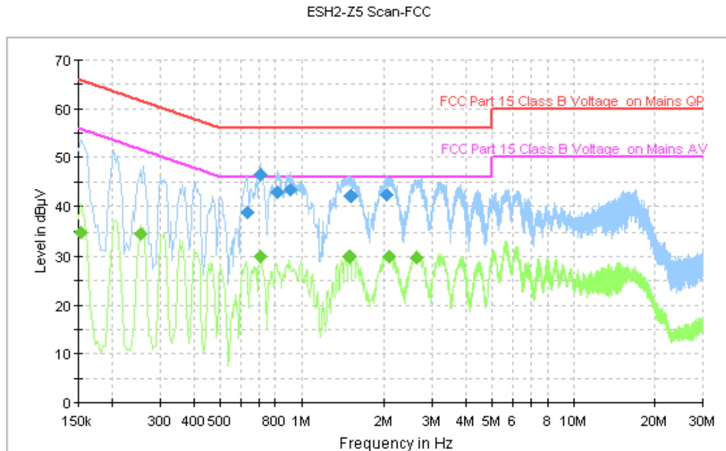
Figure A.100 Conducted Emission
