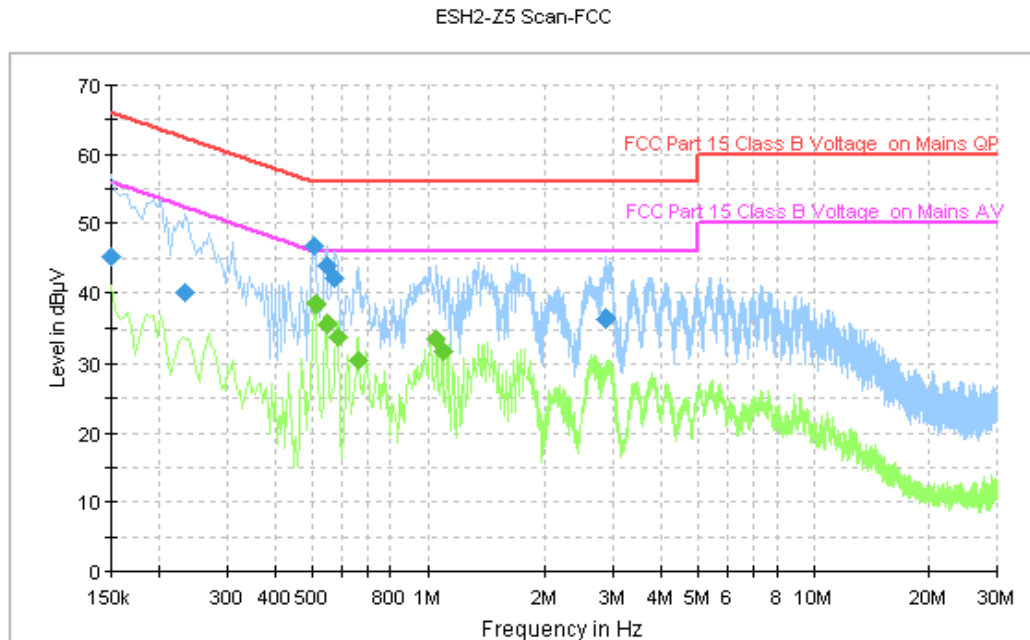
Figure A.102 Conducted Emission
