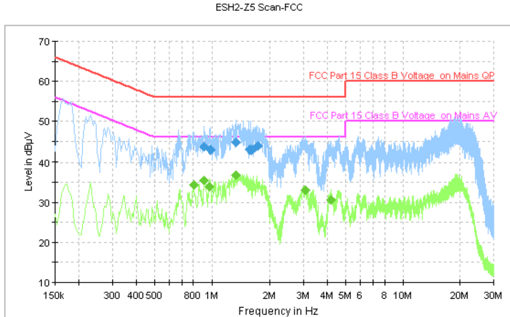
Figure A.106 Conducted Emission
