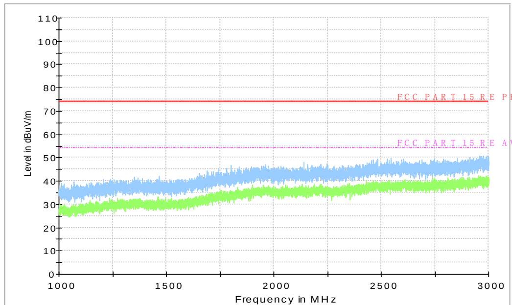
Figure A.80 Radiated Emission from 1Gz to 3GHz
