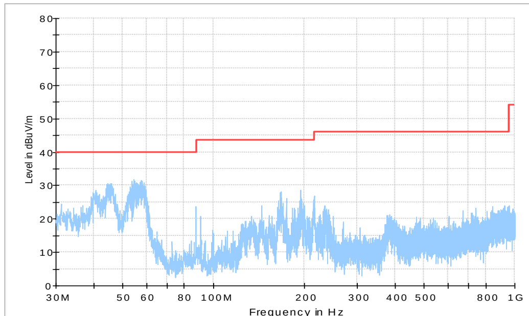
Figure A.76 Radiated Emission from 30MHz to 1GHz
