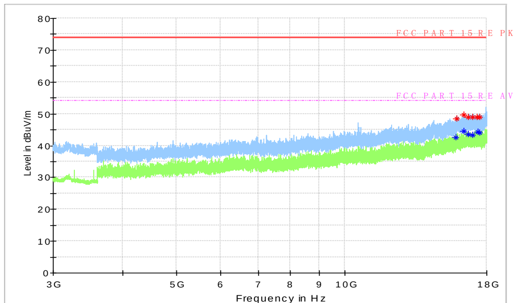
Figure A.75 Radiated Emission from 3GHz to 18GHz
