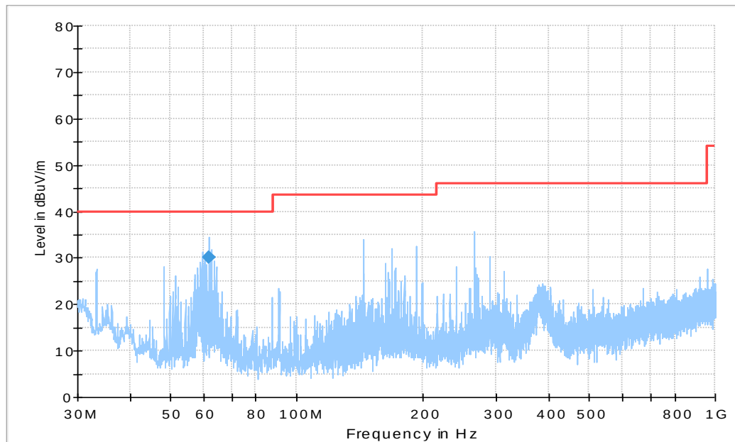
Figure A.61 Radiated Emission from 30MHz to 1GHz
