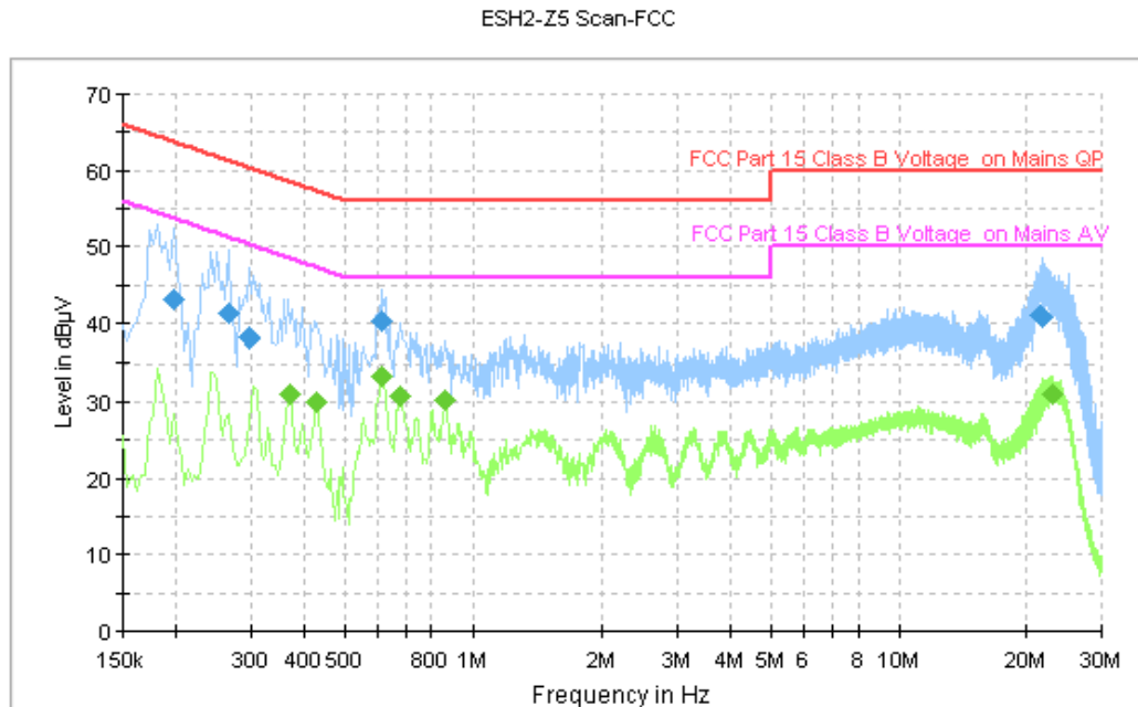
Figure A.96 Conducted Emission
