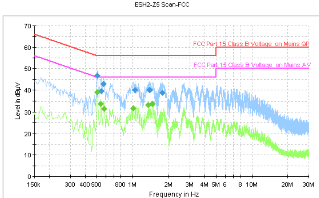
Figure A.101 Conducted Emission
