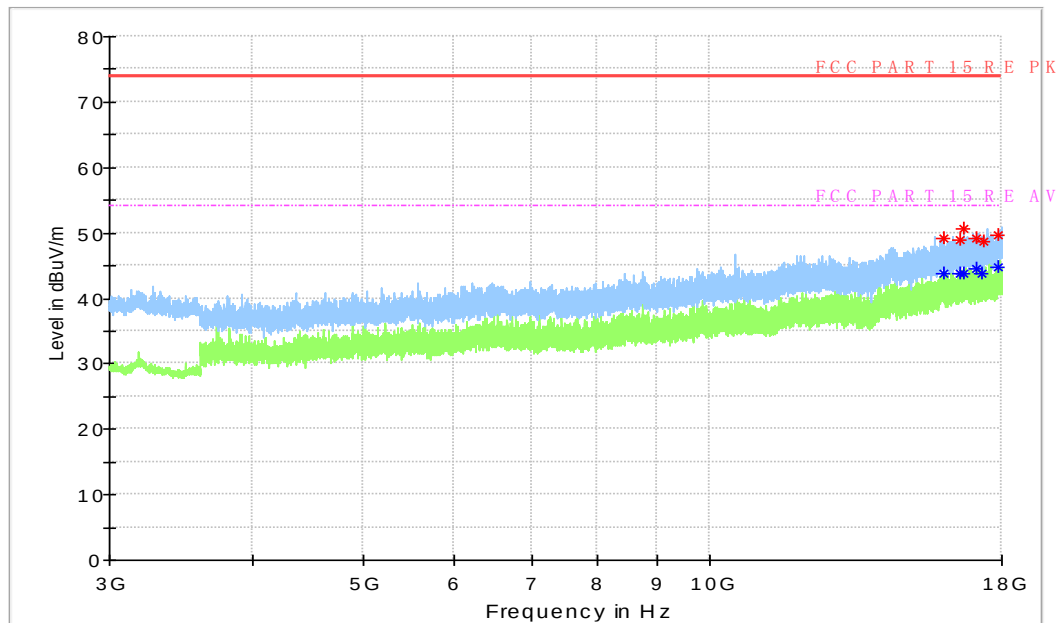
Figure A.84 Radiated Emission from 3GHz to 18GHz
