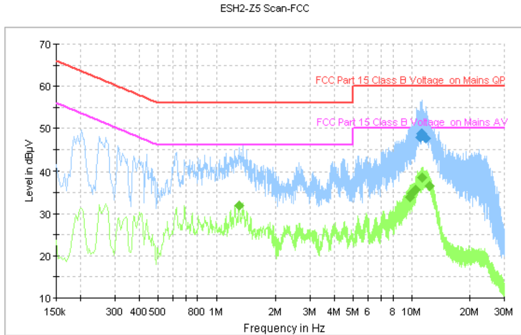
Figure A.103 Conducted Emission
