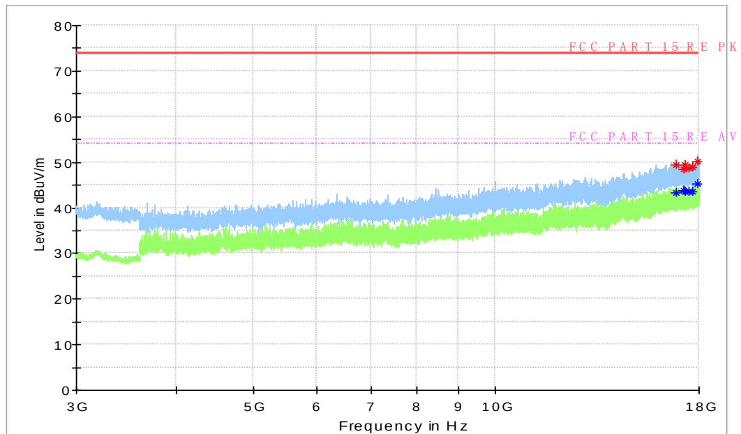
Figure A.90 Radiated Emission from 3GHz to 18GHz
