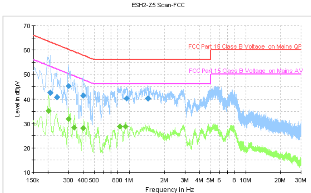
Figure A.122 Conducted Emission
