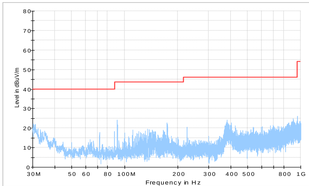
Figure A.79 Radiated Emission from 30MHz to 1GHz
