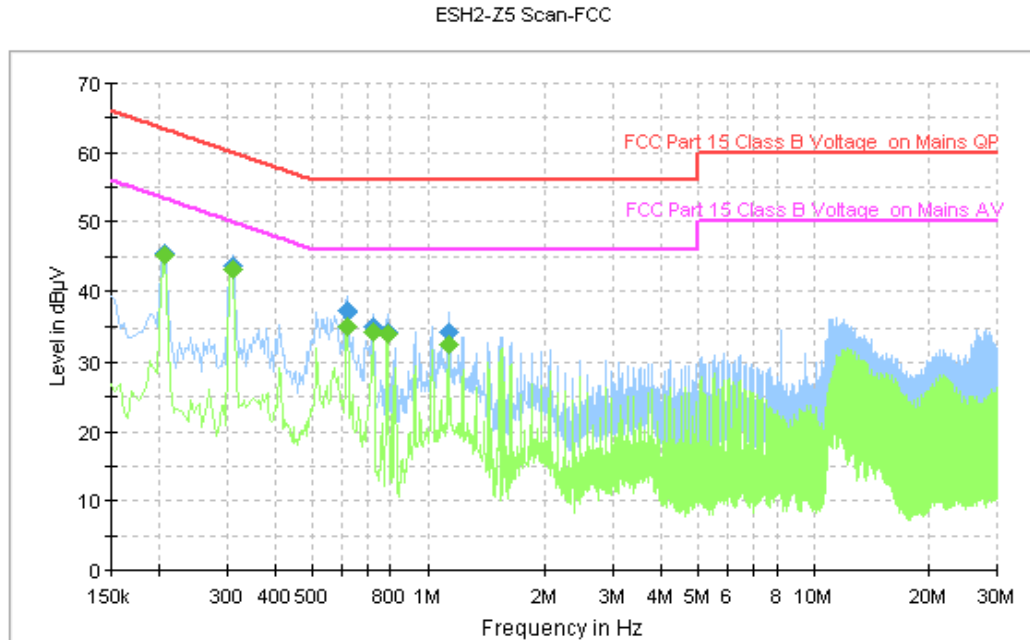
Figure A.140 Conducted Emission
