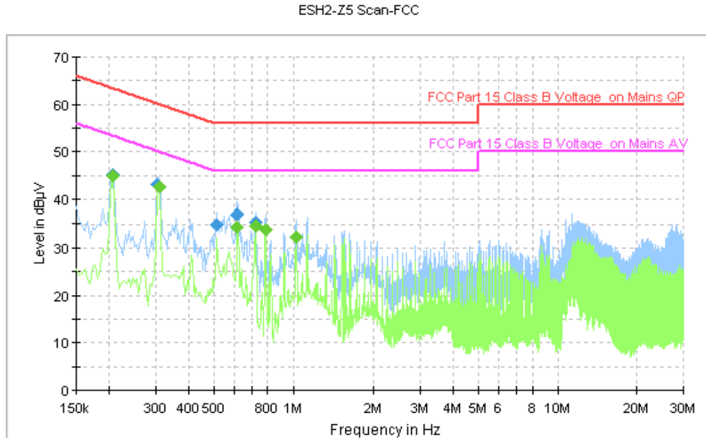
Figure A.138 Conducted Emission
