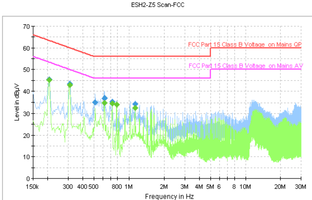
Figure A.136 Conducted Emission
