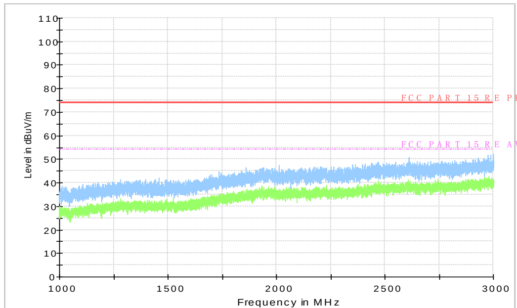
Figure A.86 Radiated Emission from 1Gz to 3GHz
