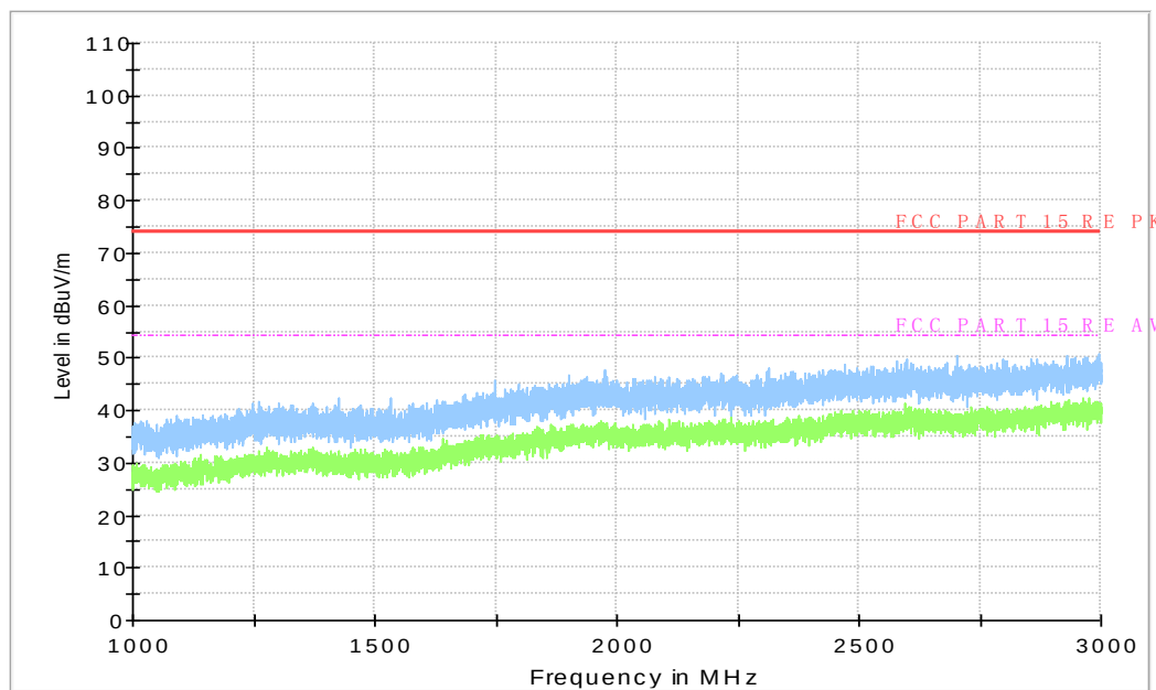
Figure A.77 Radiated Emission from 1Gz to 3GHz
