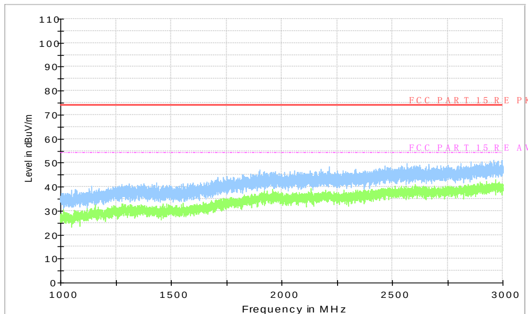
Figure A.89 Radiated Emission from 1Gz to 3GHz
