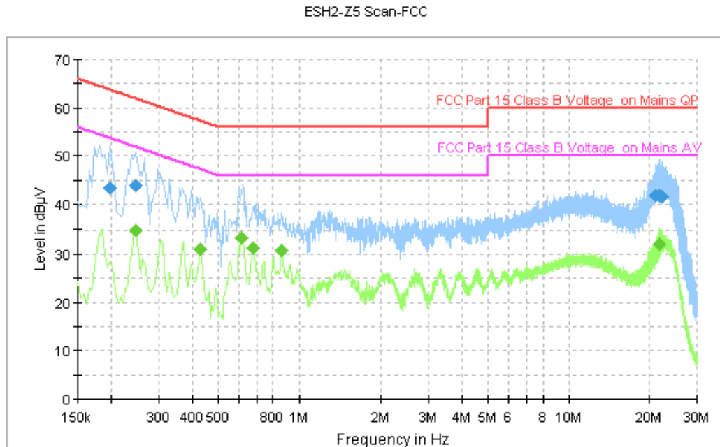
Figure A.120 Conducted Emission
