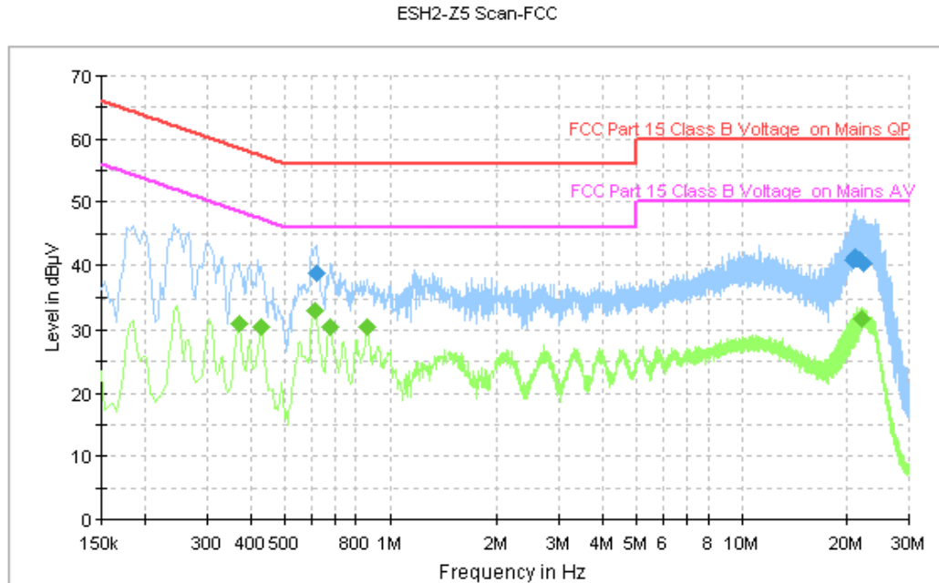
Figure A.107 Conducted Emission
