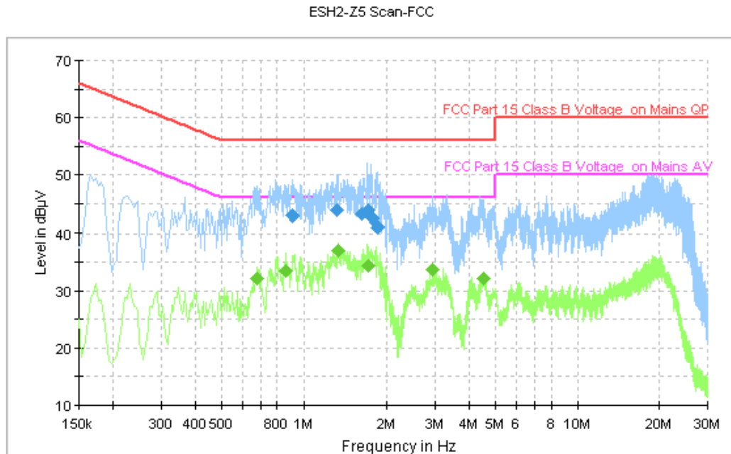
Figure A.94 Conducted Emission
