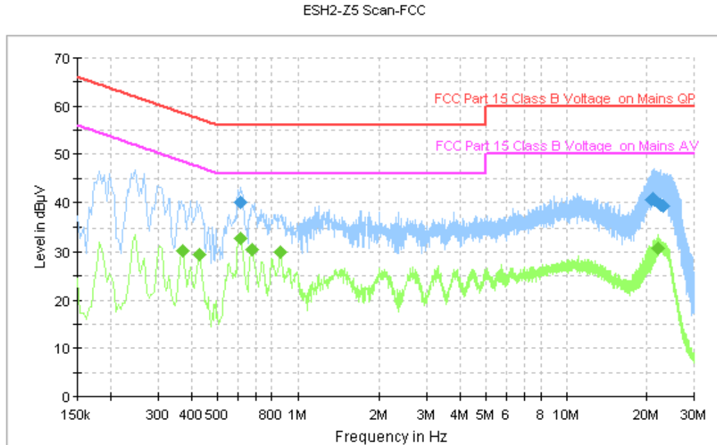
Figure A.95 Conducted Emission
