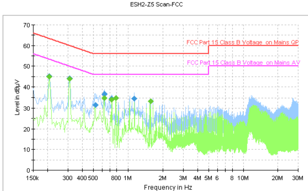
Figure A.141 Conducted Emission
