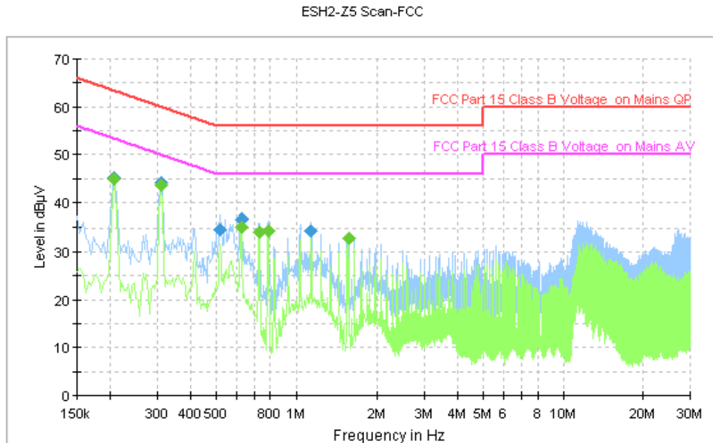
Figure A.145 Conducted Emission
