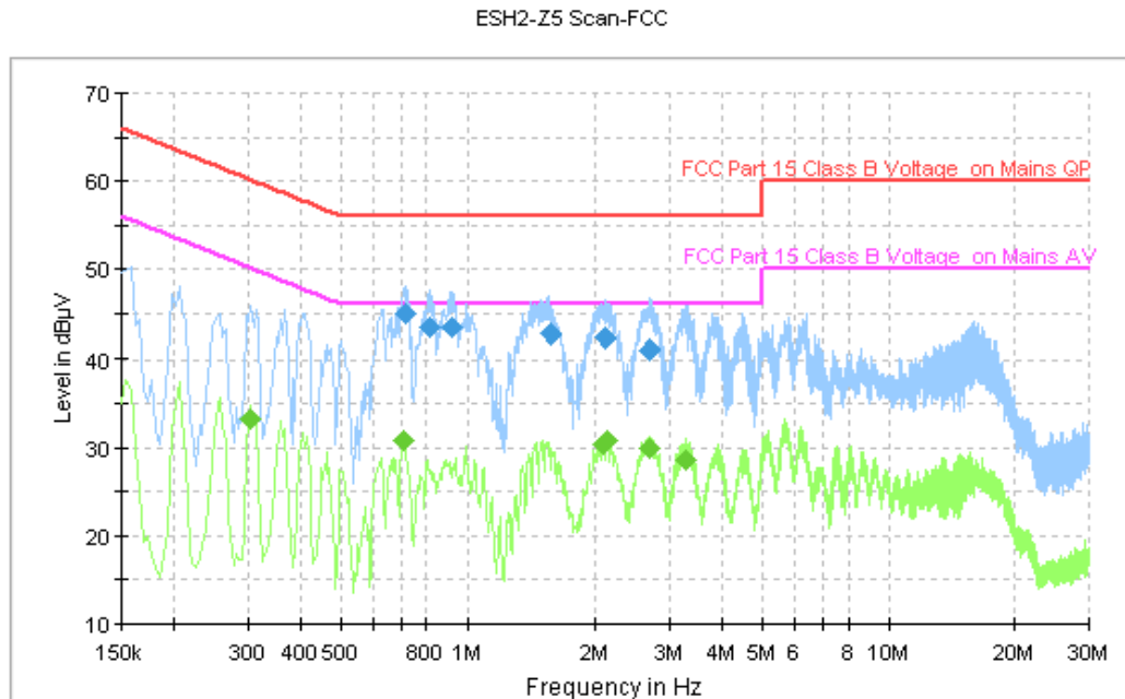
Figure A.112 Conducted Emission
