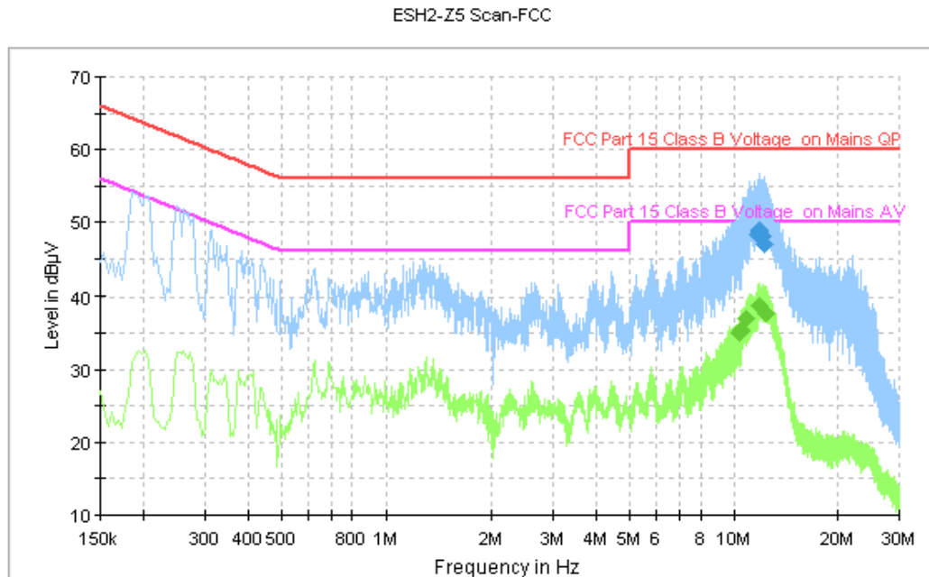
Figure A.104 Conducted Emission
