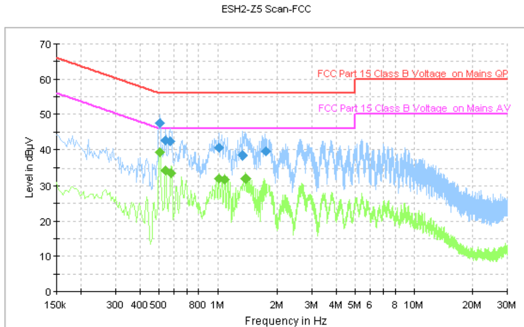
Figure A.125 Conducted Emission
