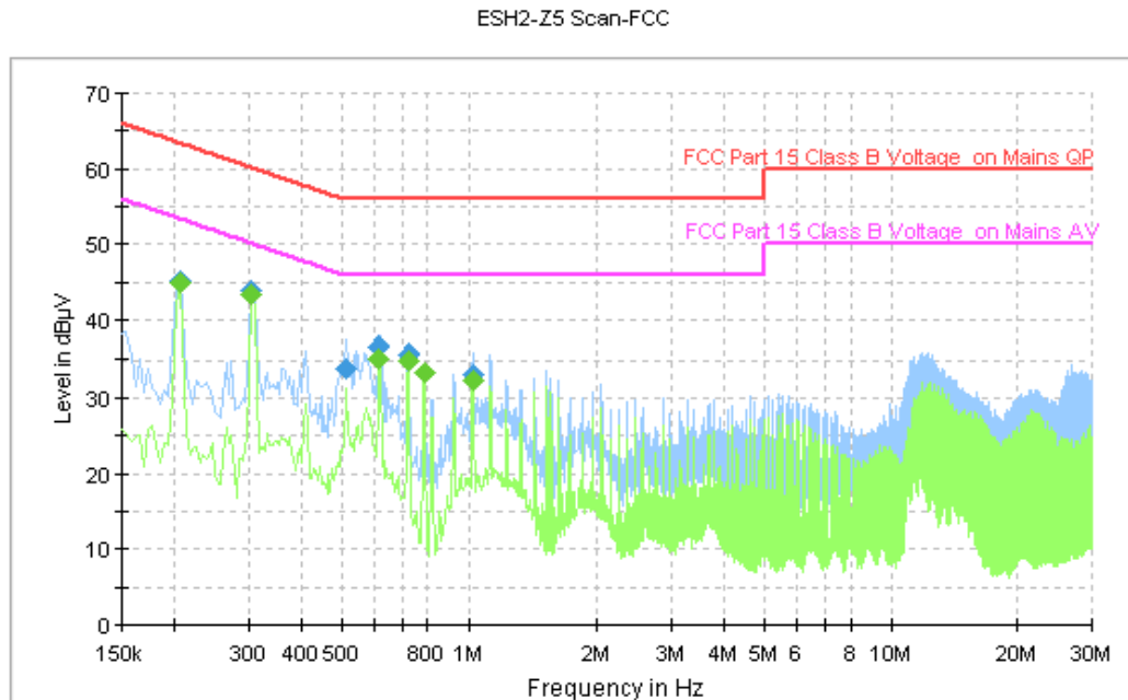
Figure A.134 Conducted Emission
