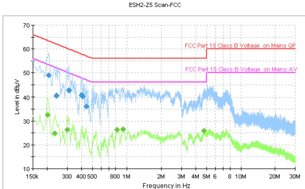
Figure A.110 Conducted Emission
