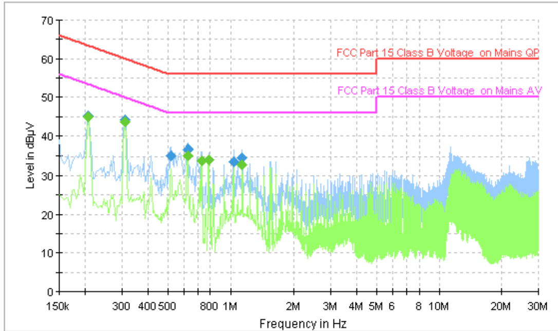
Figure A.147 Conducted Emission
