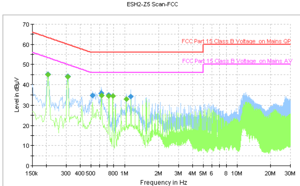
Figure A.139 Conducted Emission
