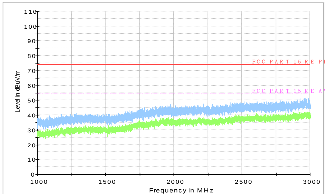
Figure A.74 Radiated Emission from 1Gz to 3GHz
