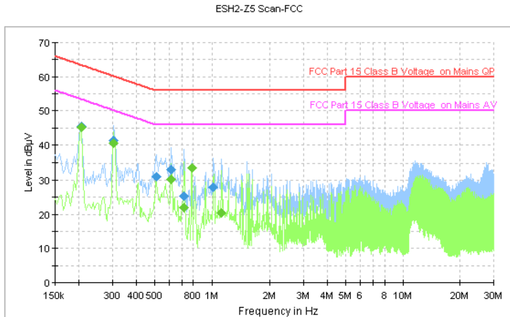
Figure A.143 Conducted Emission
