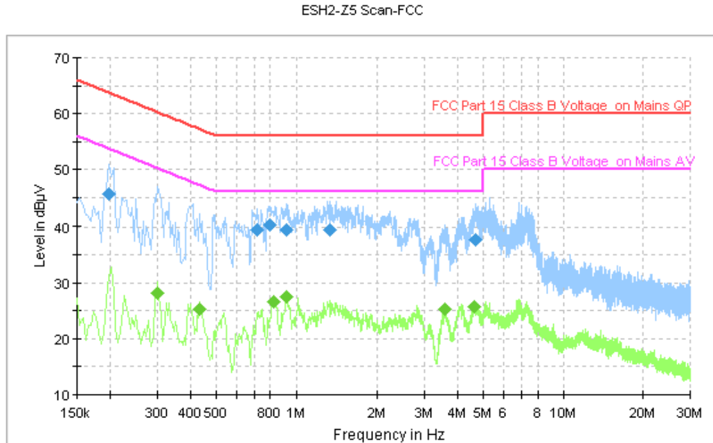
Figure A.109 Conducted Emission
