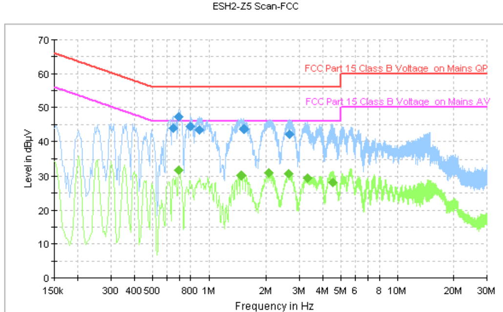
Figure A.123 Conducted Emission
