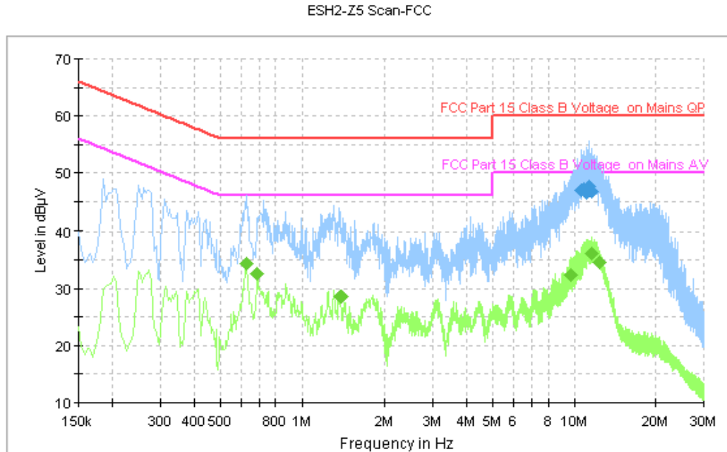
Figure A.115 Conducted Emission
