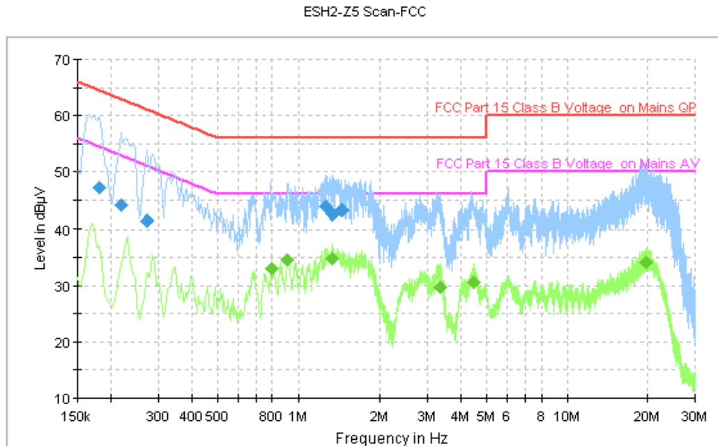
Figure A.93 Conducted Emission
