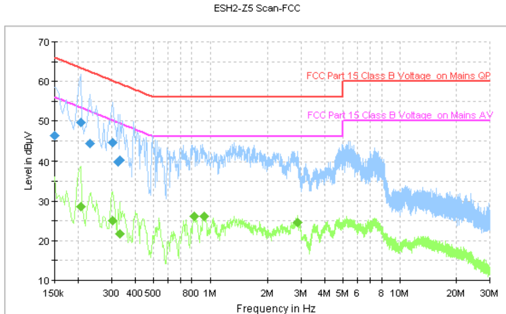
Figure A.98 Conducted Emission
