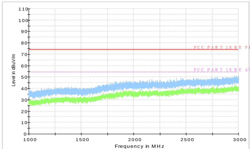
Figure A.65 Radiated Emission from 1Gz to 3GHz
