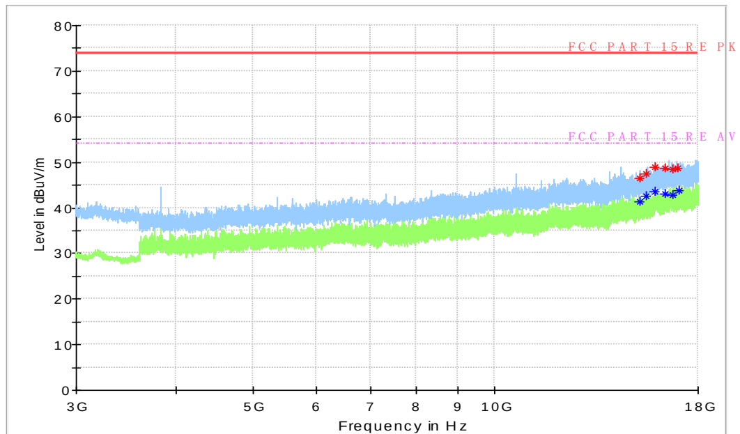
Figure A.63 Radiated Emission from 3GHz to 18GHz
