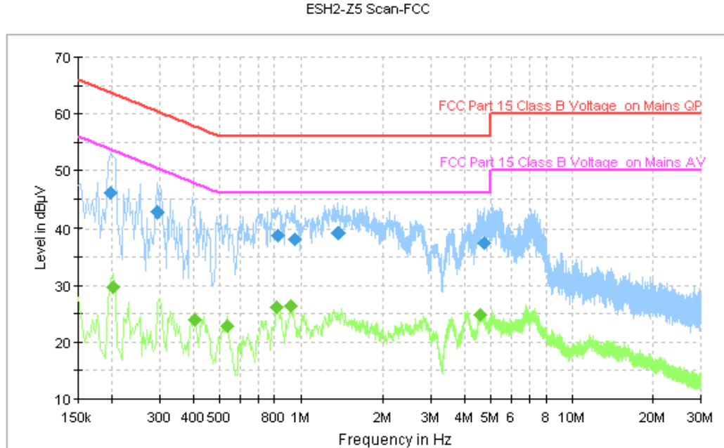
Figure A.97 Conducted Emission
