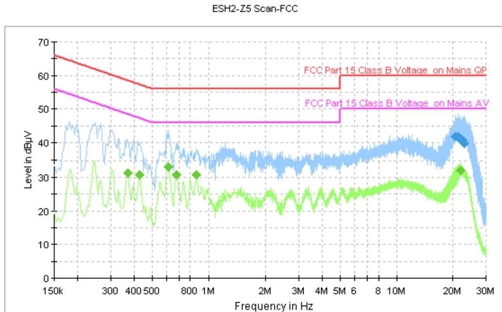
Figure A.119 Conducted Emission
