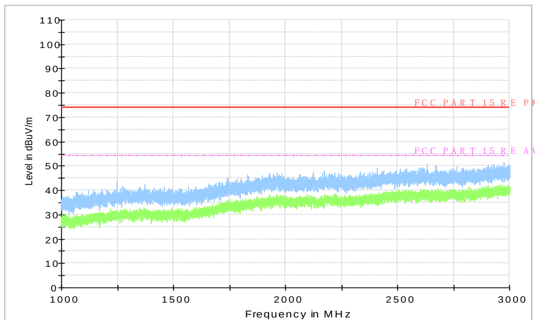
Figure A.83 Radiated Emission from 1Gz to 3GHz
