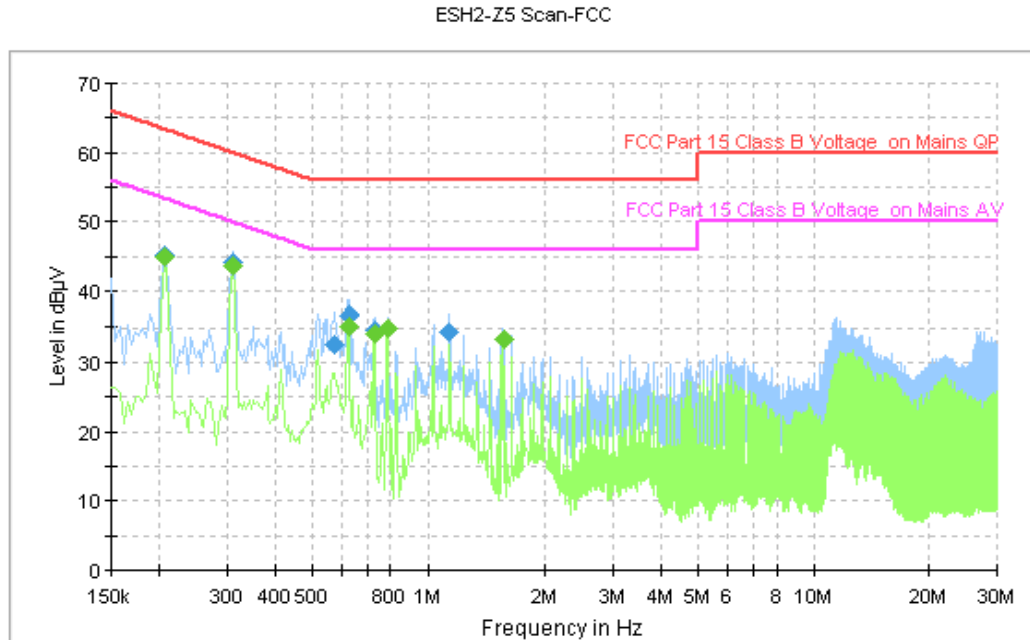
Figure A.127 Conducted Emission
