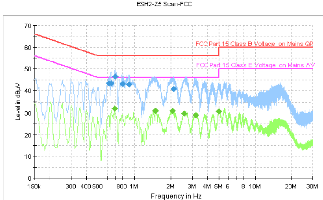
Figure A.99 Conducted Emission
