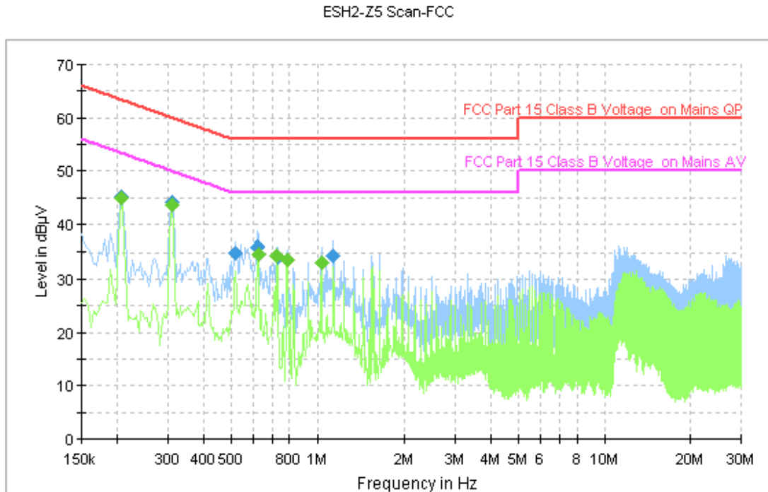
Figure A.148 Conducted Emission
