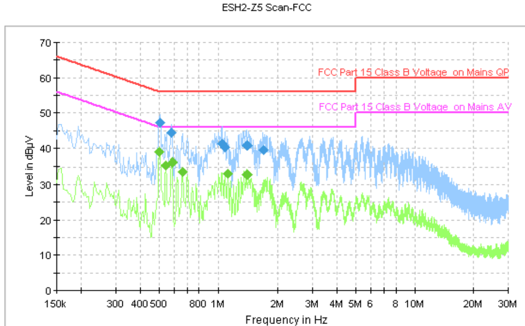
Figure A.126 Conducted Emission
