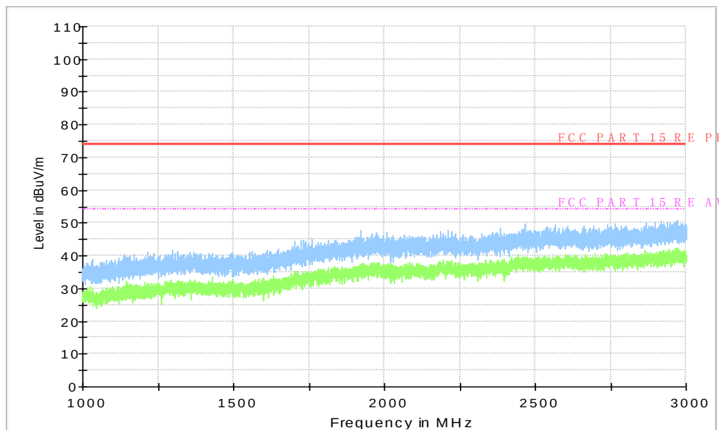
Figure A.62 Radiated Emission from 1Gz to 3GHz
