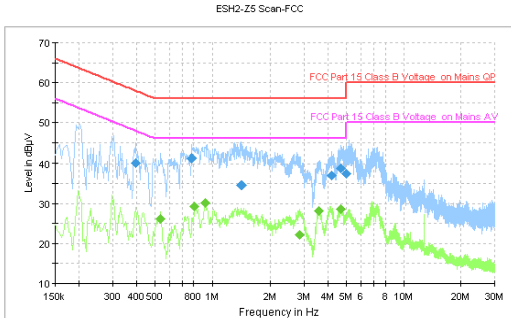
Figure A.121 Conducted Emission
