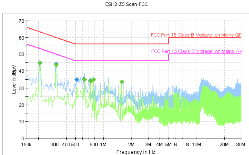
Figure A.131 Conducted Emission
