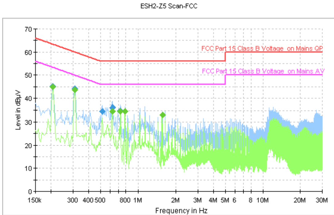
Figure A.137 Conducted Emission
