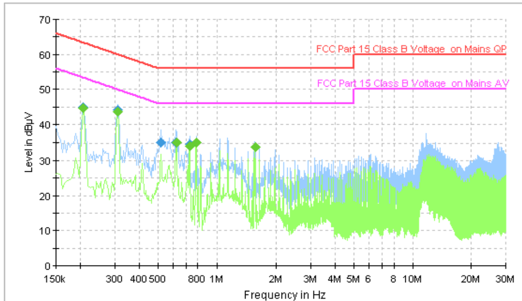
Figure A.133 Conducted Emission
