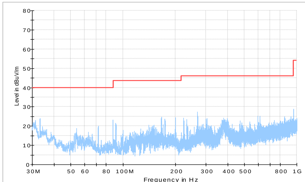
Figure A.82 Radiated Emission from 30MHz to 1GHz
