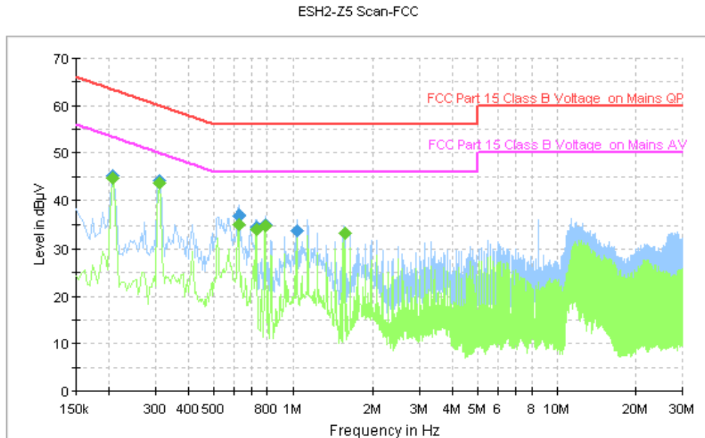
Figure A.129 Conducted Emission
