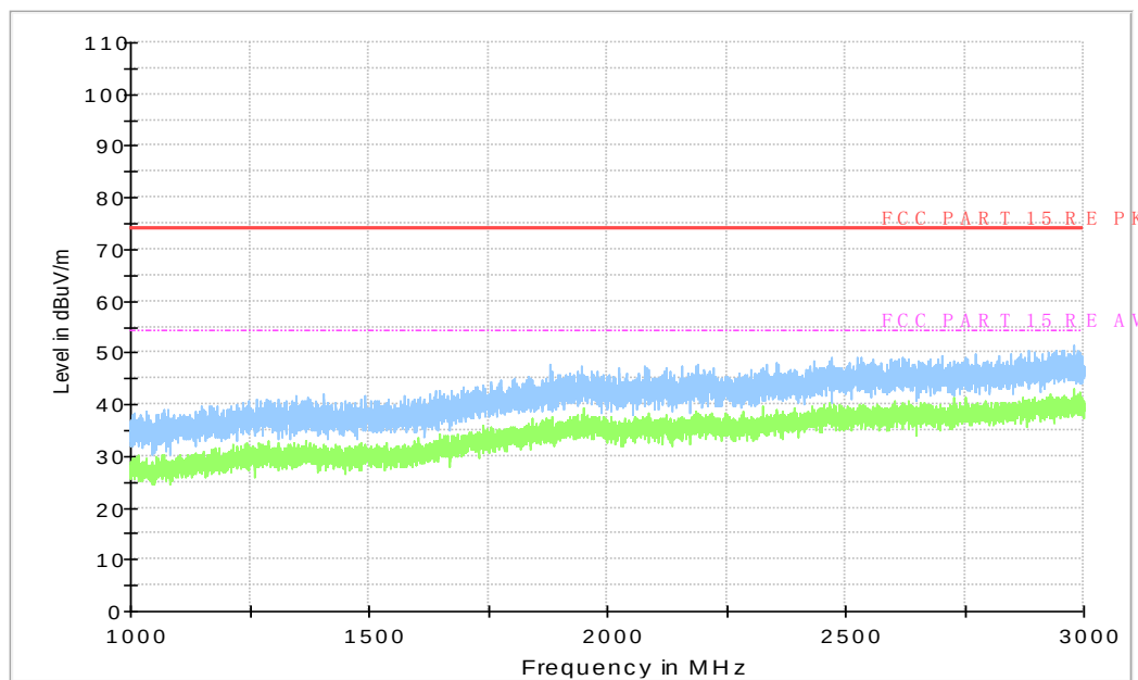
Figure A.68 Radiated Emission from 1Gz to 3GHz
