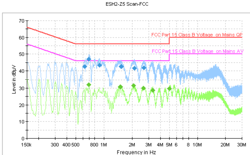
Figure A.111 Conducted Emission
