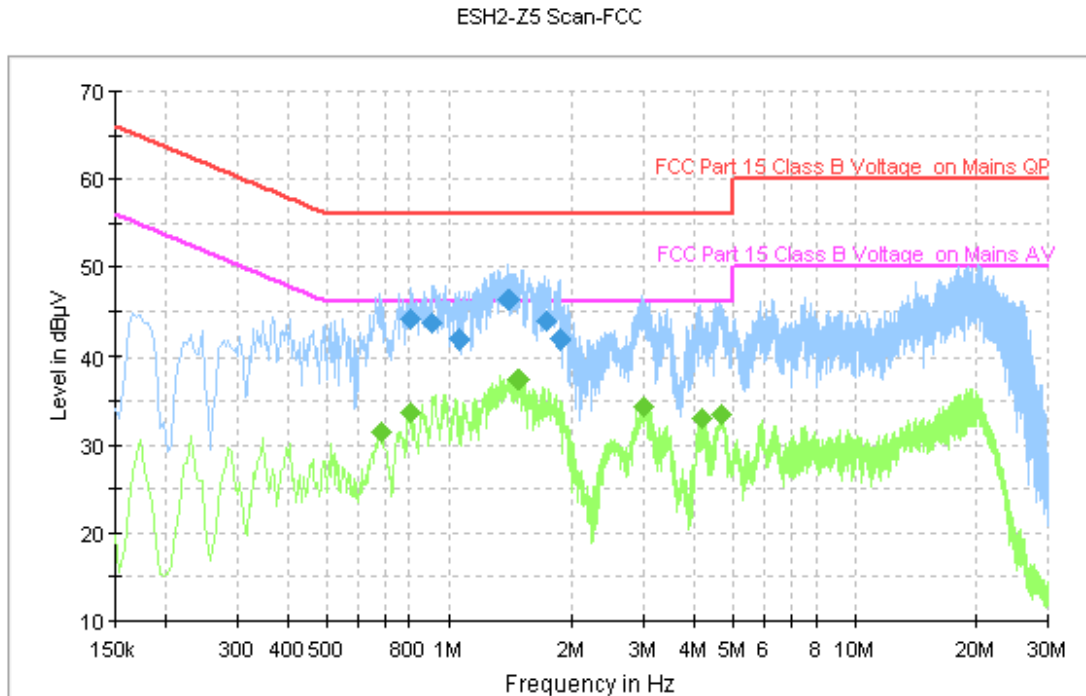
Figure A.117 Conducted Emission
