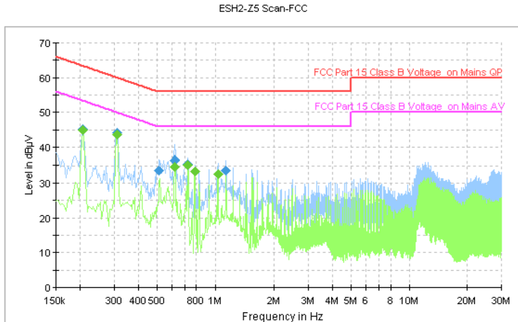
Figure A.144 Conducted Emission
