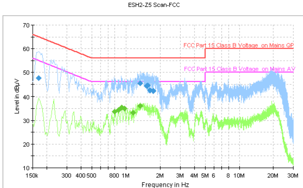
Figure A.118 Conducted Emission
