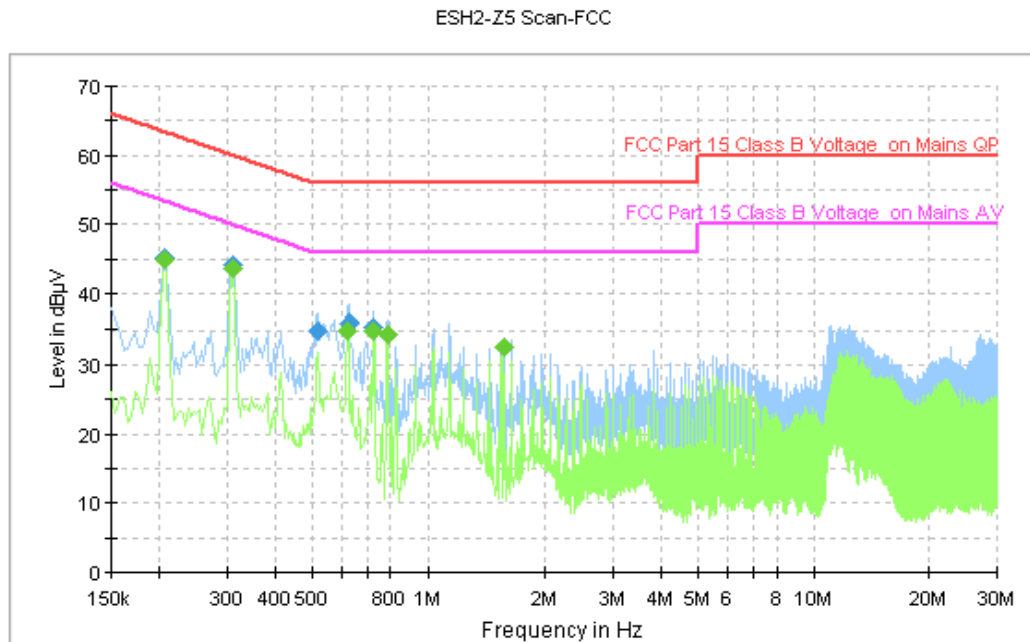
Figure A.135 Conducted Emission
