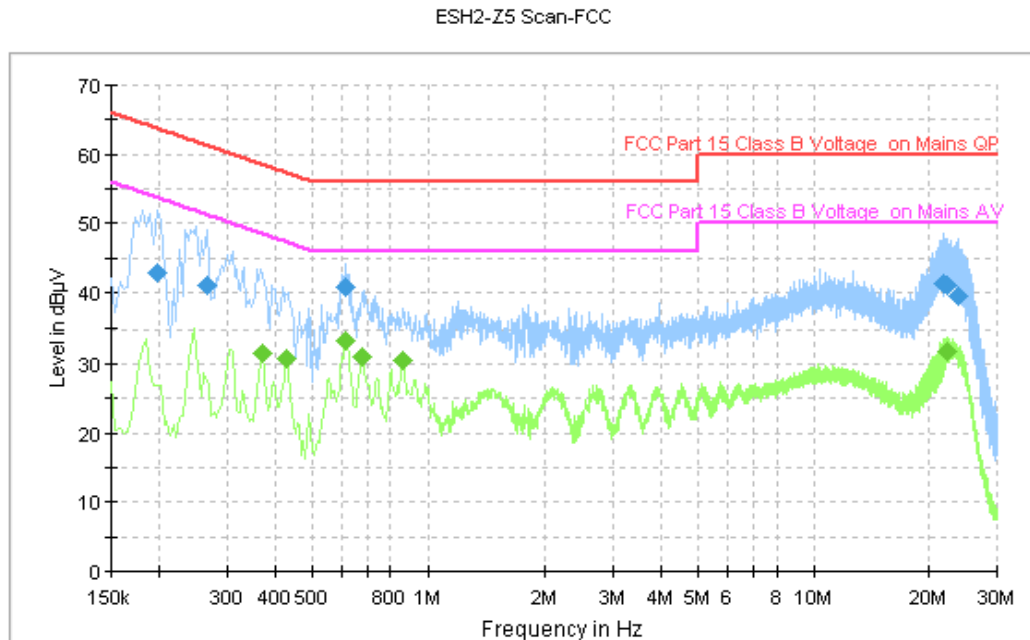
Figure A.108 Conducted Emission
