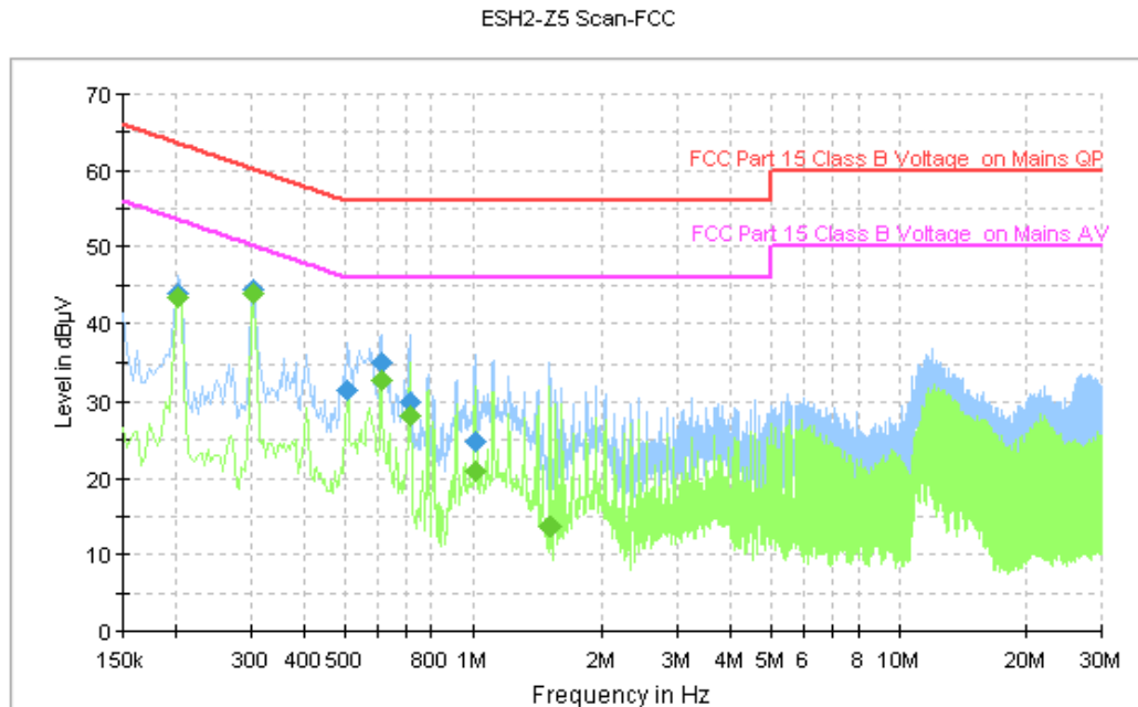
Figure A.128 Conducted Emission
