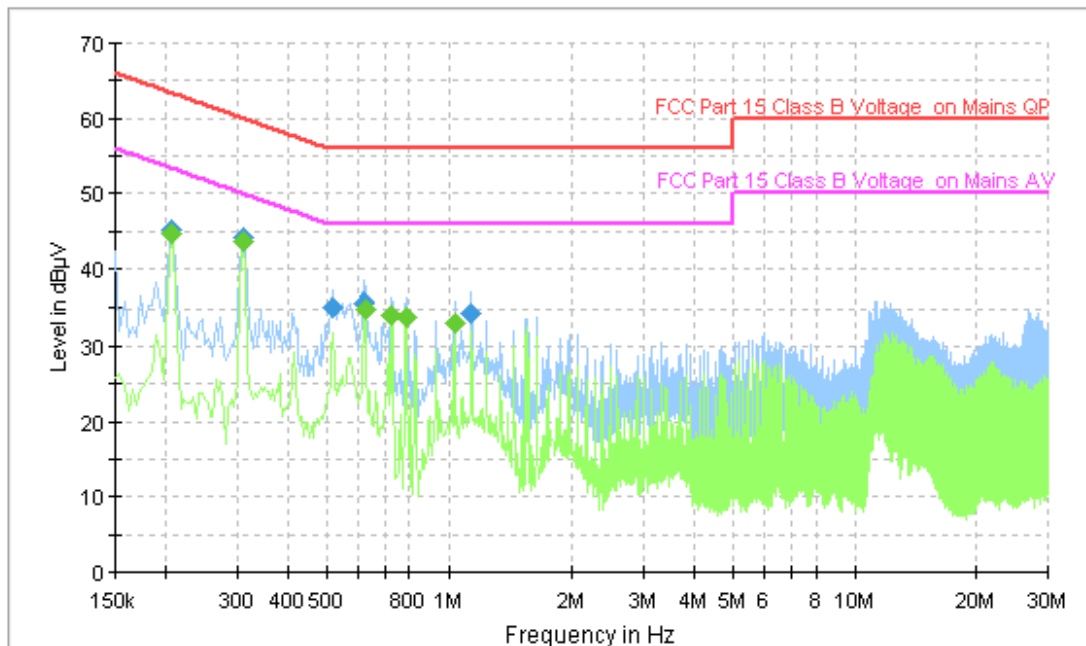
Figure A.150 Conducted Emission
