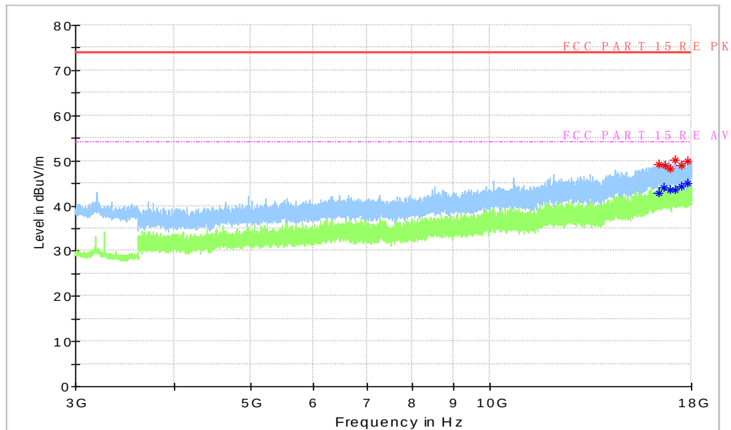
Figure A.69 Radiated Emission from 3GHz to 18GHz
