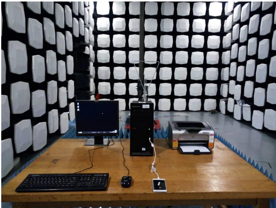
2. Radiated Emissions (Part 15B PC mode)( 1GHz-3GHz)
