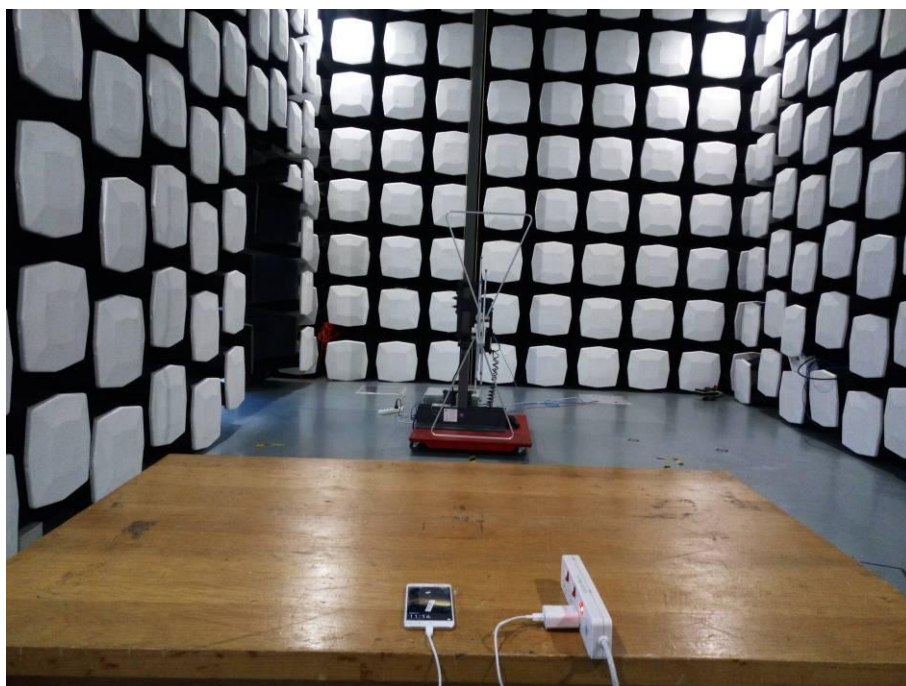
4. Radiated Emissions (Part 15B Charging mode) (below 1GHz)
