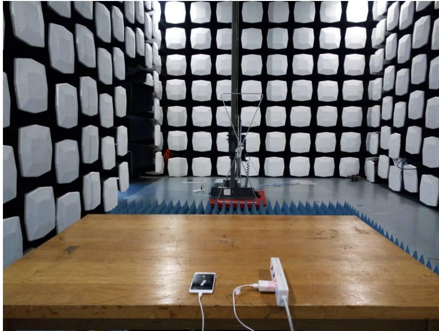
5. Radiated Emissions (Part 15B Charging mode) (1GHz-3GHz)
