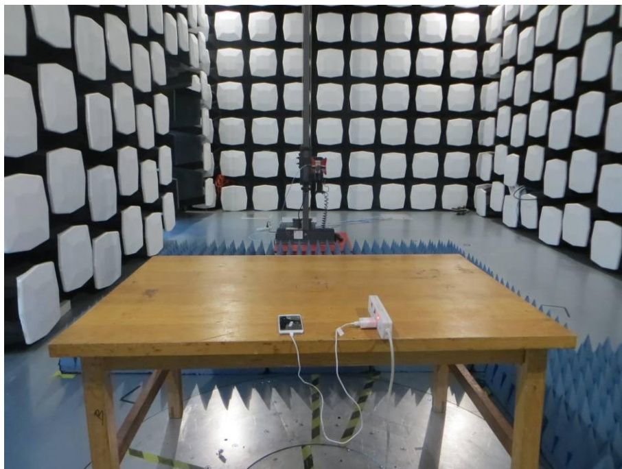
6. Radiated Emissions (Part 15B Charging mode) (3GHz-18GHz)
