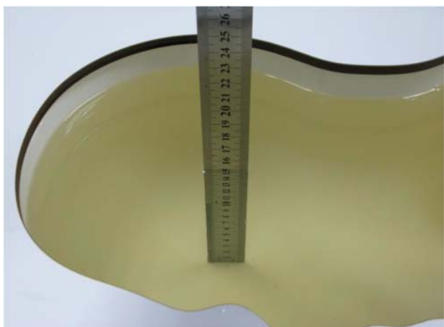
Photo 27: HSL2600MHz depth (15.0cm)
