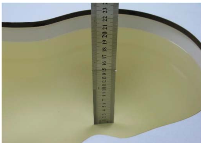
Photo 25: HSL2450MHz depth (15.0cm)
