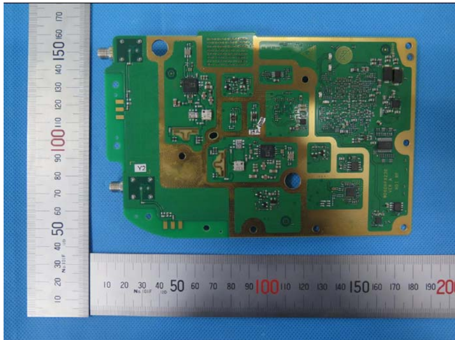
EUT –Rear of WD6DLPX2T0(UMTS, LTE band 5) View
