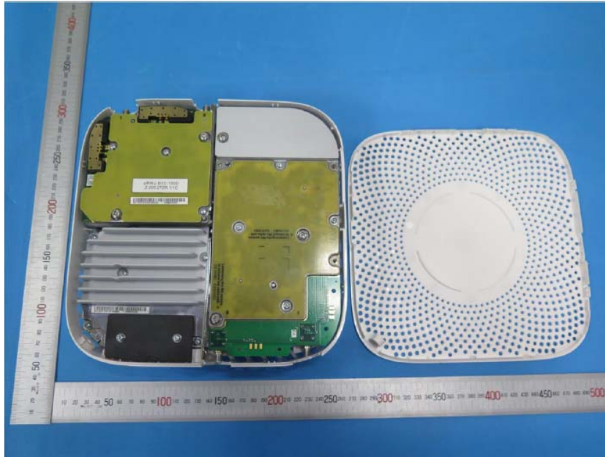
EUT –Heads of WD6DIPX220(UMTS Band 2, LTE Band 2, UMTS&LTE Band2) View
