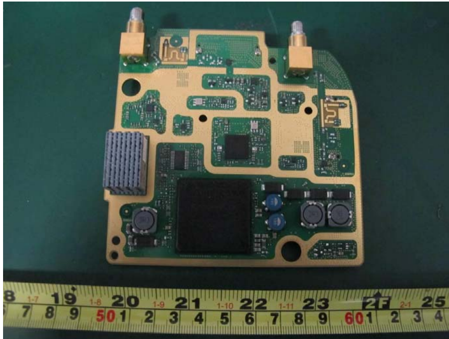
EUT –Rear of WD6DIPX220(UMTS Band 2, LTE Band 2, UMTS&LTE Band2) View
