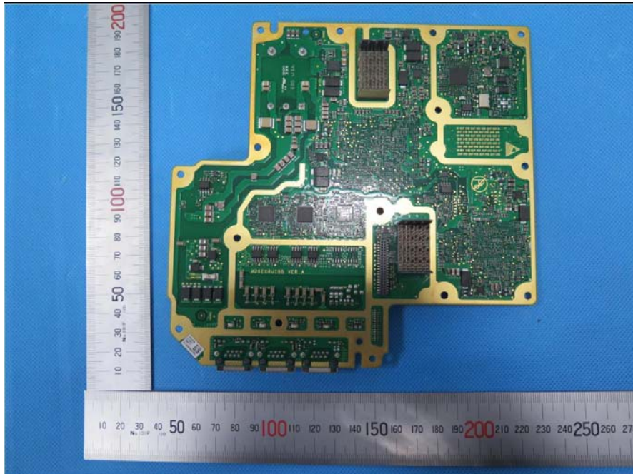
EUT –Rear of WD6EXRUIBD View
