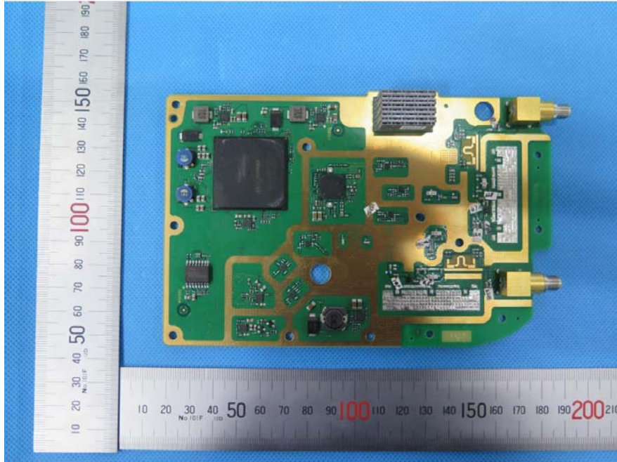
EUT –Heads of WD6DLPX2T0(UMTS, LTE band 5) View
