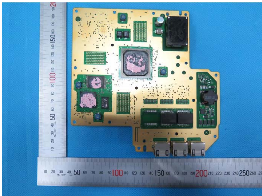
EUT –Heads of WD6EXRUIBD View
