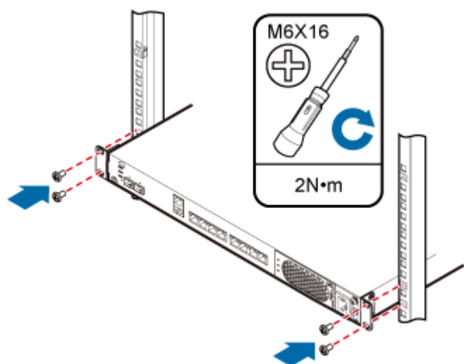
Figure 6-18 Tightening screws
