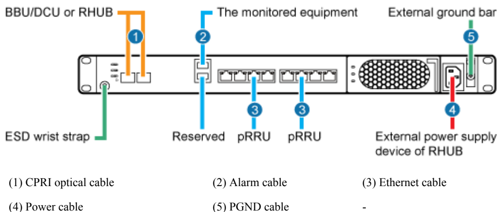
Figure 6-28 Cable connections for an RHUB
