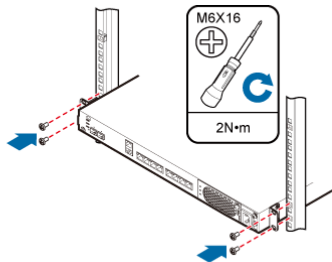
Figure 6-14 Tightening screws
