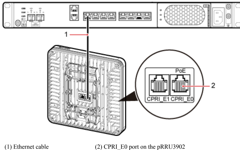
Figure 8-38 Installing an Ethernet cable
