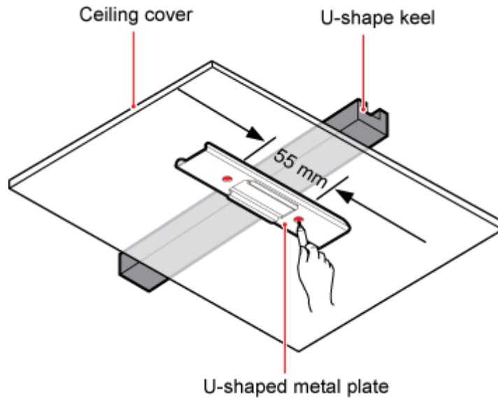
Figure 8-26 Anchor points on the suspended ceiling plate
