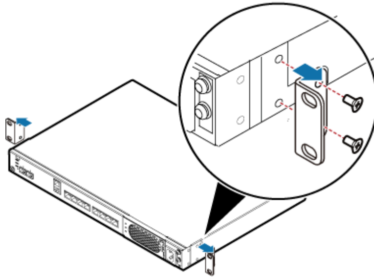
Figure 6-20 Removing mounting ears and screws
