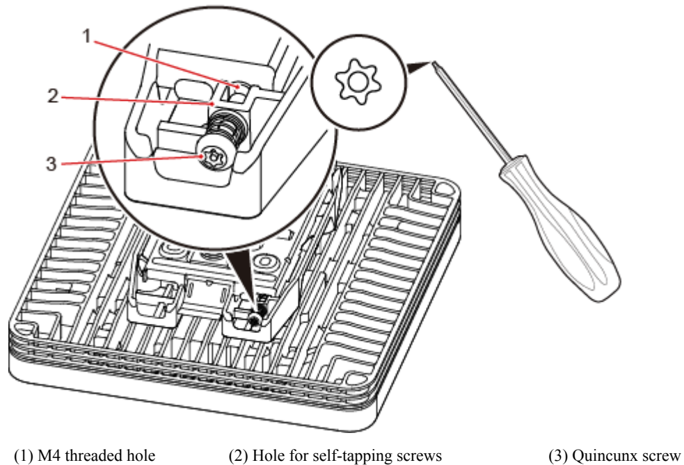
Figure 8-29 Locking the protection screw
