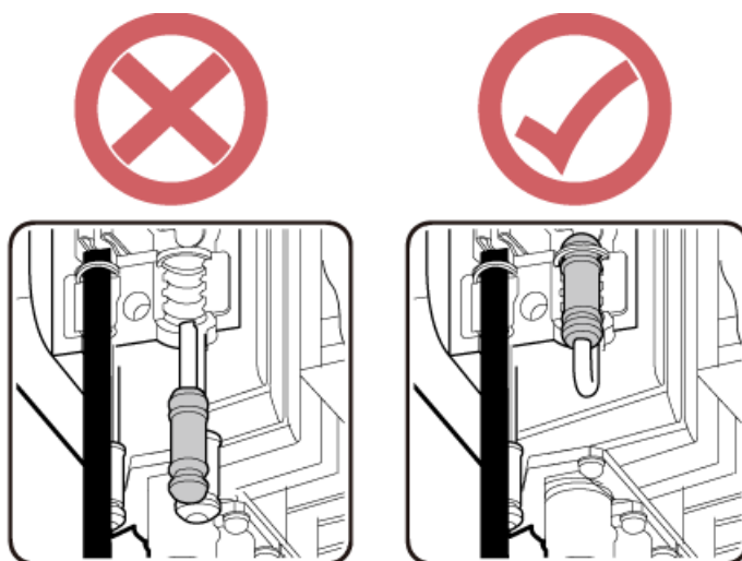
Figure 9-23 Correct placement of waterproof blocks
