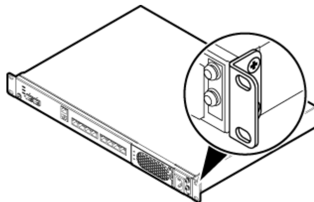
Figure 6-16 Installing mounting ears in standard mode
