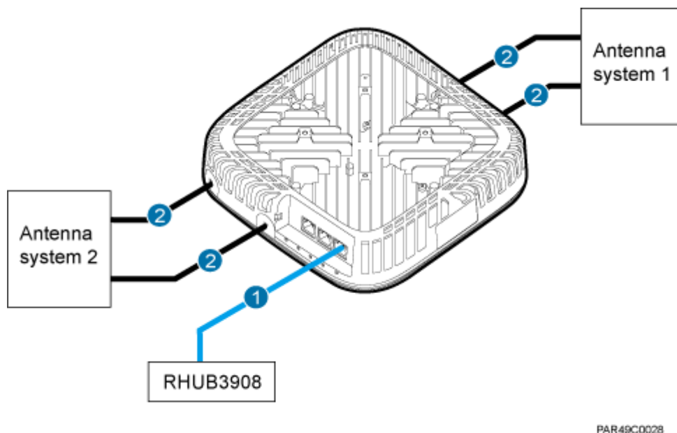
Figure 7-24 pRRU3901 cable connection (2)
