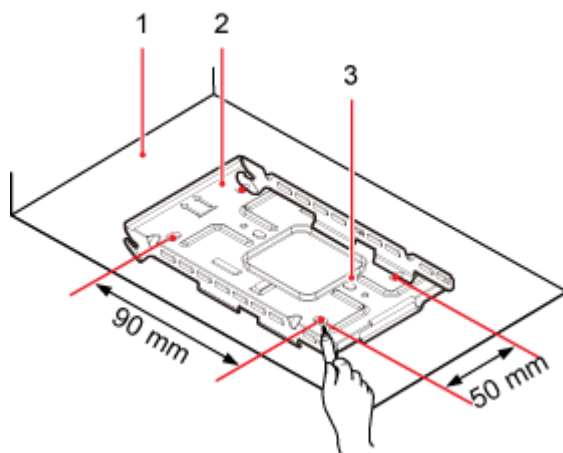
Figure 8-11 Anchor points on the pRRU3902 mounting bracket
