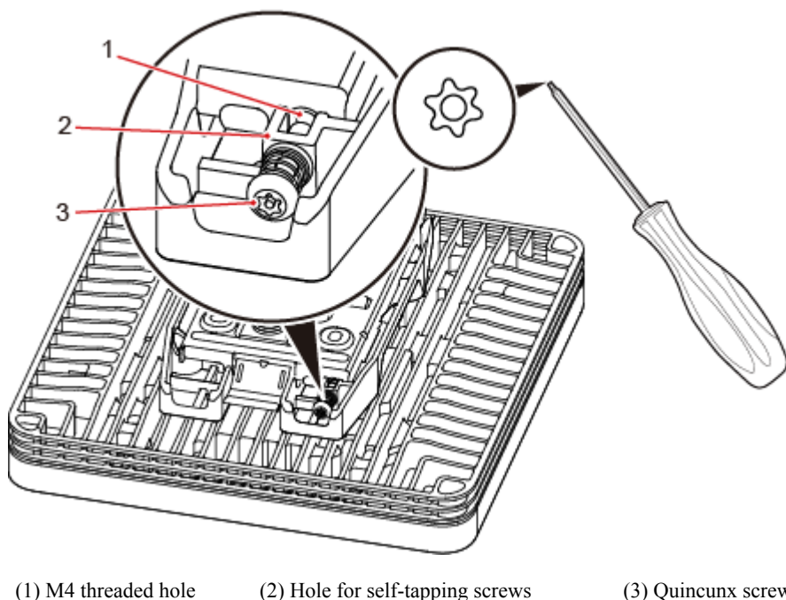
Figure 8-25 Locking the protection screw
