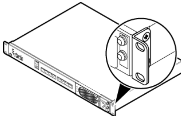
Figure 6-21 Installing mounting ears in standard mode
