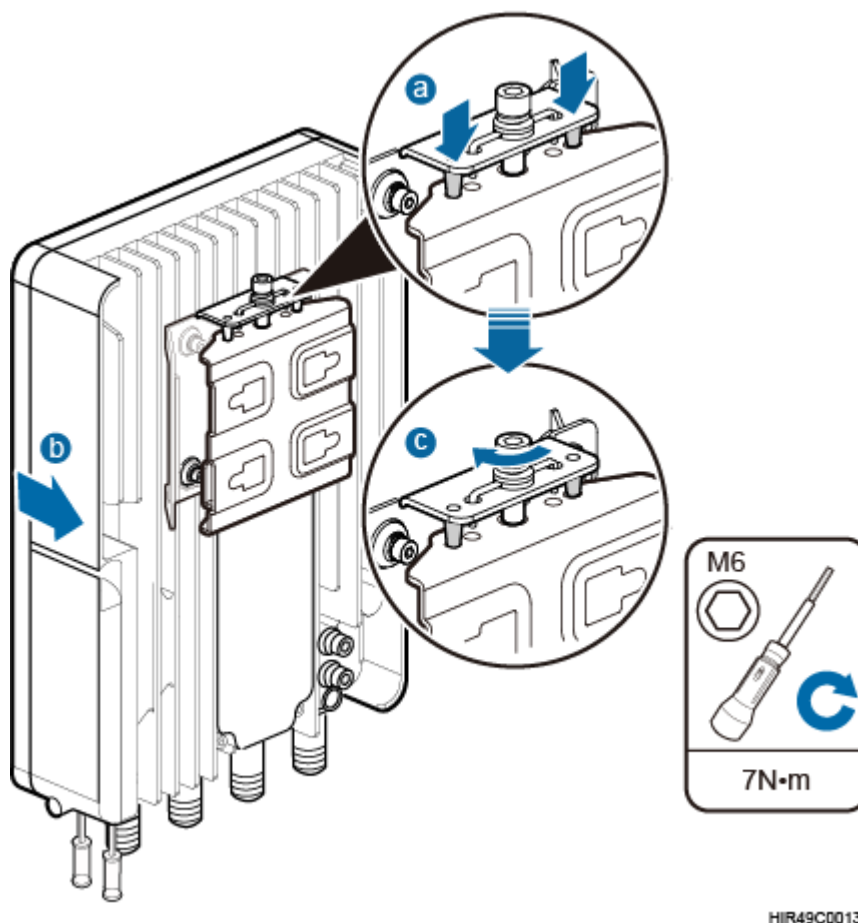
Figure 9-13 Securing the pRRU onto the mounting kit
