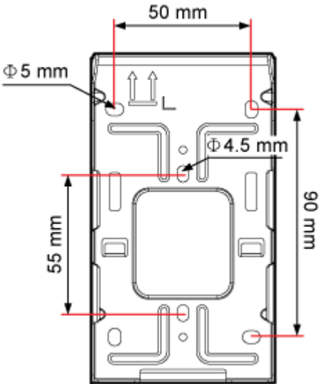
Figure 8-4 Mounting bracket specifications
