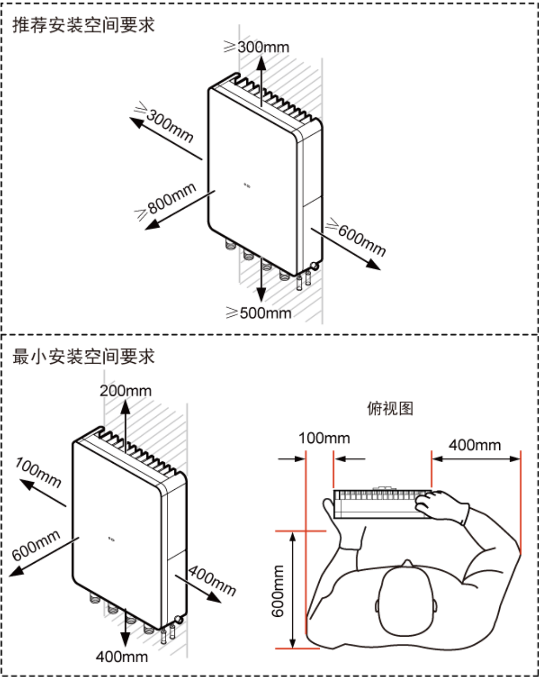
Figure 9-3 Clearances for installing a pRRU3907
