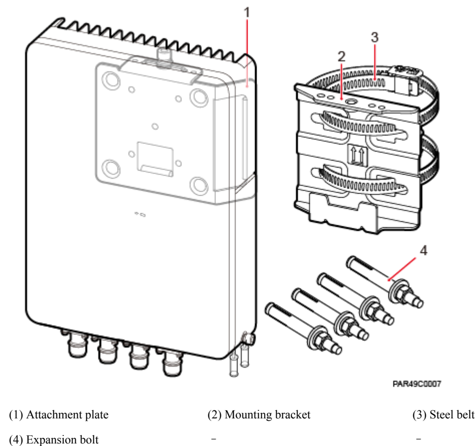
Figure 9-6 Mounting bracket and common attachment plate for installing a pRRU
