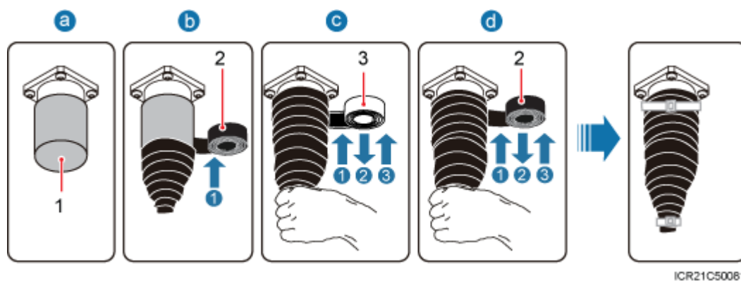
Figure 9-20 Waterproofing a dustproof cap
