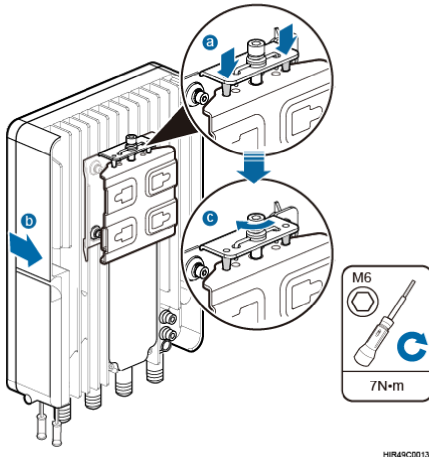
Figure 9-10 Securing the pRRU onto the mounting kit
