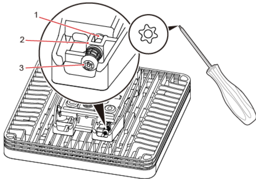
Figure 8-19 Locking the protection screw
