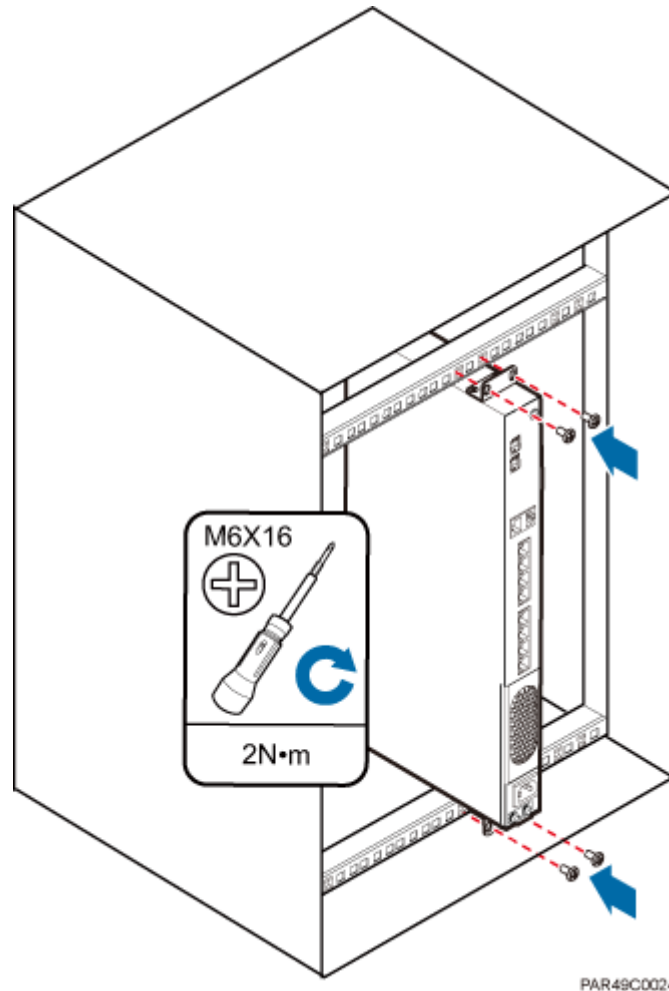
Figure 6-19 Tightening screws
