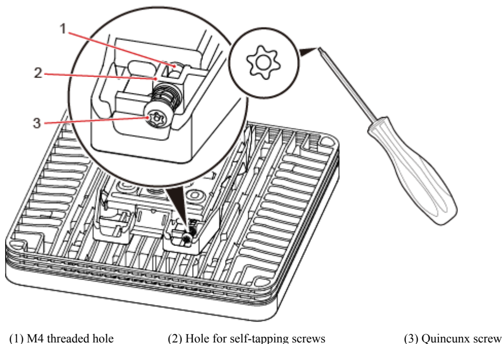
Figure 8-15 Locking the protection screw
