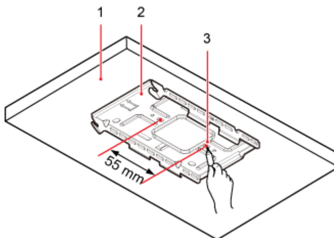
Figure 8-16 Anchor points on the pRRU3902 mounting bracket
