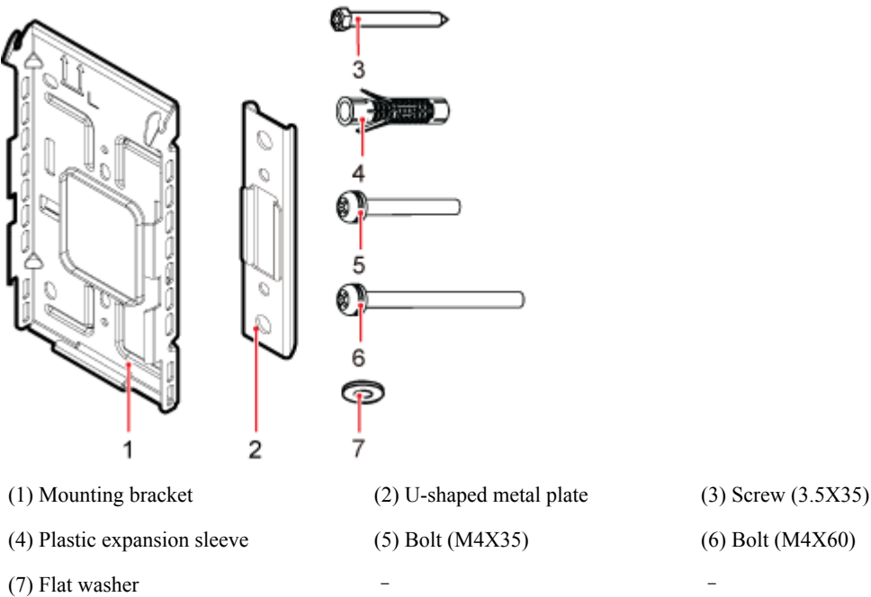
Figure 8-3 pRRU3902 mounting kits
