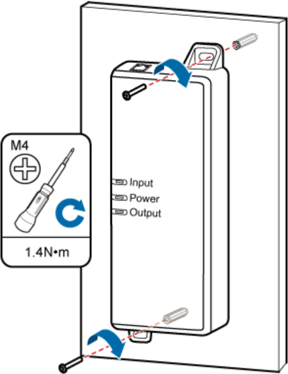
Figure 10-3 Installing Extender
