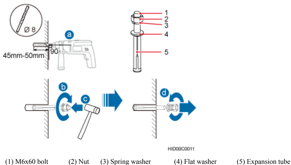
Figure 9-8 Drilling a hole and inserting an expansion bolt assembly
