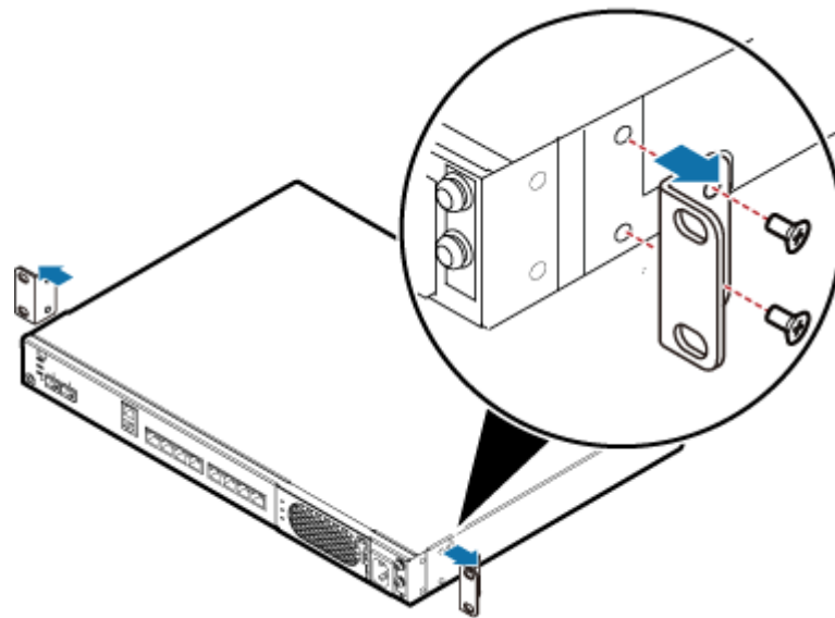
Figure 6-15 Removing mounting ears and screws
