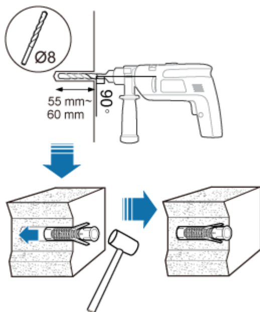
Figure 7-7 Drilling holes and installing expansion bolts
