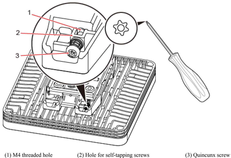
Figure 8-34 Locking the protection screw
