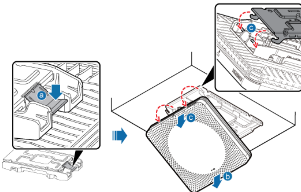
Figure 5-8 Removing the pRRU
