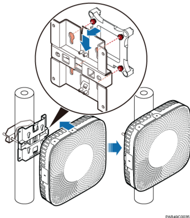
Figure 6-17 Installing a pRRU3901
