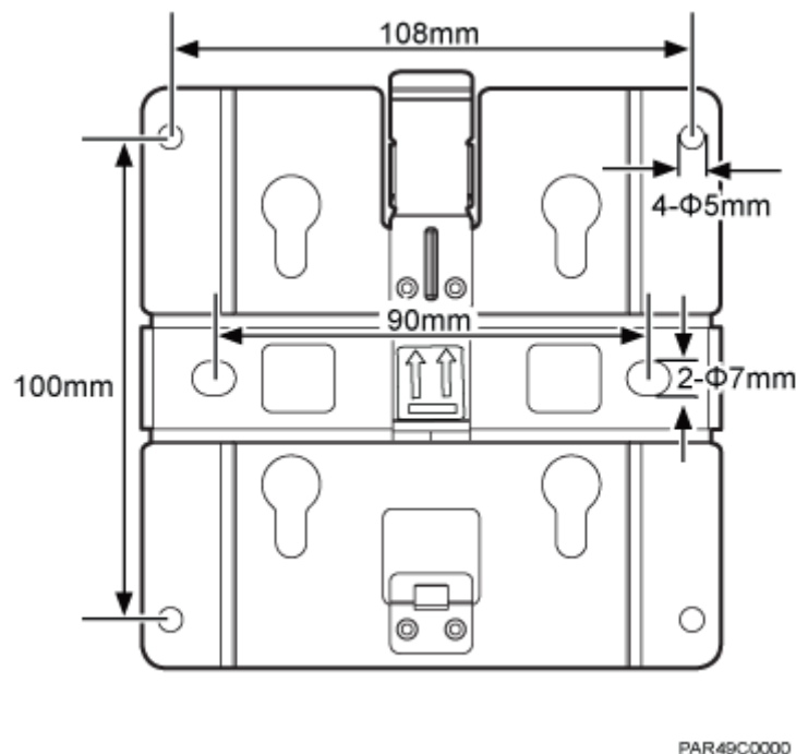
Figure 6-6 Plate specifications
