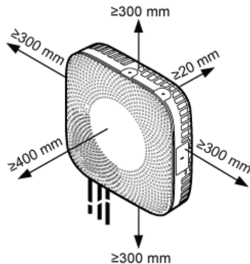
Figure 6-1 Recommended space requirements of the pRRU3901
