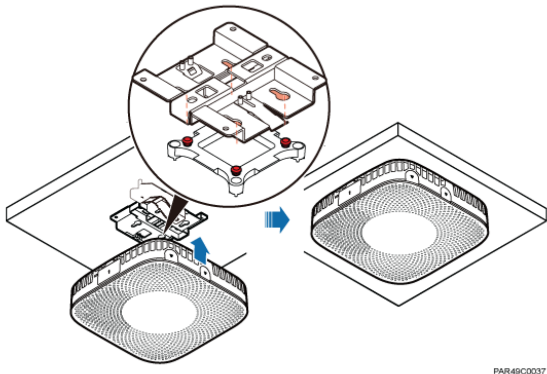
Figure 6-20 Installing a pRRU3901
