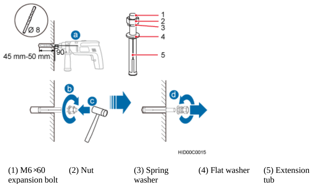
Figure 5-25 Drilling holes and installing expansion bolts
