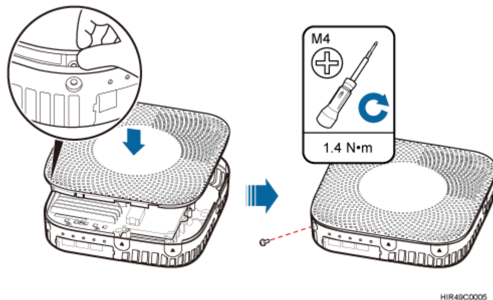
Figure 8-11 Installing the pRRU3901 housing
