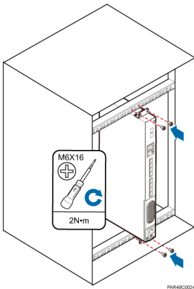
Figure 5-18 Tightening screws
