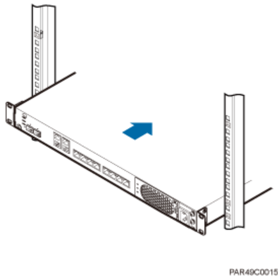
Figure 5-16 Pushing an RHUB3908 into a cabinet
