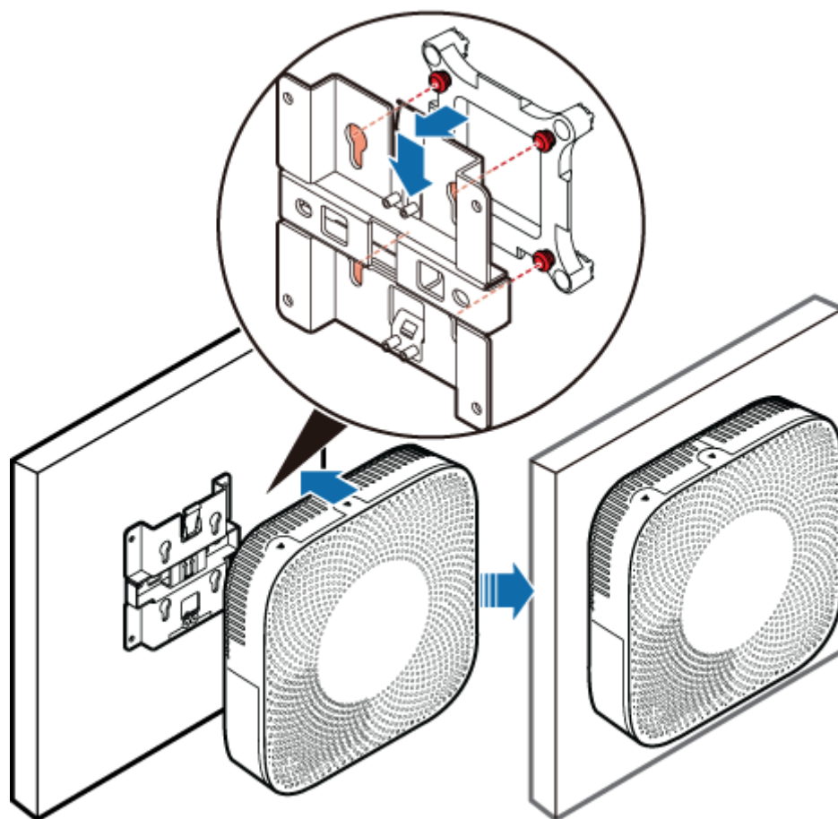
Figure 6-10 Installing the pRRU3901 on a plate
