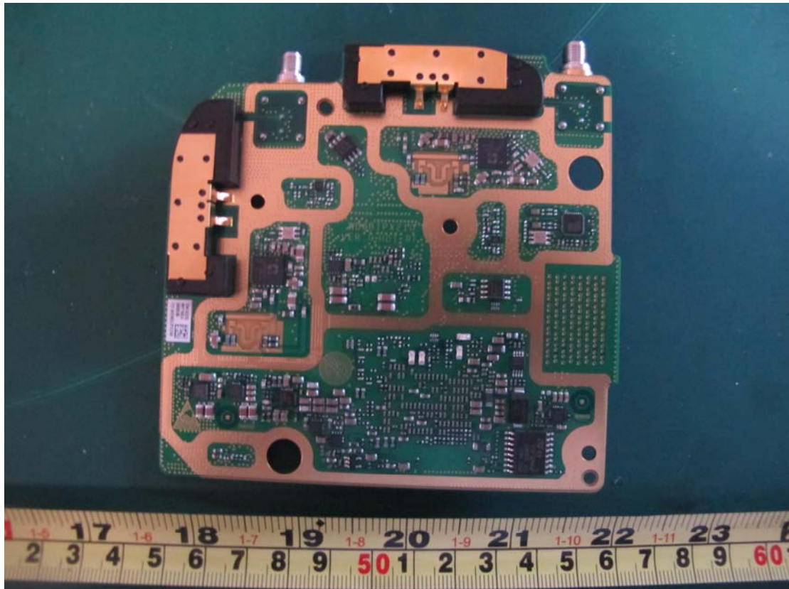
Photo-01 Heads of WD6DLPX240 (UMTS Band IV, LTE band 4)
