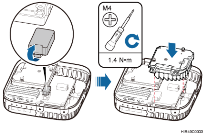
Figure 8-8 Installing the RF daughter board in slot S2
