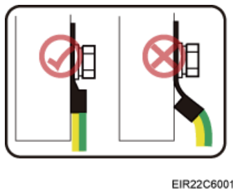
Figure 5-30 Correct direction of an OT terminal for the PGND cable
