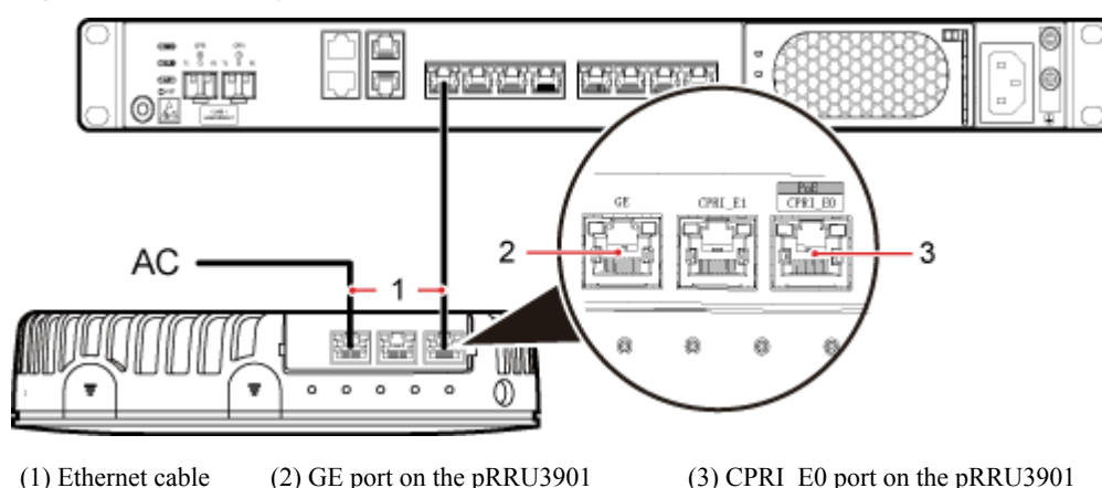
Figure 6-29 Installing an Ethernet cable
