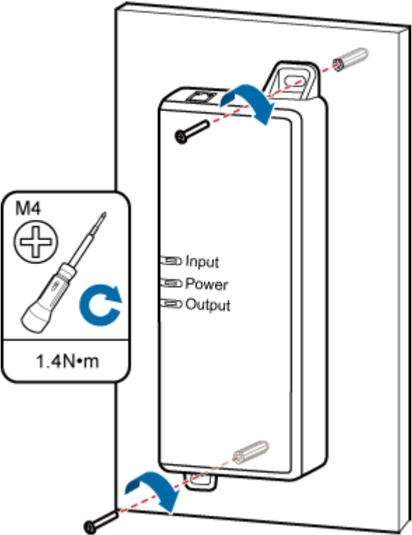
Figure 7-3 Installing Extender
