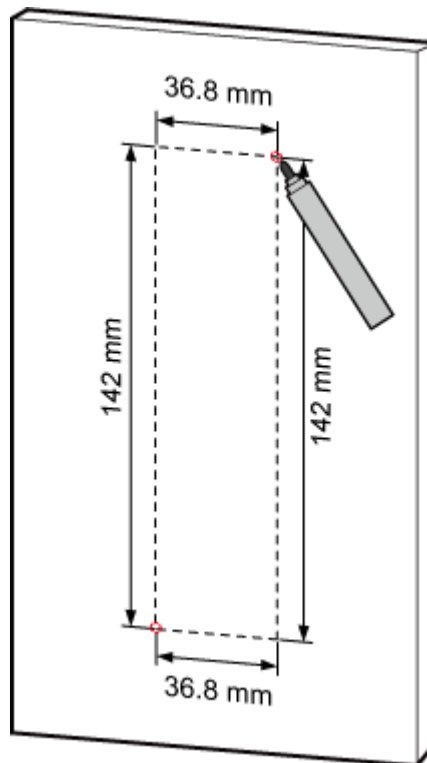
Figure 7-1 Marking anchor points
