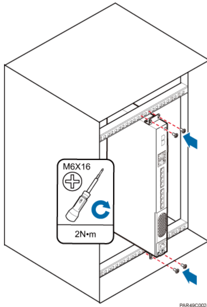
Figure 5-18 Tightening screws
