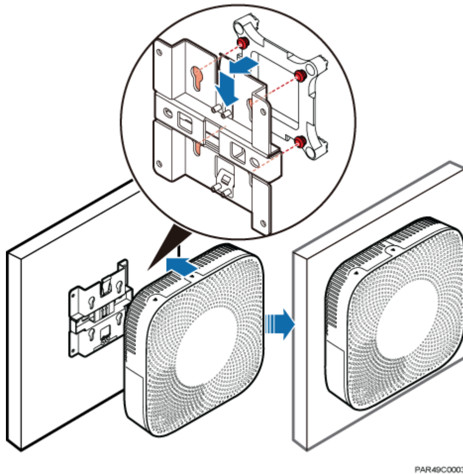
Figure 6-10 Installing the pRRU3901 on a plate
