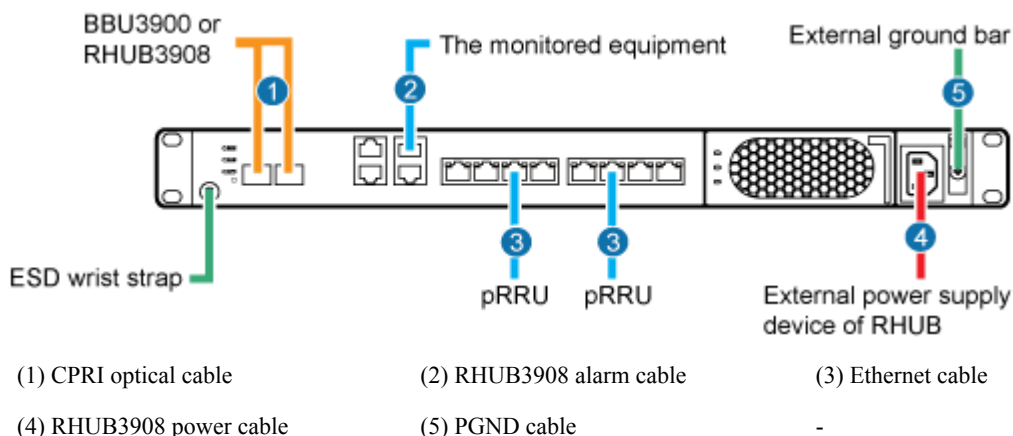
Figure 5-27 Cable connections for an RHUB3908
