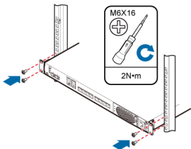
Figure 5-17 Tightening screws
