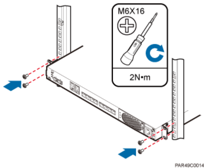
Figure 5-13 Tightening screws
