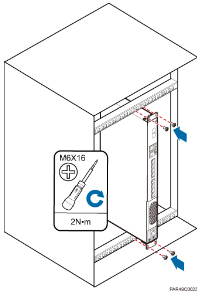
Figure 5-21 Tightening screws
