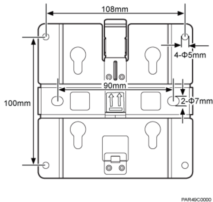
Figure 6-6 Plate specifications
