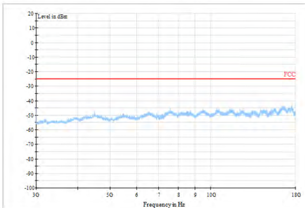
RSE-TX-DIRECTOR.ABOVE 1.5G_H
