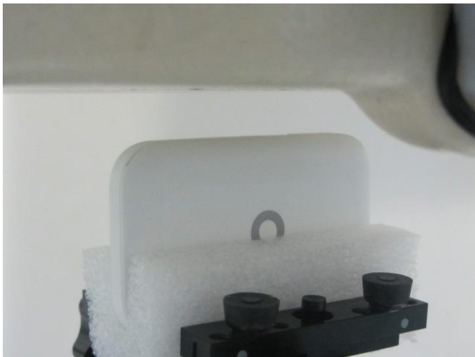
Photo 9: Bottom Side(10mm)
