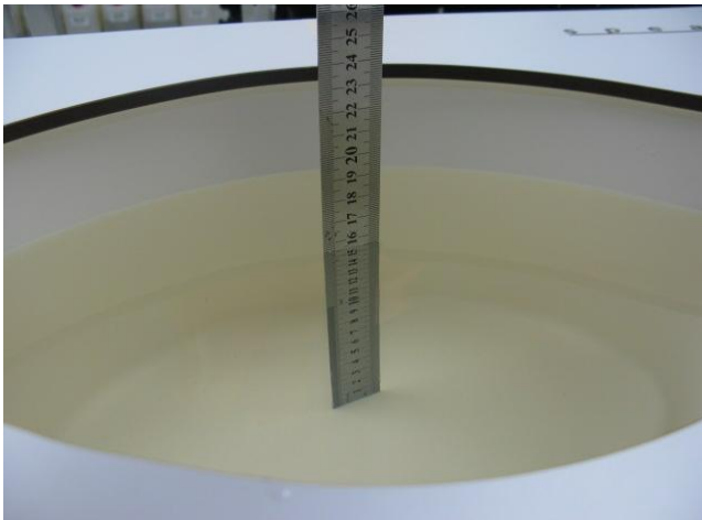
Photo 14: MBBL 3500-5800 MHz depth (15.1cm)
