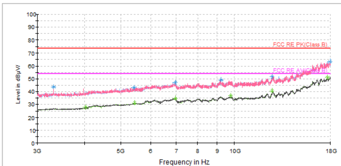
Radiated Emission from 3GHz to 18GHz
