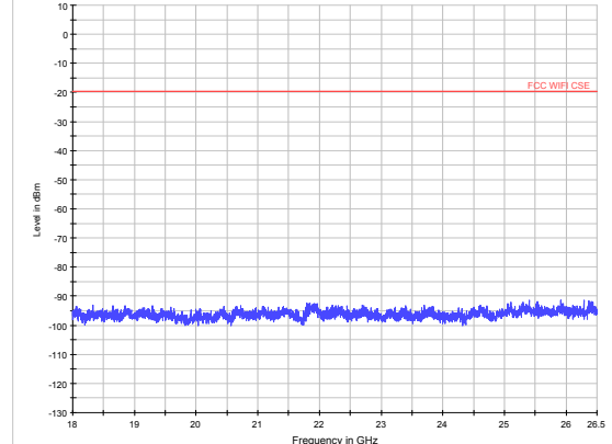
802.11b CH10 18GHz to 26.5GHz
