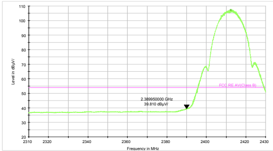
802.11b-Channel 1: Average
