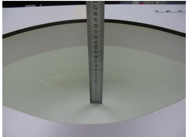
Photo 13: MSL 2600MHz depth (15.3cm)
