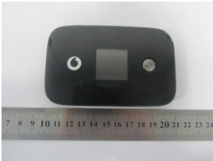
Photo 4: Front Side(10mm)
