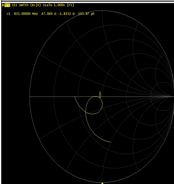
Impedance Test-Body
