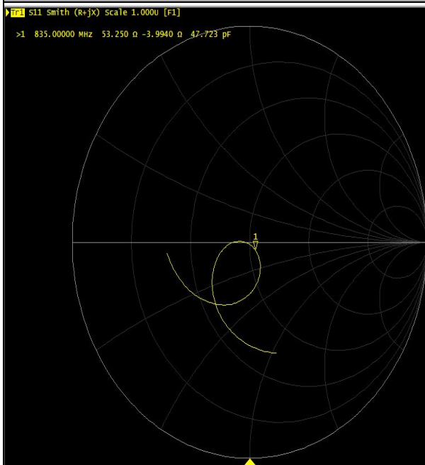
Impedance Test-Body
