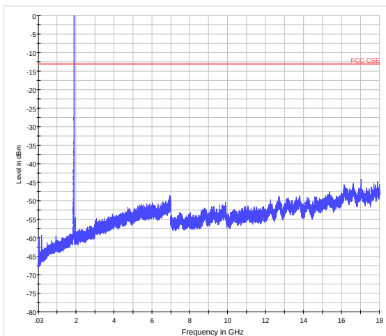
WCDMA Band II CH-High 30MHz~18GHz
