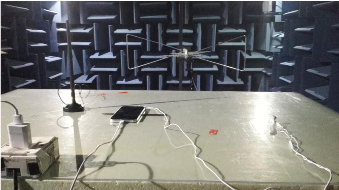
Radiated Spurious Emission (30M~1GHz)
