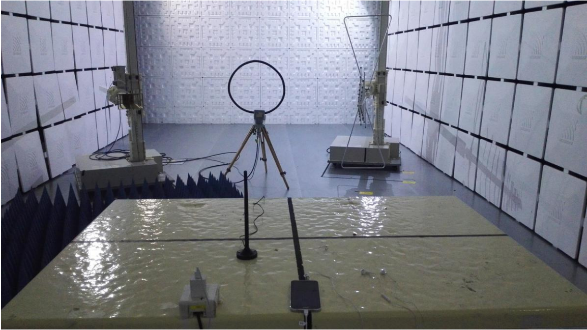
Radiated Spurious Emission (9K~30MHz)
