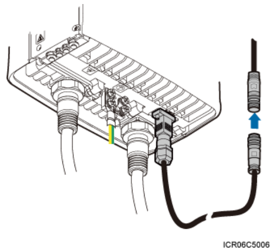
Figure 8-12 Installing an RRU AISG multi-wire cable
