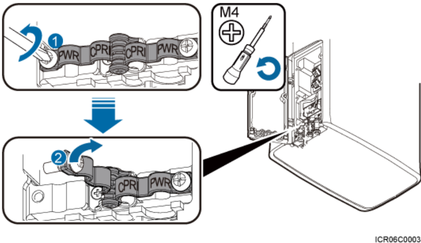
Figure 8-16 Opening clips
