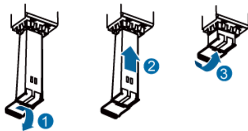
Figure 8-18 Installing an optical module
