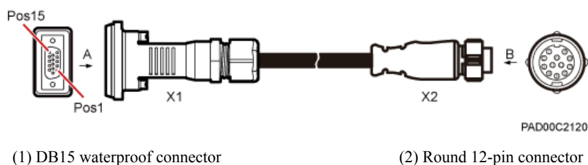
Figure 3-8 RGPS jumper
