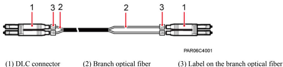
Figure 3-4 Fiber optical cable between a BBU and an RRU or between RRUs
