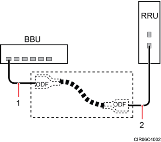
(1) Single-mode CPRI fiber optic cable between a BBU (2) Single-mode CPRI fiber optic cable between an ODF and an RRU
