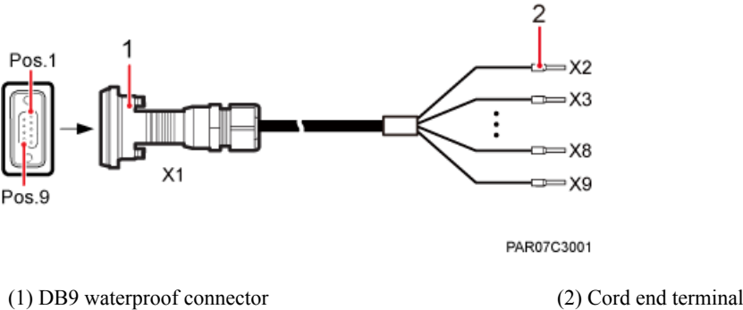
Figure 3-3 RRU alarm cable
