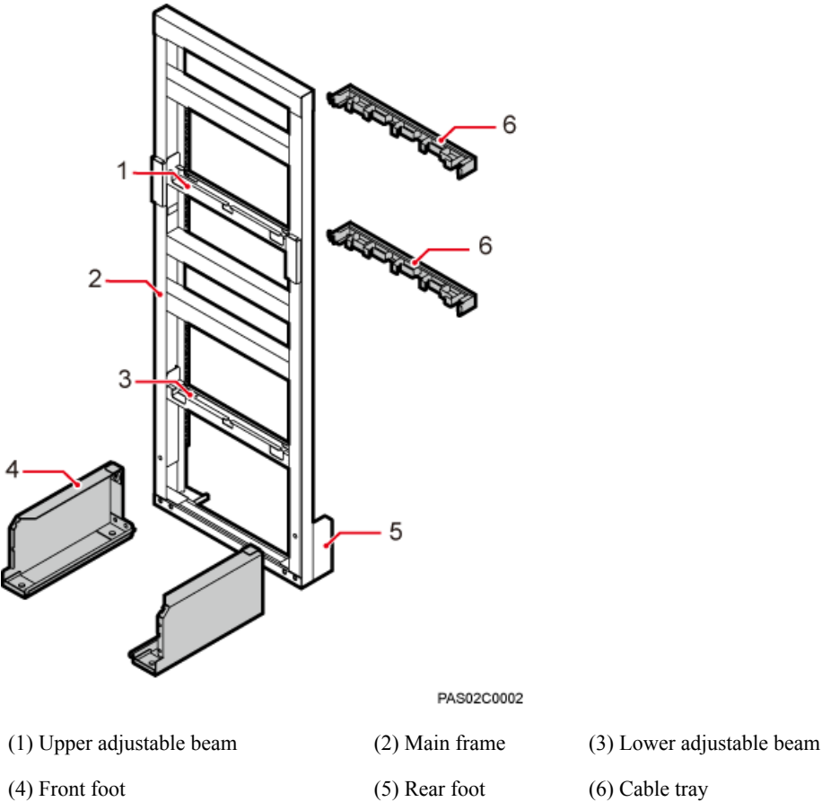
Figure 4-2 IFS06 structure
