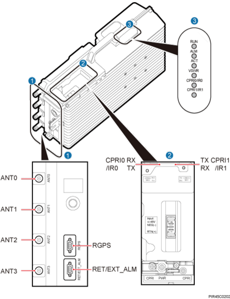
Figure 2-3 Ports on the RRU panels
