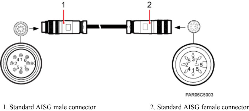
Figure 3-12 AISG extension cable
