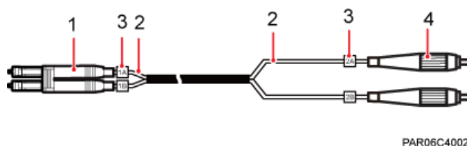
Figure 3-6 Single-mode fiber optic cable between a BBU and an ODF or between an ODF and an RRU
