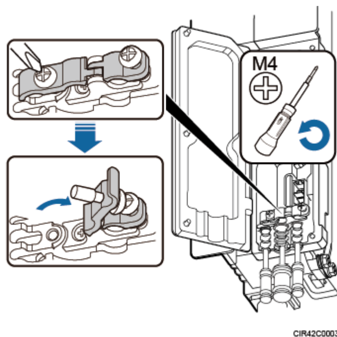
Figure 9-24 Opening clips
