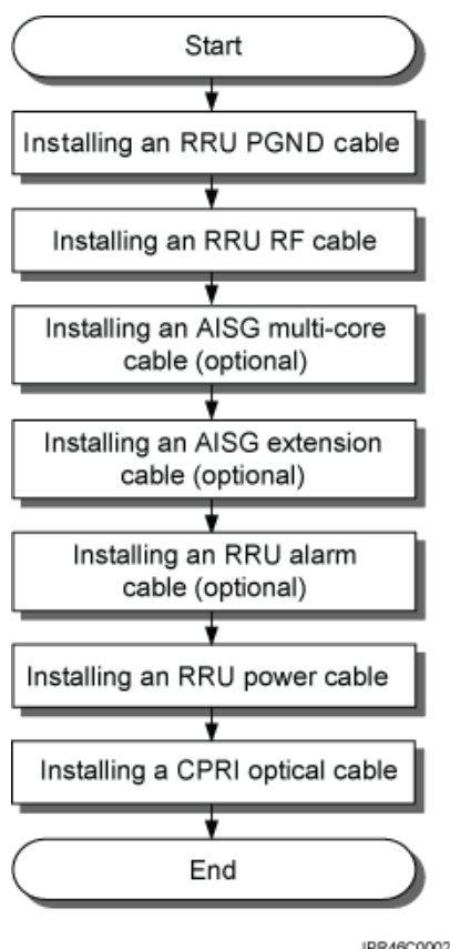
Figure 9-11 Process of installing RRU cables
