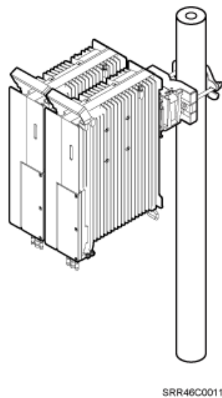
Figure 3-10 Two RRUs installed on a pole
