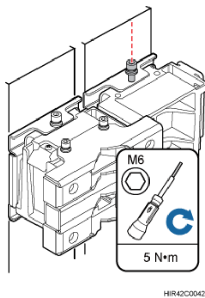
Figure 8-13 Securing the captive screw into the connection hole
