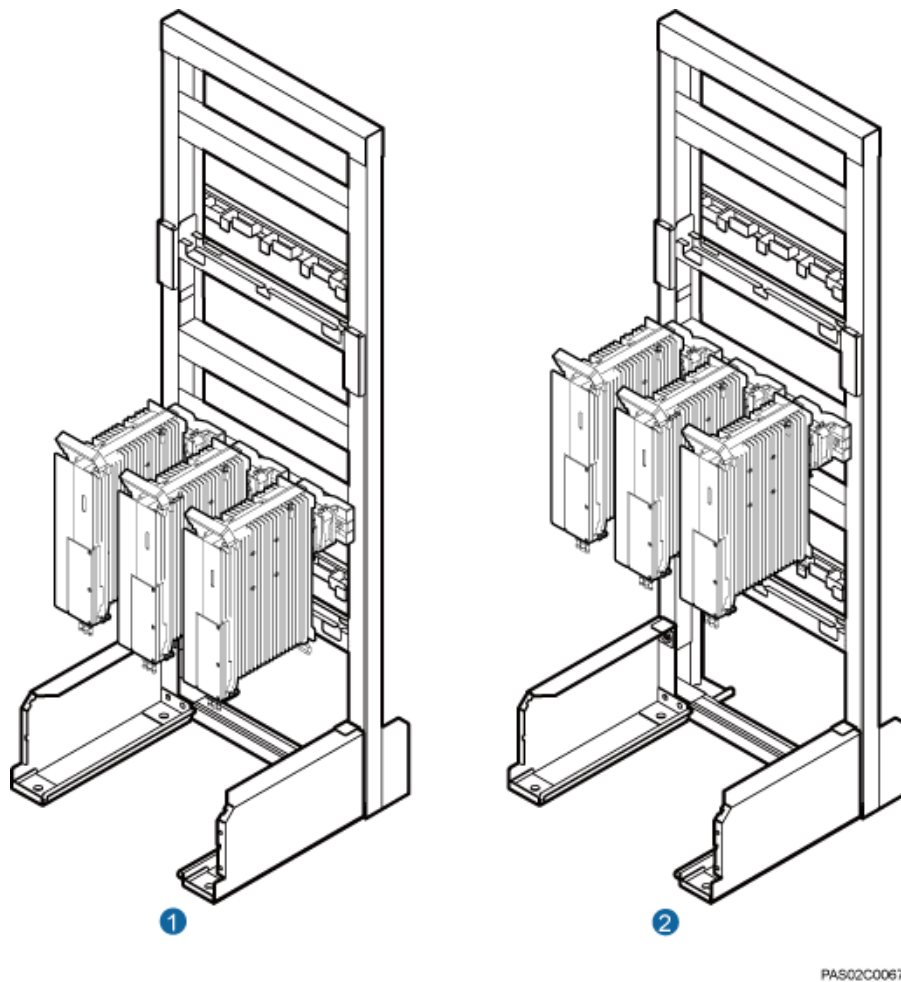
Figure 3-18 Three RRUs installed on an IFS06
