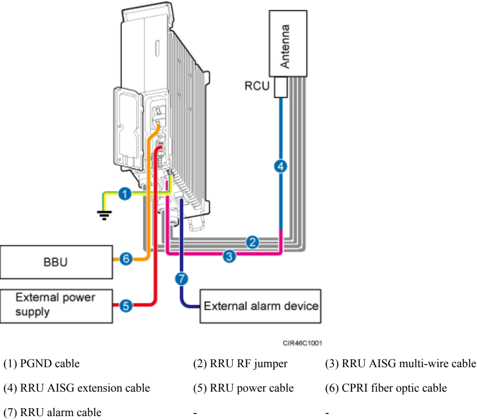
Figure 9-9 Cable connections for a single RRU
