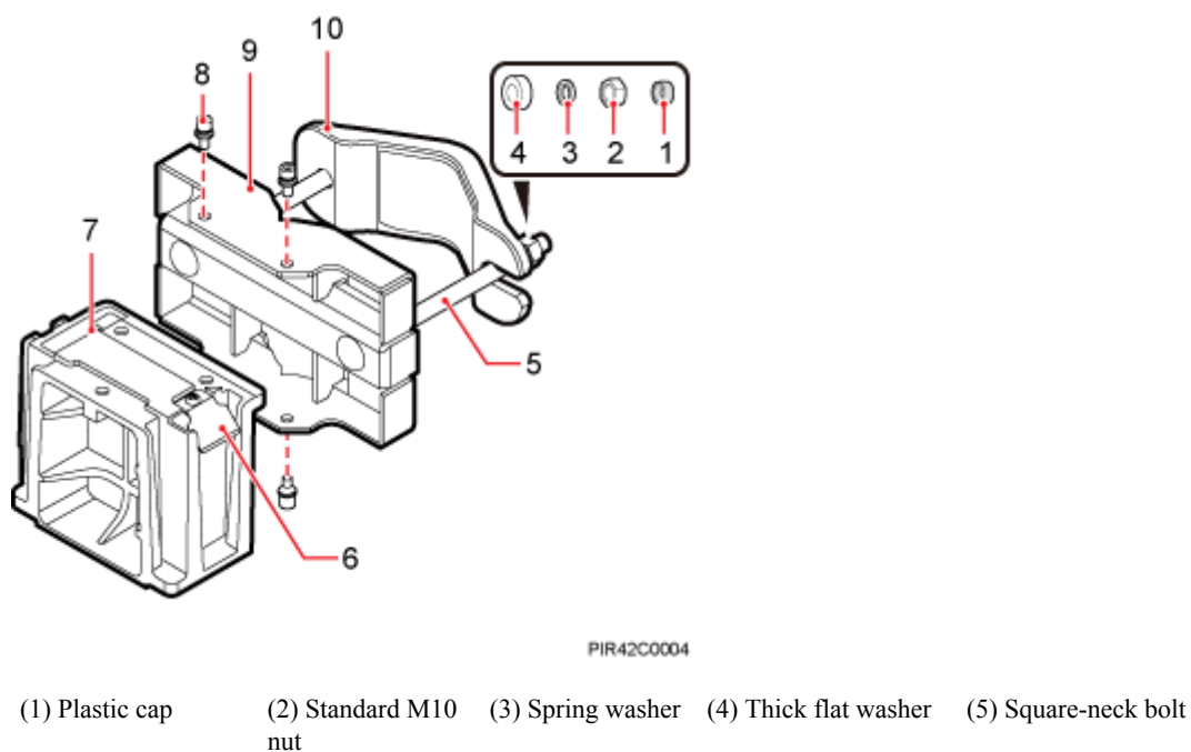
Figure 8-2 12 L blade RRU mounting kit
