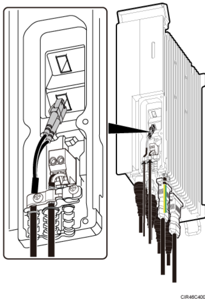
Figure 9-27 Installing CPRI optical cables for dual-fiber bidirectional optical modules
