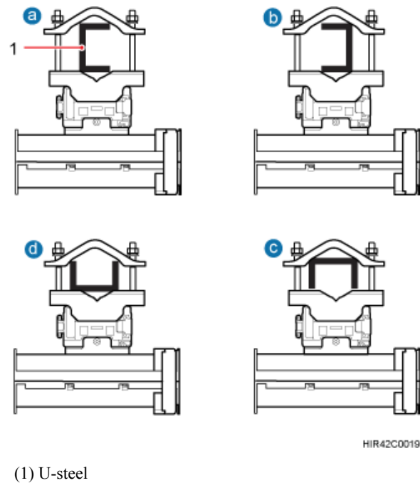
Figure 8-22 Top view of the RRU
