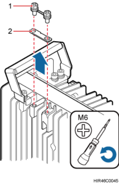
Figure 6-1 Removing the metal sheet
