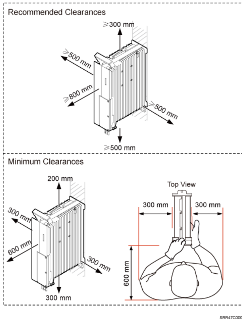
Figure 3-21 Clearance for a single RRU in side-mounted mode
