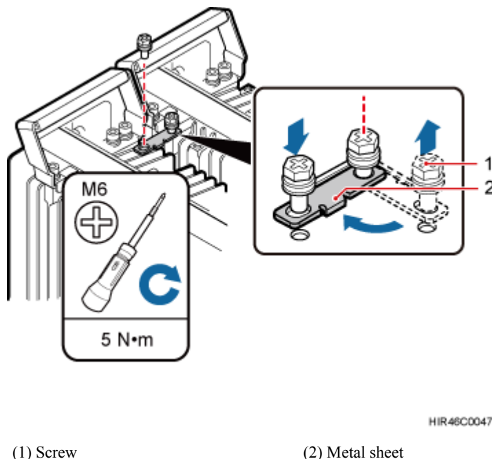
Figure 8-14 Installing the metal sheet
