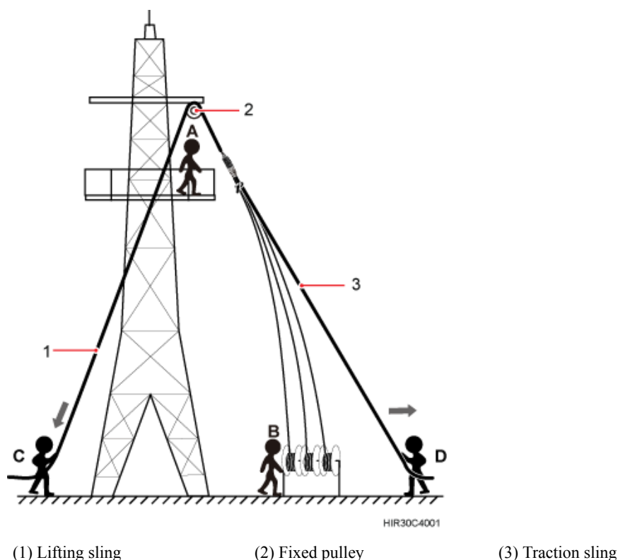
Figure 7-6 Hoisting fiber optic cables onto the tower
