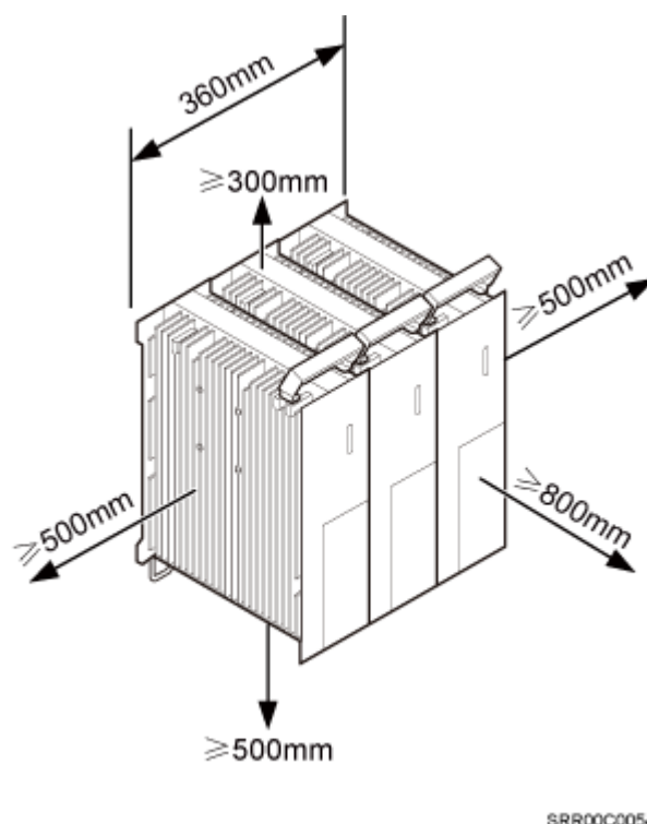
Figure 3-24 Recommended clearances for three or more RRUs installed on a pole
