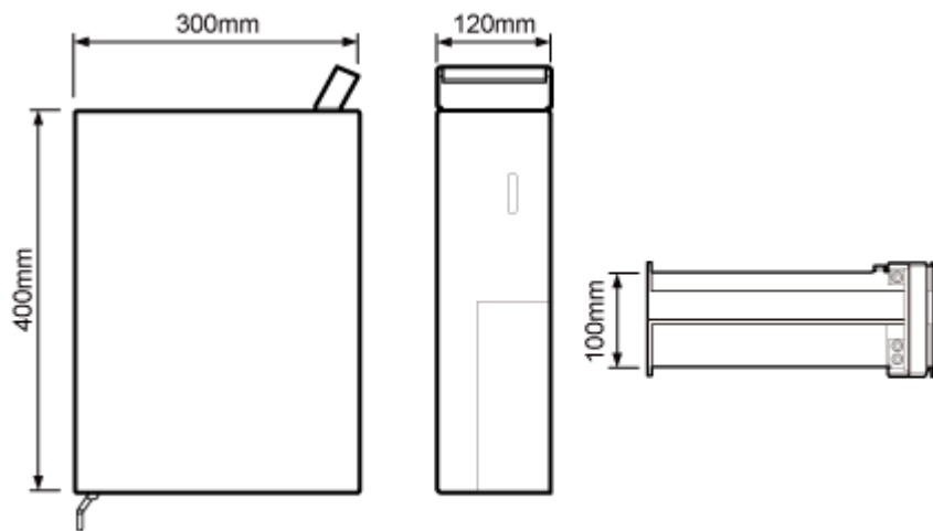
Figure 3-2 RRU dimensions
