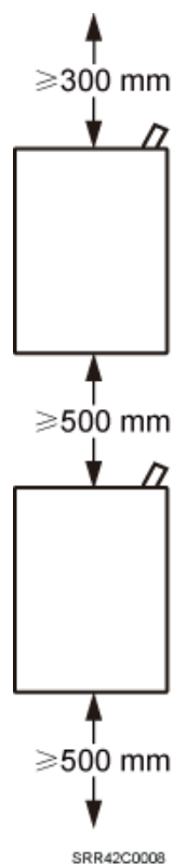
Figure 3-31 Recommended vertical spacing between RRUs
