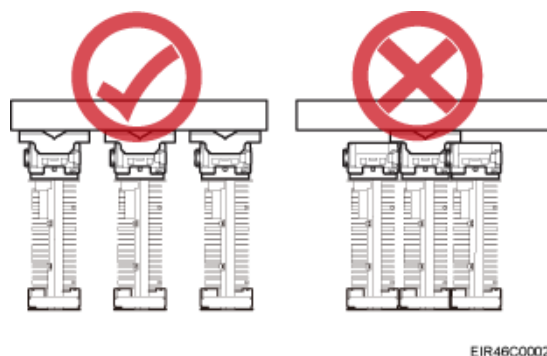
Figure 3-15 Correct installation of mounting brackets for multiple RRUs installed on a wall in side-mounted mode
