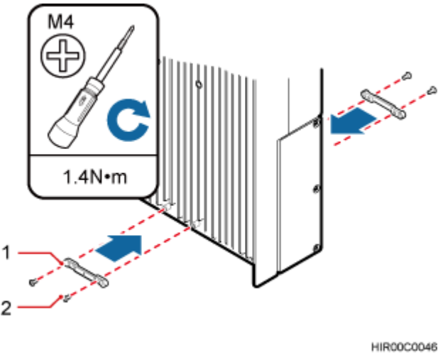
Figure 6-2 Installing buckles at the bottom
