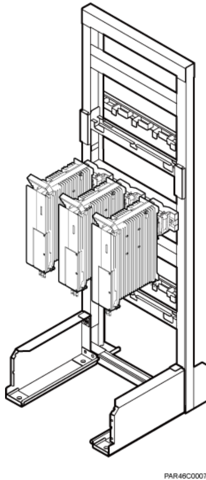
Figure 8-49 Installing RRUs on the lower level
