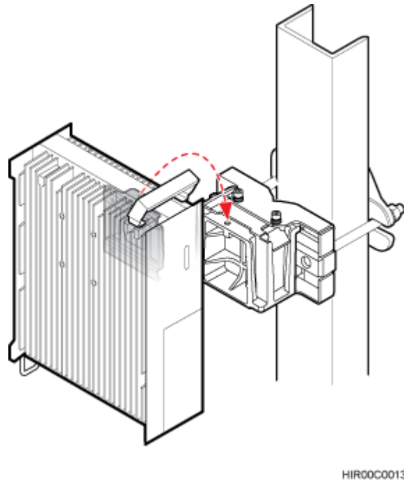
Figure 8-27 Installing the RRU onto the main bracket
