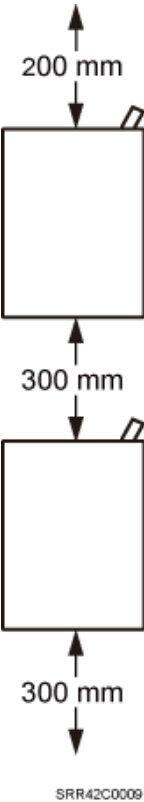
Figure 3-32 Minimum vertical spacing between RRUs
