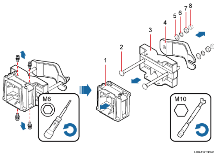
Figure 8-44 Disassembling the mounting brackets
