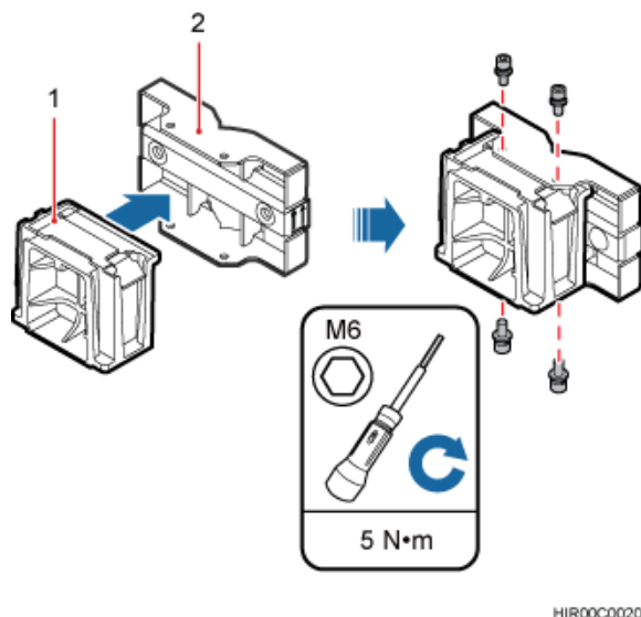
Figure 8-47 Installing the main bracket
