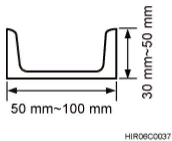
Figure 3-12 U-steel specifications
