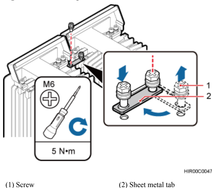
Figure 8-19 Installing the sheet metal tab
