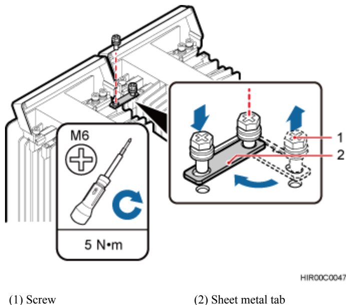
Figure 8-14 Installing the sheet metal tab
