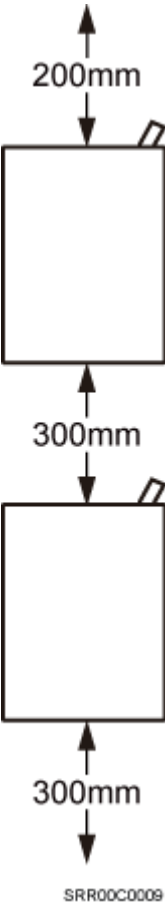
Figure 3-33 Minimum vertical spacing between RRUs
