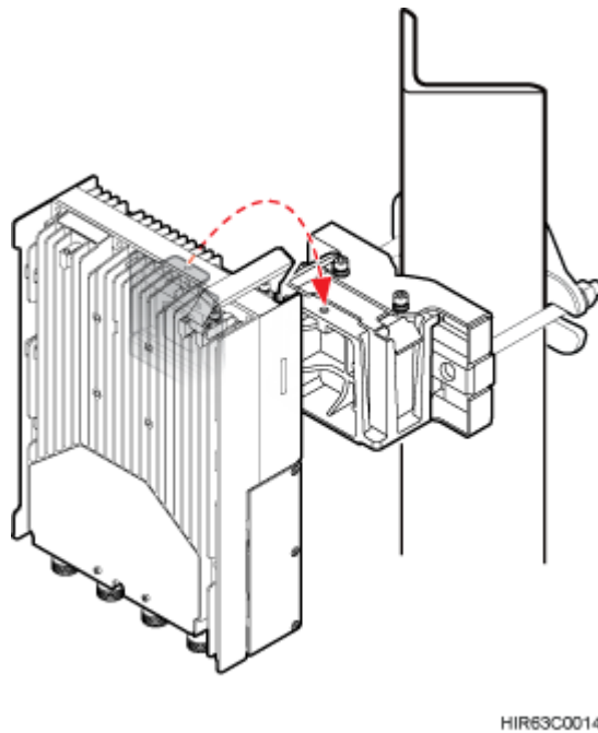
Figure 8-34 Installing the RRU onto the main bracket
