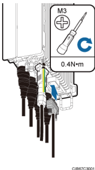
Figure 9-19 Installing an RRU alarm cable
