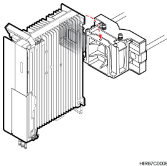
Figure 8-6 Installing the RRU onto the main bracket
