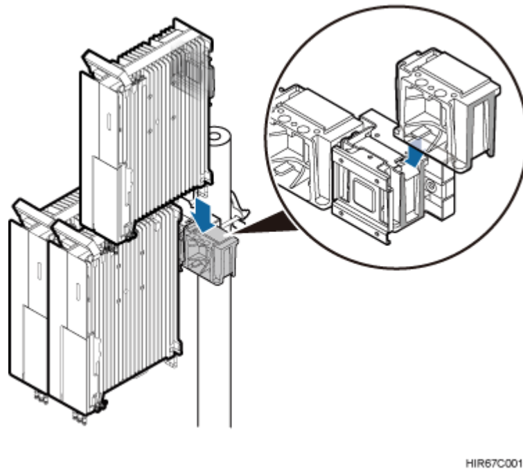
Figure 8-17 Installing the third RRU onto the third main bracket
