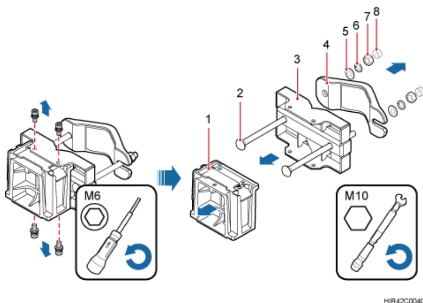
Figure 8-44 Disassembling the RRU mounting brackets
