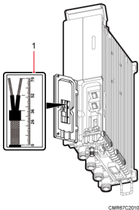
Figure 12-1 Cable diagram on labels
