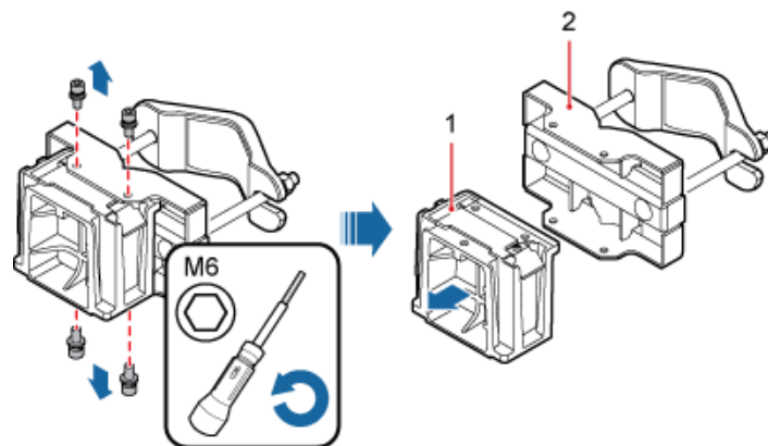
Figure 8-16 Removing the RRU main bracket
