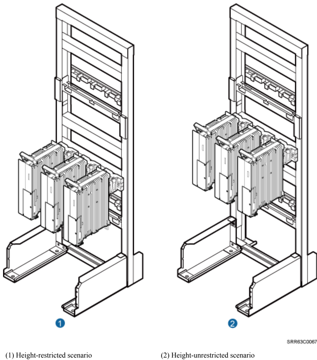
Figure 3-19 Three RRUs installed on an IFS06
