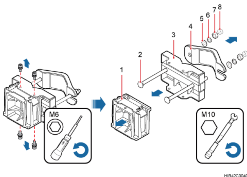
Figure 8-36 Disassembling the RRU mounting brackets
