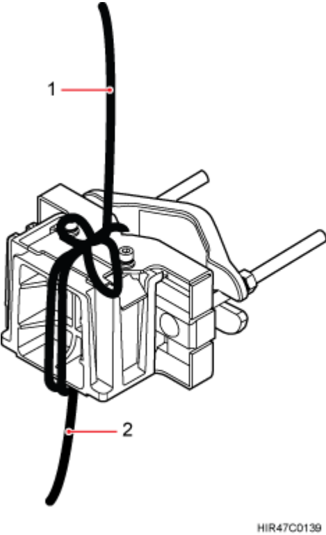
Figure 7-1 Binding mounting kits for the RRU
