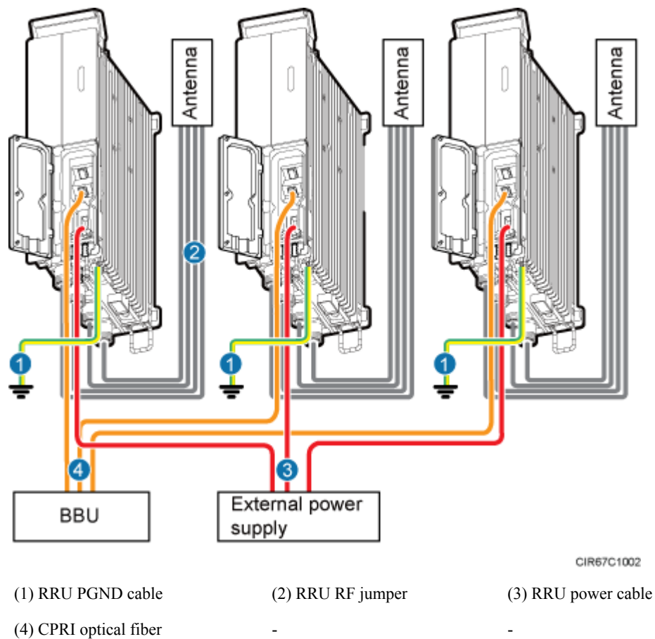
Figure 9-9 Cable connections of multiple RRUs
