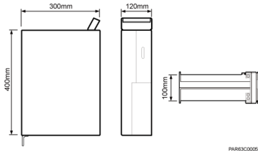
Figure 3-2 RRU dimensions
