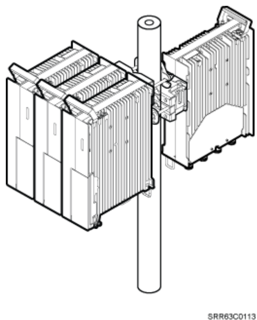
Figure 3-10 Four RRUs installed on a pole
