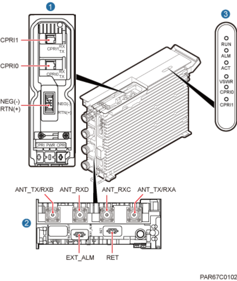
Figure 3-3 Ports on the RRU panels
