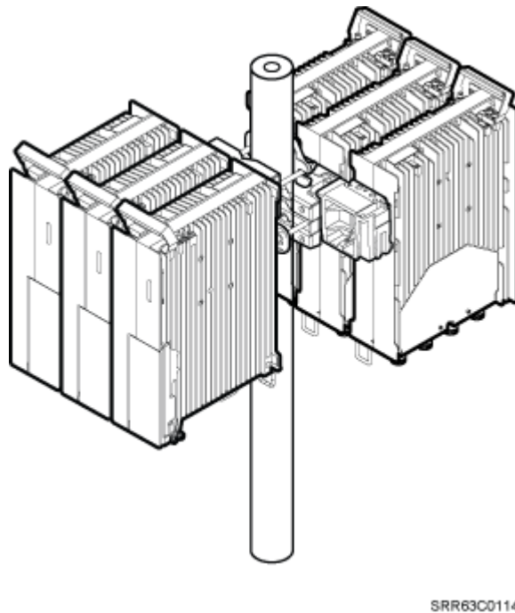
Figure 3-11 Six RRUs installed on a pole
