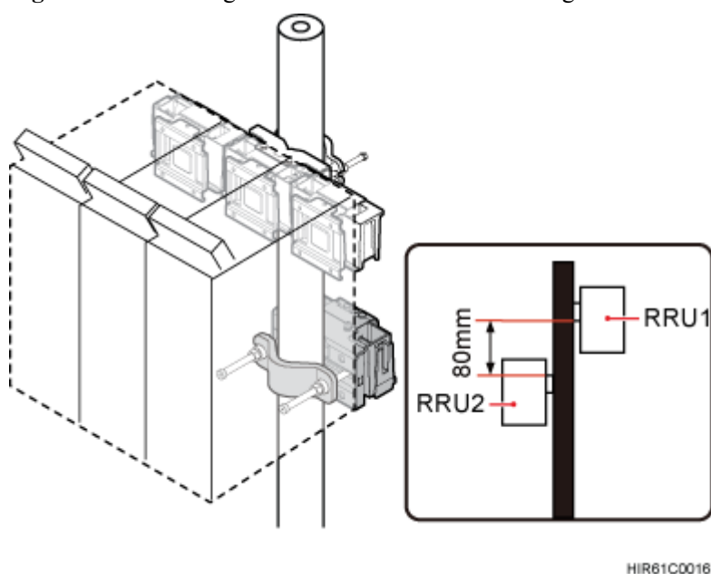
Figure 8-20 Installing the second set of RRU mounting brackets
