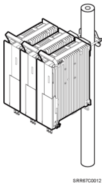
Figure 3-9 Three RRUs installed on a pole
