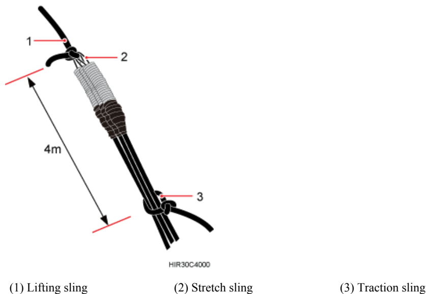
Figure 7-7 Binding fiber optic cables
