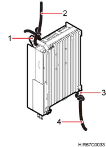
Figure 7-2 Binding the RRU
