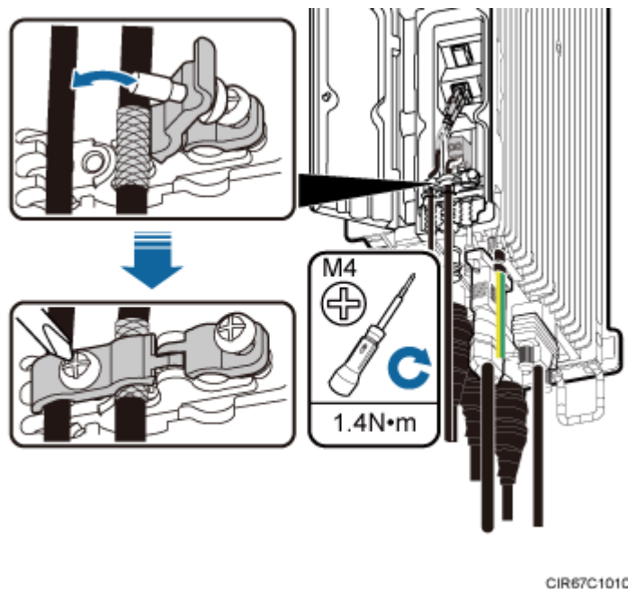
Figure 9-26 Closing clips
