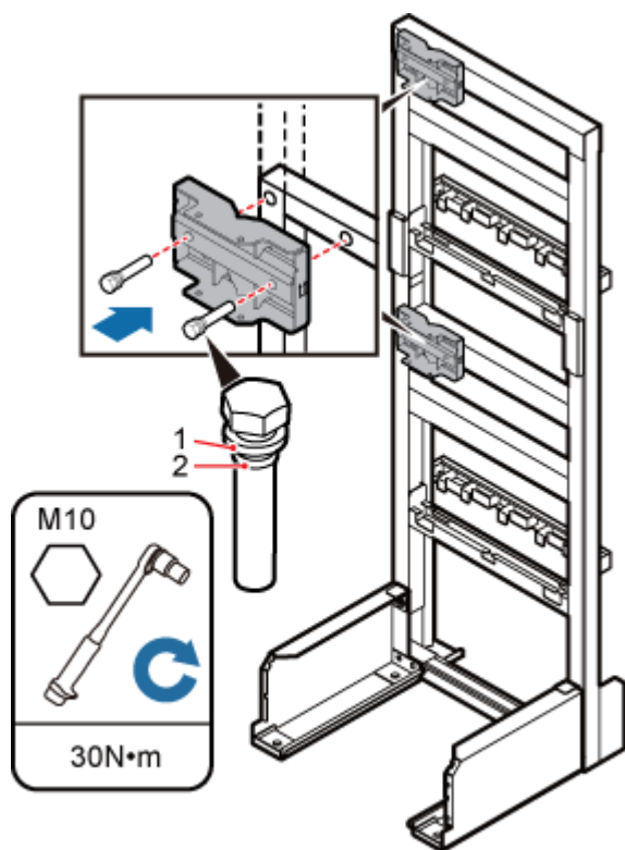
Figure 8-45 Installing the pole installation bracket in height-unrestricted scenarios
