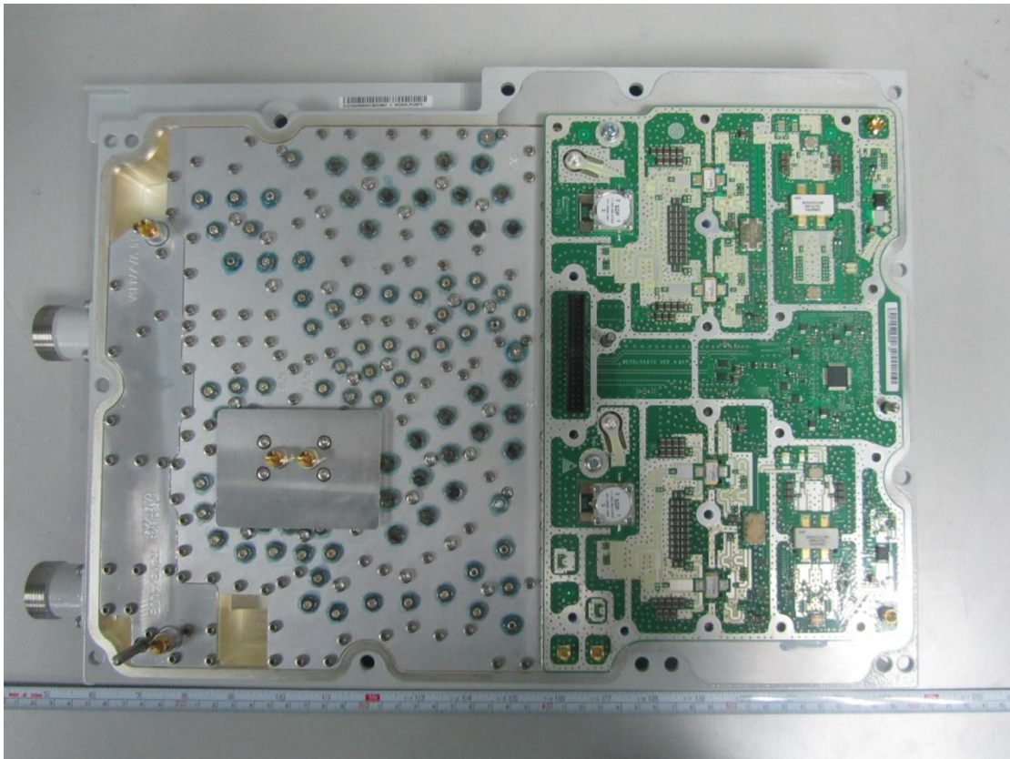
Board component side of RRU3268
