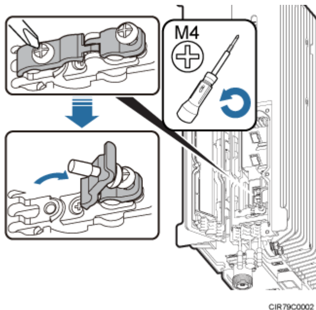
Figure 7-22 Opening clips
