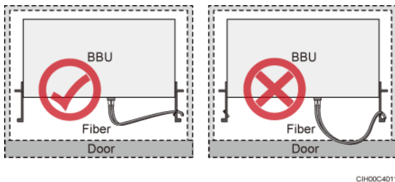
Figure 7-7 FE/GE cables routed through the cabinet
