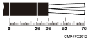
Figure 10-3 Stripping the specified length of sheath
