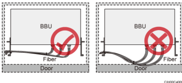
Figure 7-6 CPRI fiber optic cables routed through the cabinet (2)
