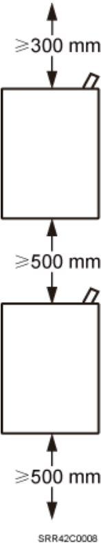
Figure 3-12 Recommended vertical spacing between RRUs
