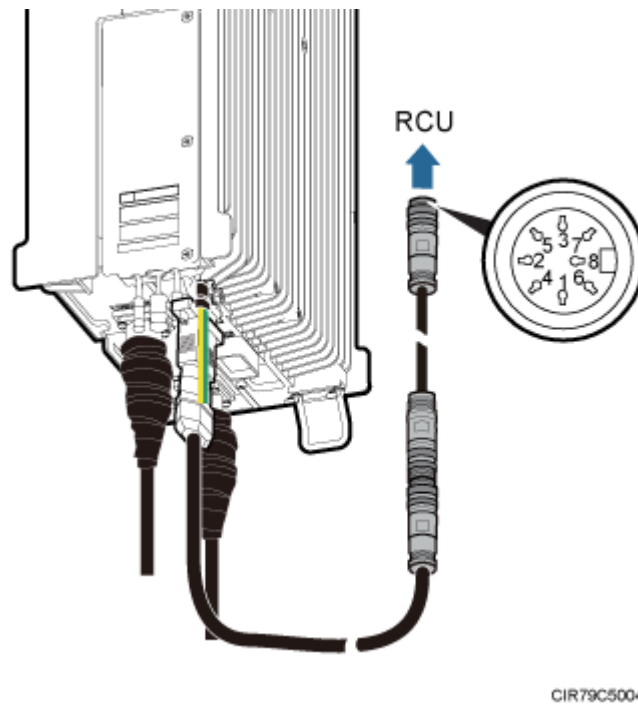
Figure 7-18 Installing an RRU AISG extension cable
