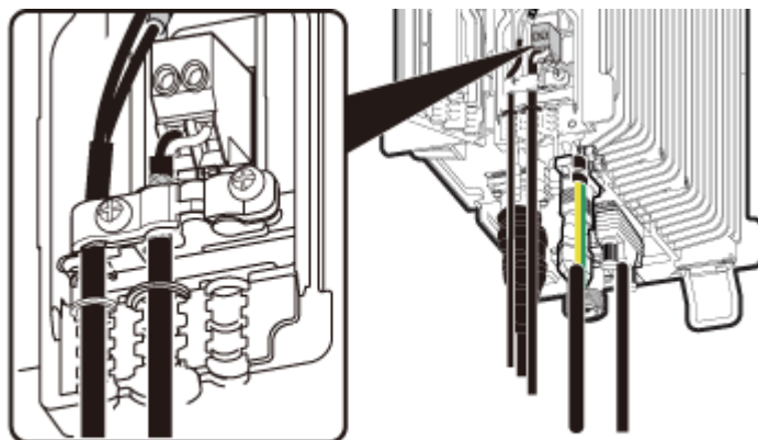
Figure 7-25 Installing an RRU power cable
