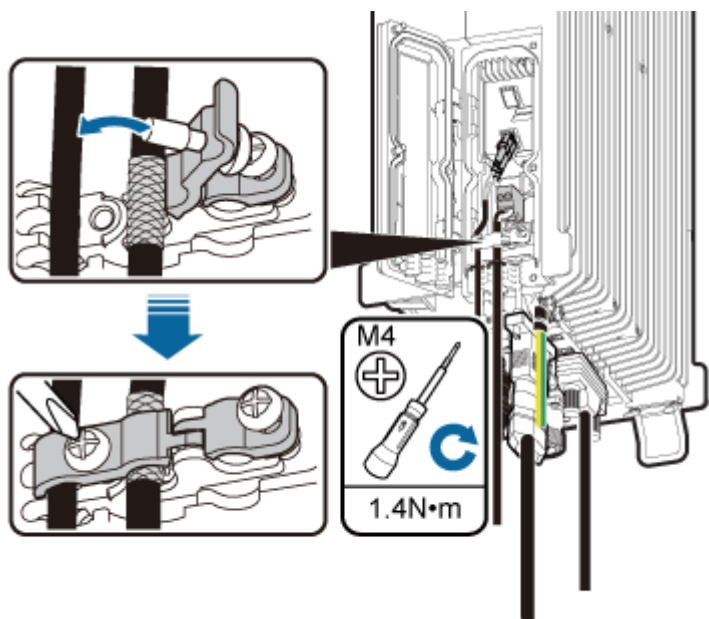
Figure 7-26 Closing clips
