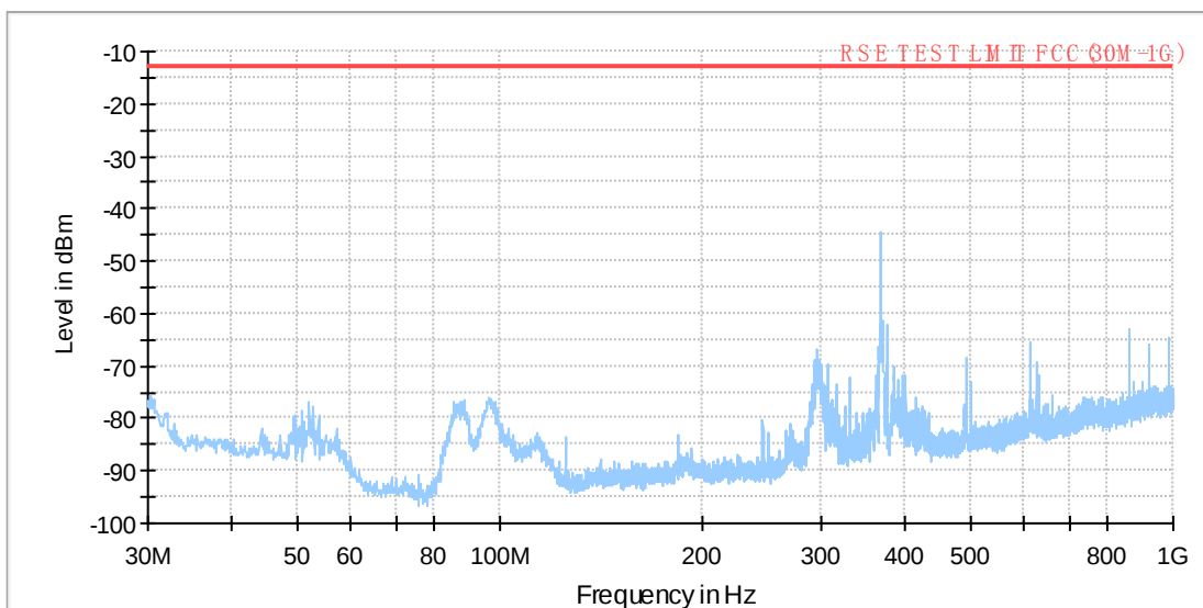
RSE TEST FCC(30M-1G)
