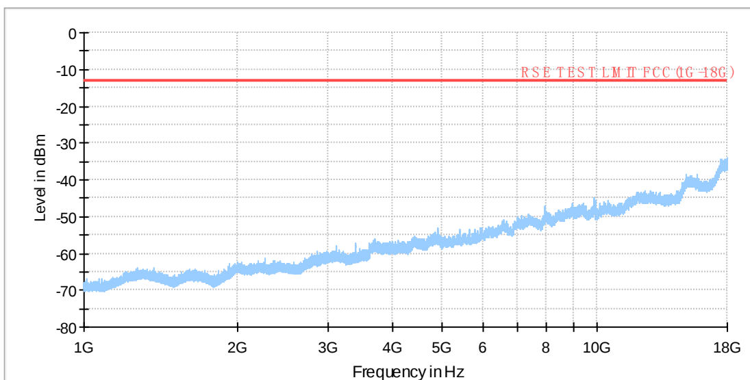
RSE TEST FCC(1G-18G)
