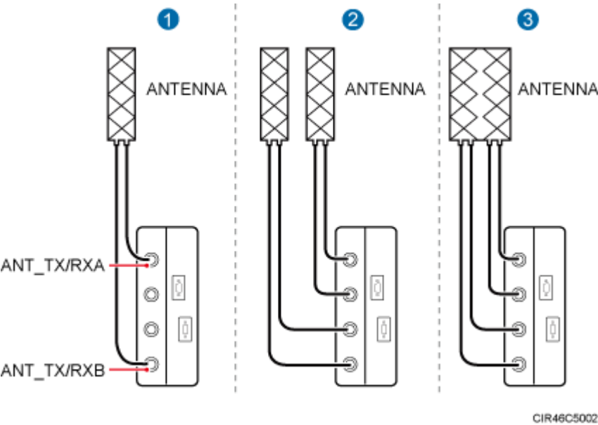
Figure 4-1 RF cable connections for the RRU
