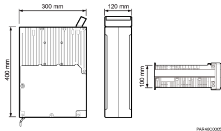
Figure 2-2 RRU dimensions
