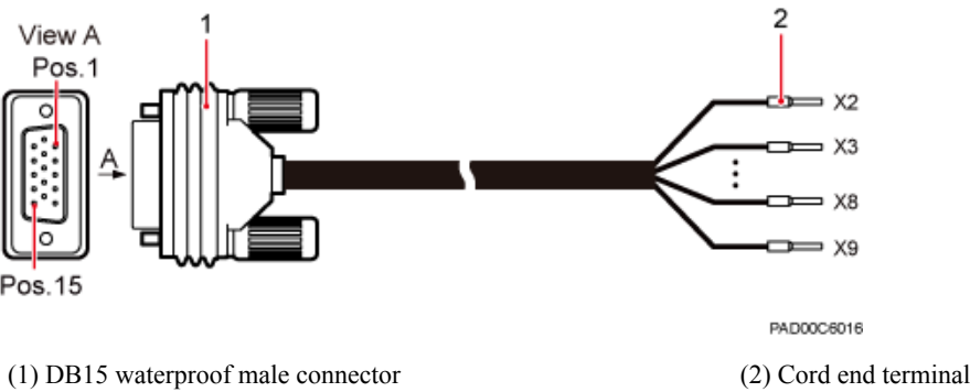
Figure 3-4 Alarm cable
