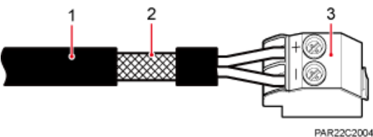
Figure 3-3 RRU power cable
