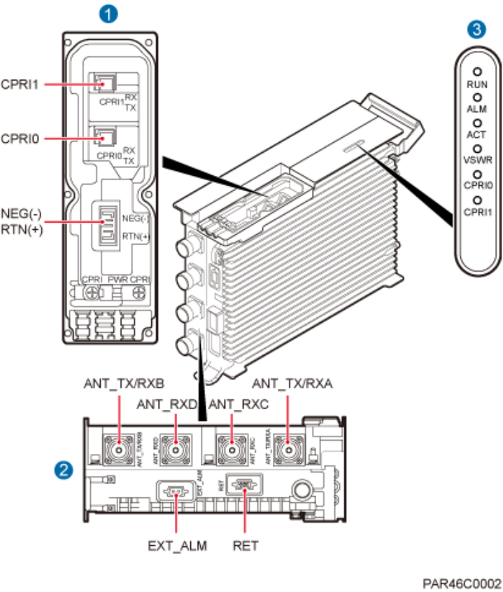
Figure 2-4 Ports on the RRU panels
