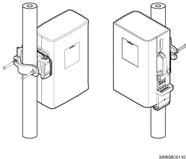
Figure 3-10 A single RRU installed on a pole
