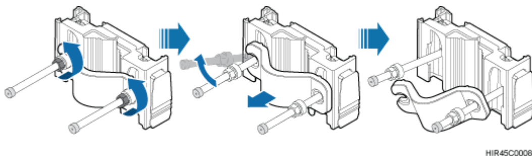
Figure 7-24 Moving the bolt out of the trough
