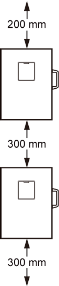
Figure 3-34 Minimum vertical spacing between RRUs
