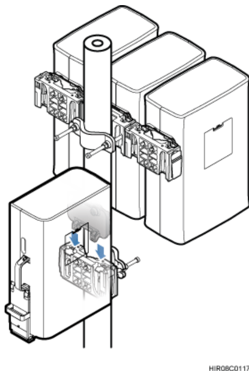
Figure 7-21 Installing the fourth RRU onto the fourth main bracket
