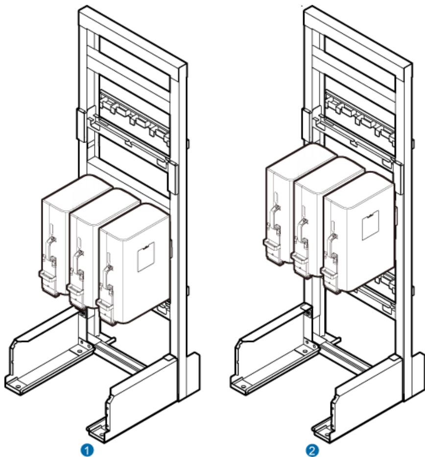
Figure 3-21 Three RRUs installed on an IFS06
