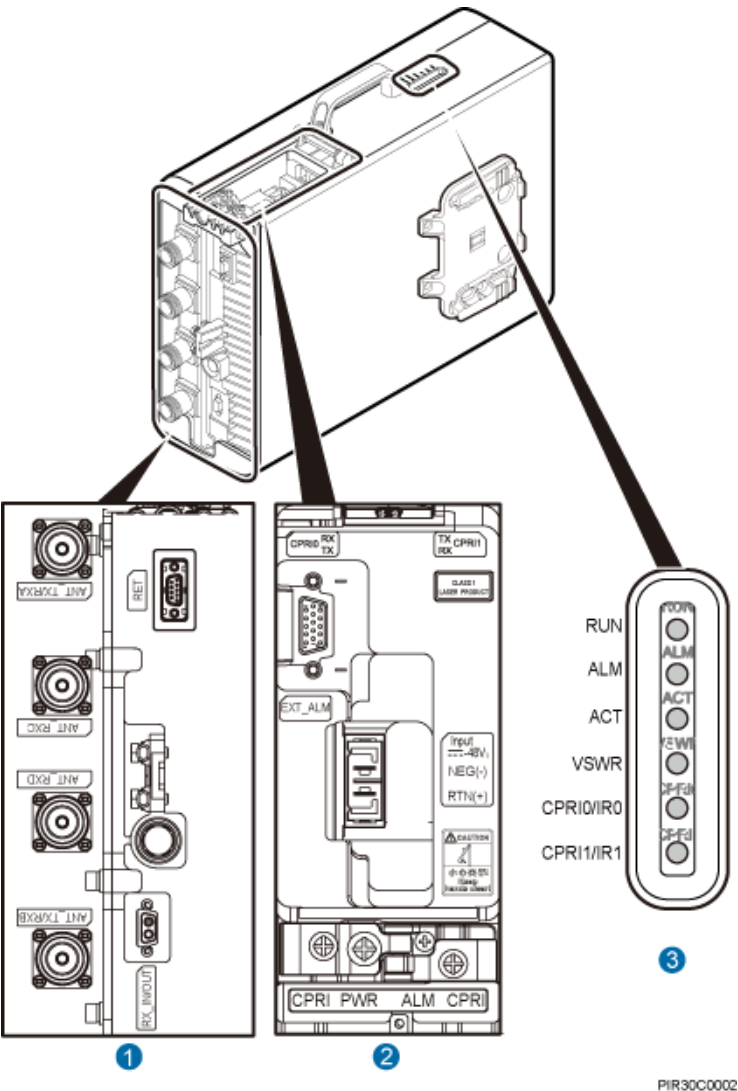
Figure 3-3 Ports on the RRU panels
