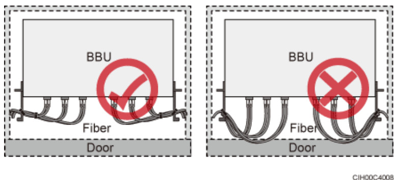
Figure 8-5 CPRI fiber optic cables routed through the cabinet (1)
