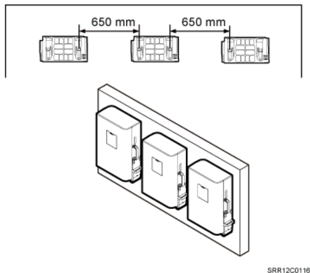
Figure 3-29 Minimum clearances for three or more RRUs installed on a wall in standard mode
