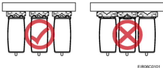
Figure 3-19 Correct installation of mounting brackets for multiple RRUs
