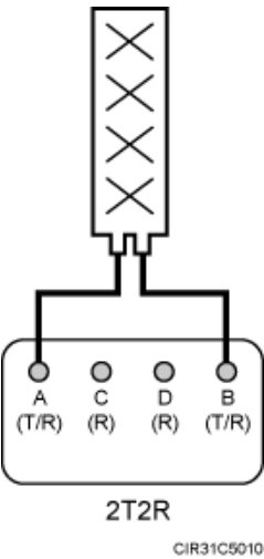
Figure 3-4 Recommended usage of RF ports on an RRU3942 used for DBS3900 V100R004C00, DBS3900 GSM V100R013C00, DBS3900 GSM V300R013C00, or DBS3900 WCDMA V200R013C00
