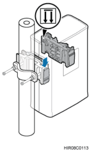
Figure 7-11 Installing the second main bracket
