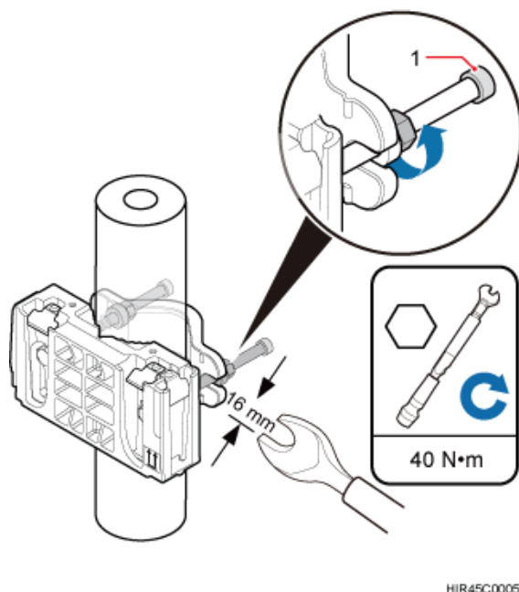
Figure 7-6 Securing the main and auxiliary brackets onto the pole
