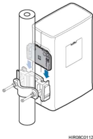
Figure 7-10 Installing the first RRU onto the main bracket
