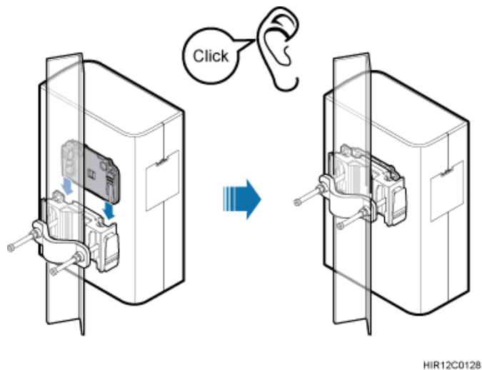
Figure 7-33 Installing the RRU onto the main bracket
