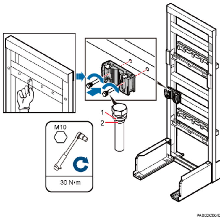
Figure 7-39 Installing the main bracket in height-restricted scenarios
