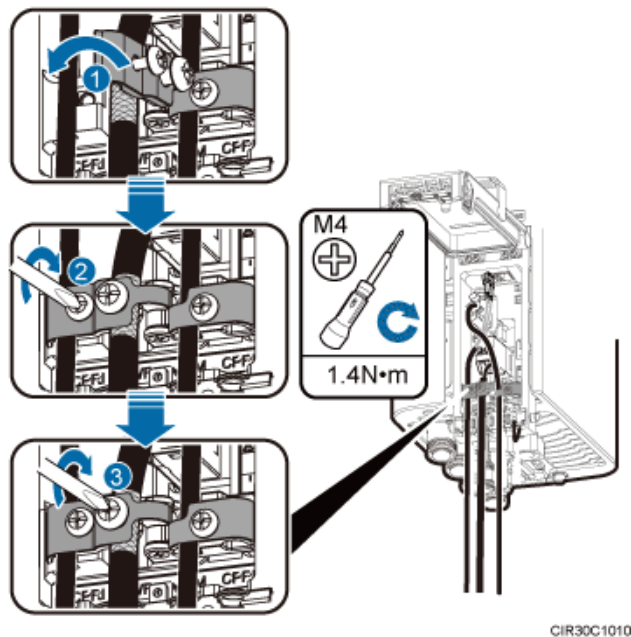
Figure 8-30 Closing clips
