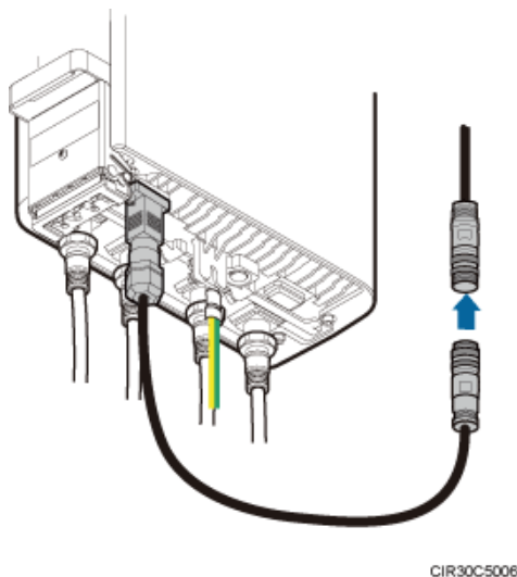
Figure 8-21 Installing an RRU AISG multi-wire cable
