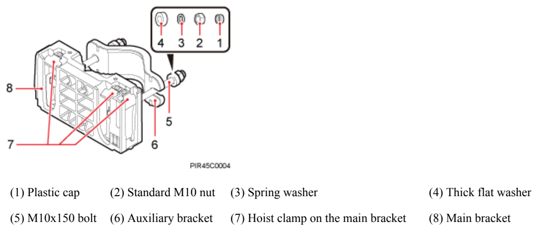
Figure 7-2 Common RRU mounting kit
