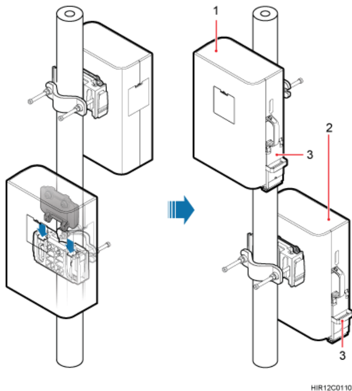
Figure 7-16 Installing the second RRU onto the main bracket
