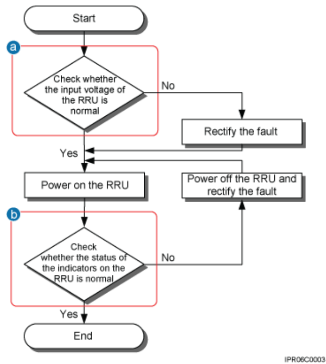
Figure 10-1 RRU power-on check process
