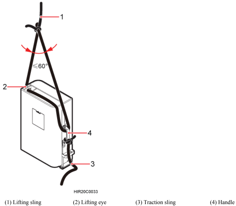
Figure 6-2 Binding the RRU
