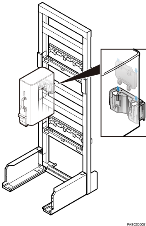
Figure 7-42 Installing the RRU onto the main bracket
