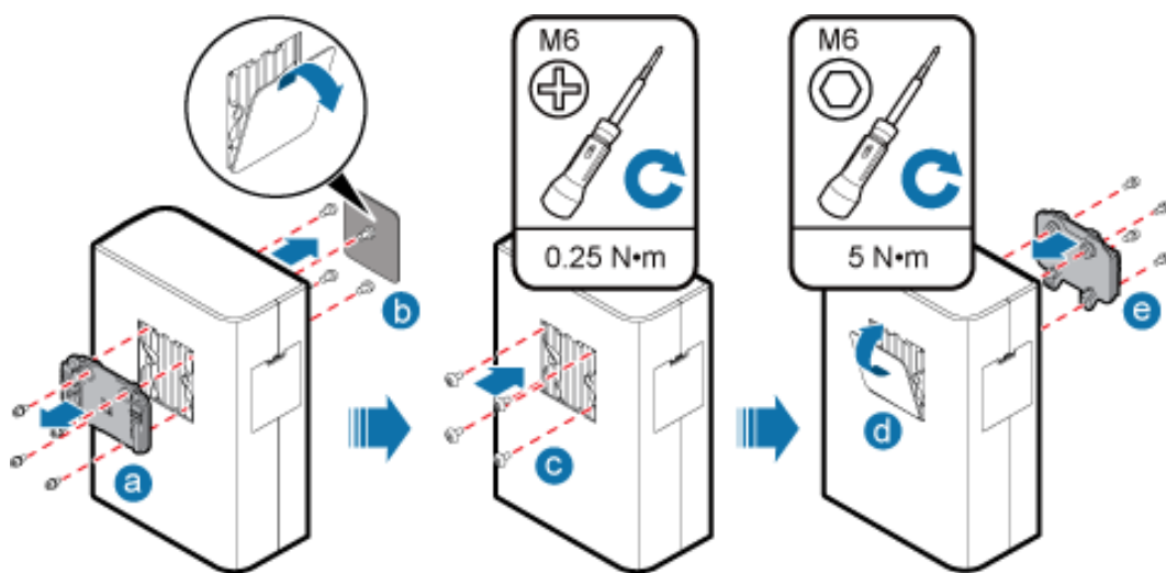
Figure 7-15 Interchanging the cover plate on the front of the second RRU with the attachment plate at the rear of the second RRU
