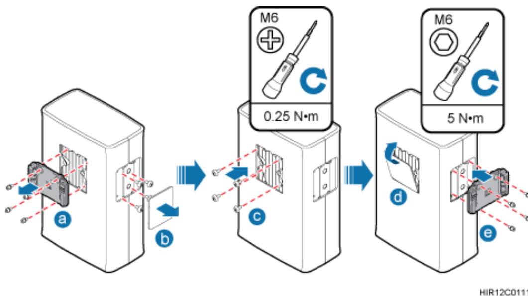
Figure 7-41 Interchanging the attachment plate at the rear of the RRU with the cover plate on one side of the RRU
