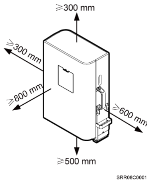
Figure 3-23 Recommended clearance for a single RRU
