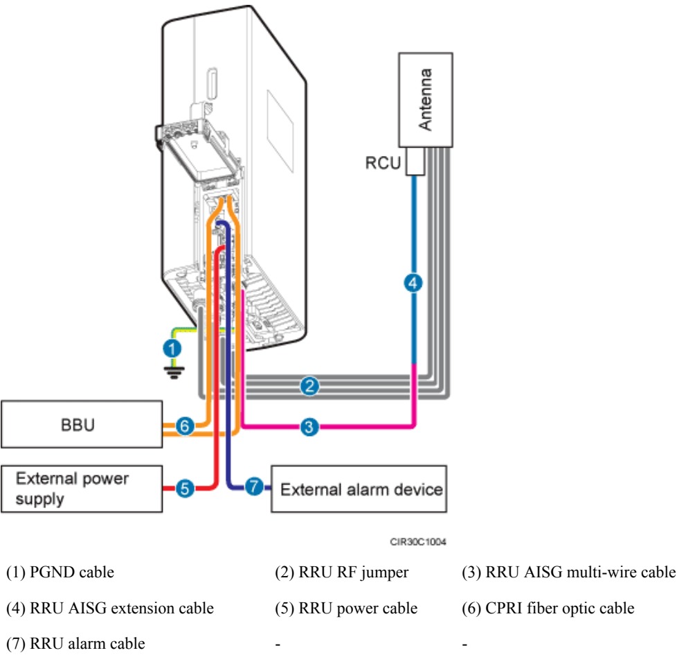
Figure 8-9 Cable connections for a single RRU in the multimode scenario
