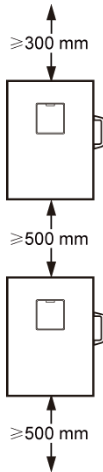
Figure 3-33 Recommended vertical spacing between RRUs
