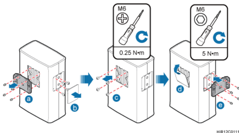
Figure 7-7 Interchanging the attachment plate at the rear of the RRU with the cover plate on one side of the RRU
