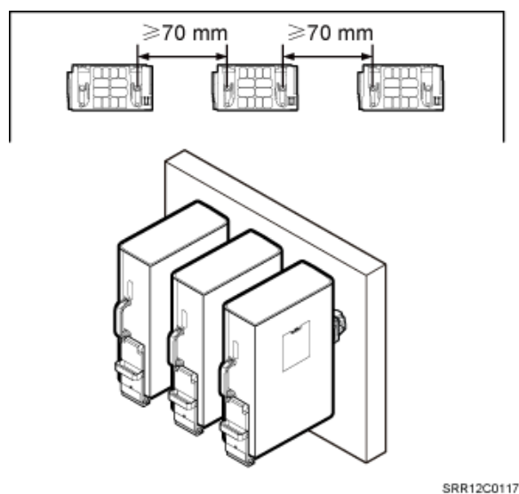
Figure 3-30 Recommended clearances for three or more RRUs installed on a wall in side-mounted mode
