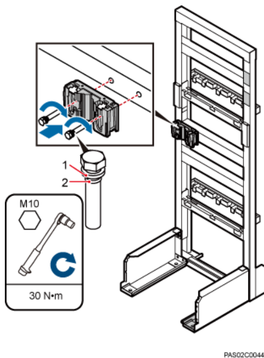
Figure 7-40 Installing the main bracket in height-unrestricted scenarios
