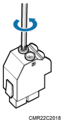
Figure 11-6 Tightening screws
