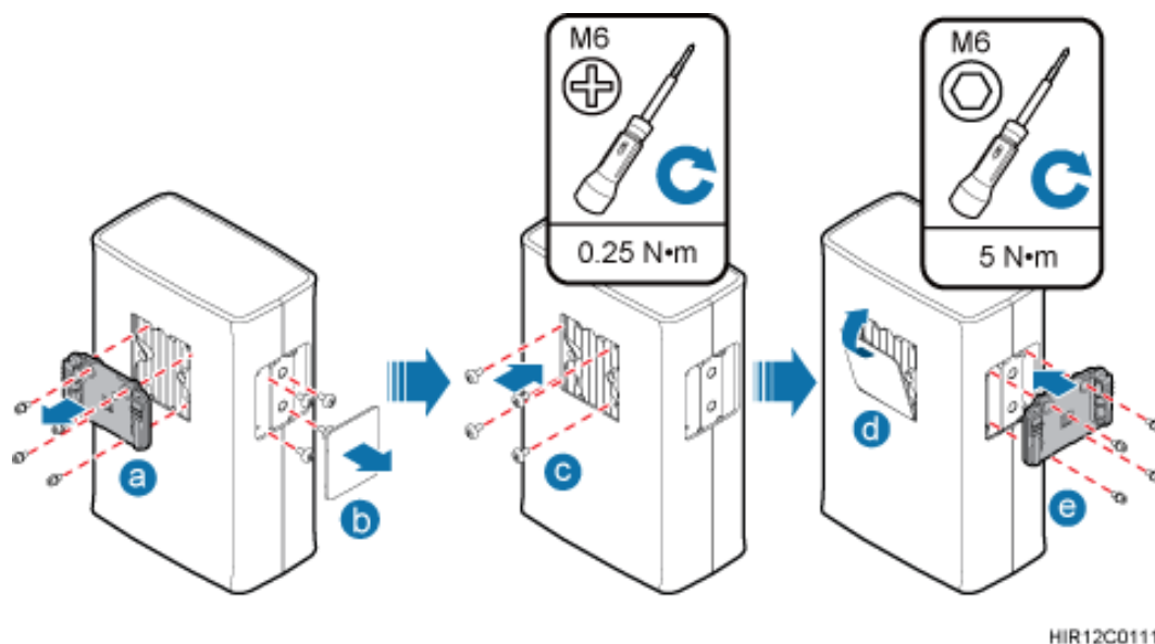
Figure 7-9 Interchanging the attachment plate at the rear of the RRU with the cover plate on one side of the RRU
