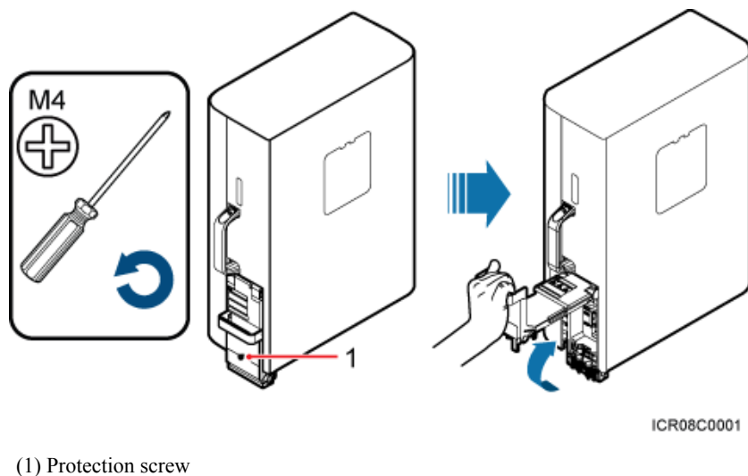
Figure 8-23 Opening the cover plate of the RRU cabling cavity
