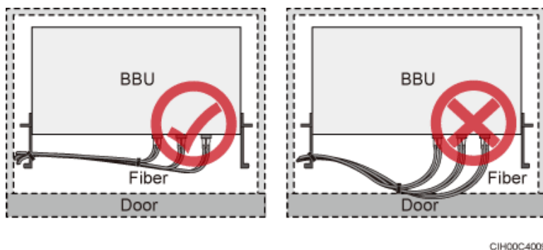
Figure 8-6 CPRI fiber optic cables routed through the cabinet (2)
