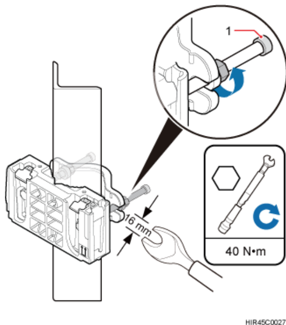
Figure 7-32 Securing the main and auxiliary brackets onto the angle steel
