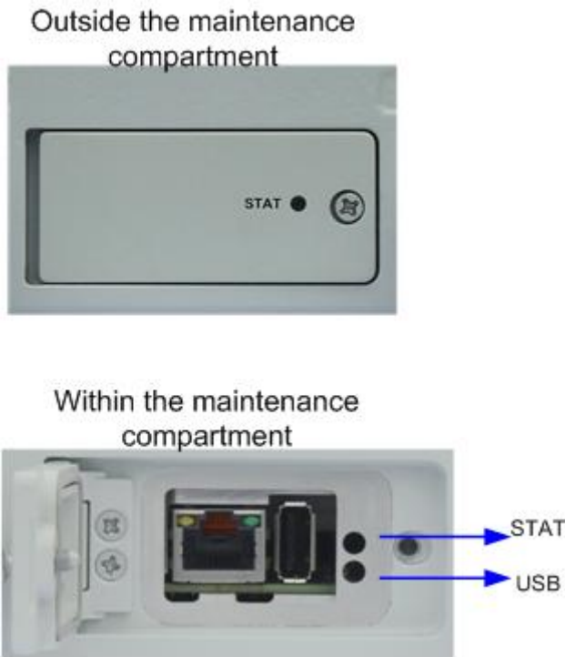
Figure 3-6 Indicator positions
