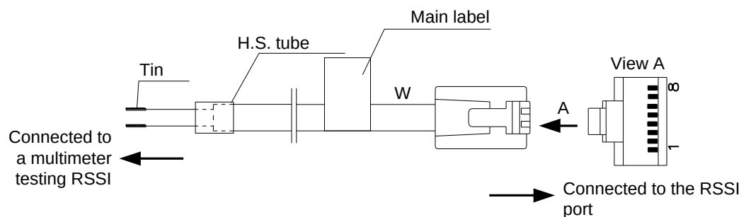
Figure 7-2 RSSI cable
