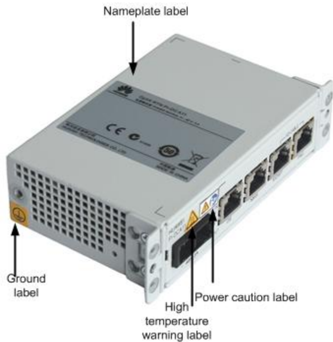
Figure 6-6 Label positions on an indoor PI
