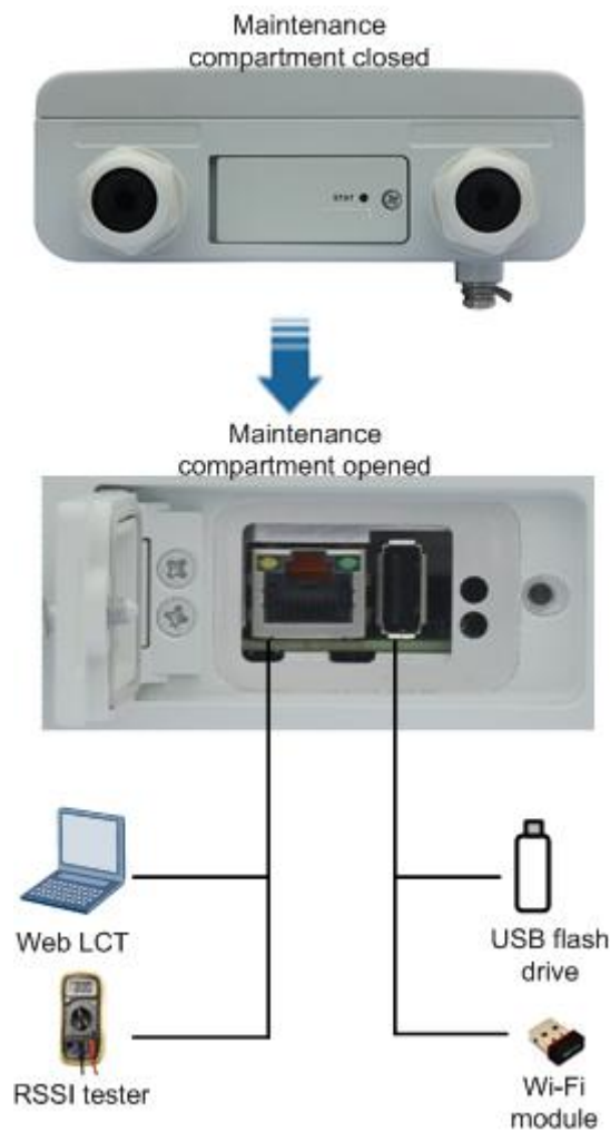
Figure 3-4 Front view of the management ports
