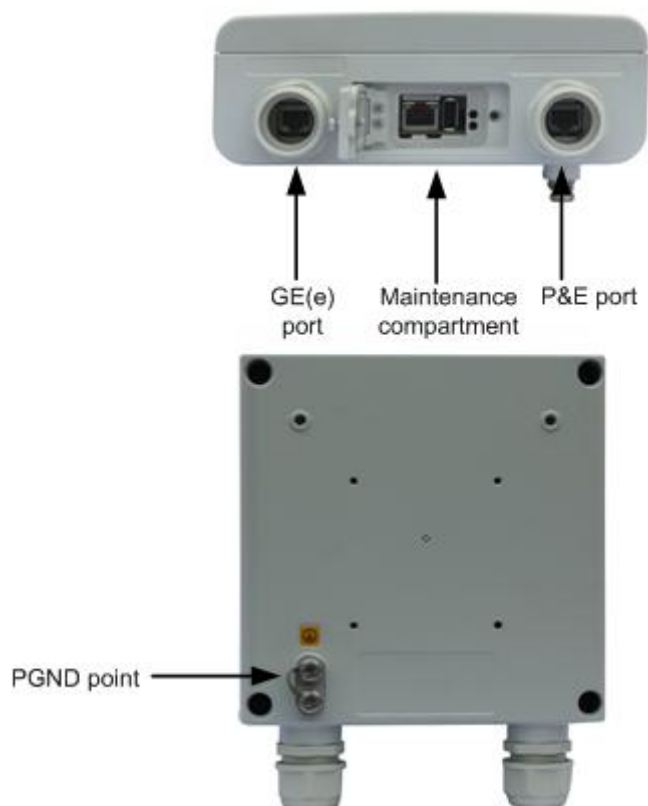
Figure 3-3 Port positions
