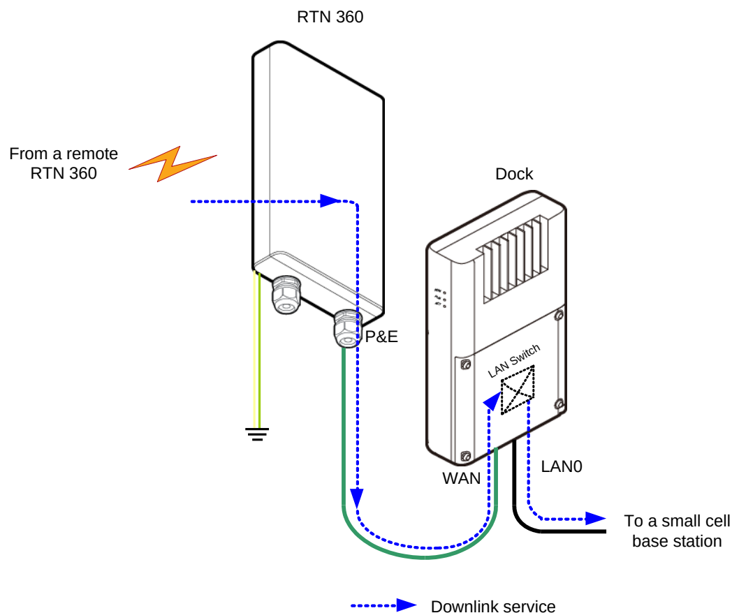
Figure 1-2 Site providing a one-direction microwave link
