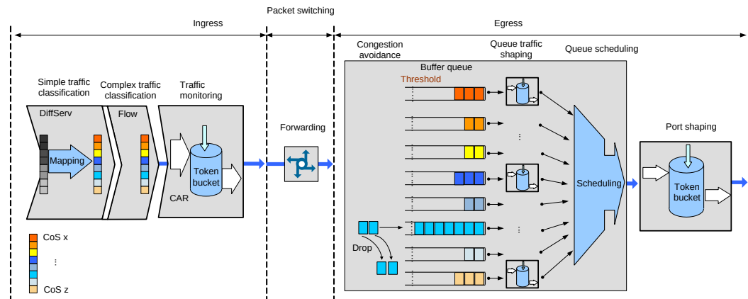
Figure 2-4 QoS processing
