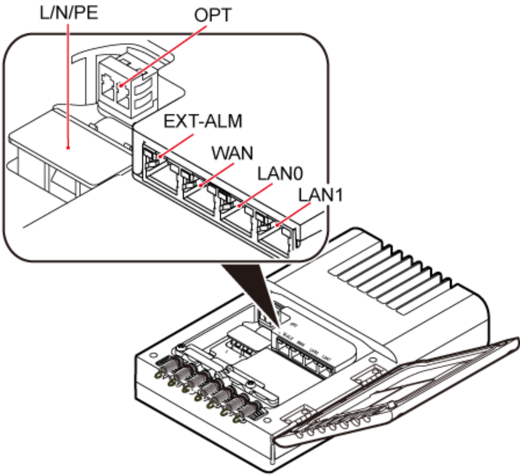
Figure 6-8 Ports
