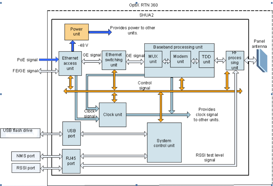
Figure1 Block diagram of RTN 360
