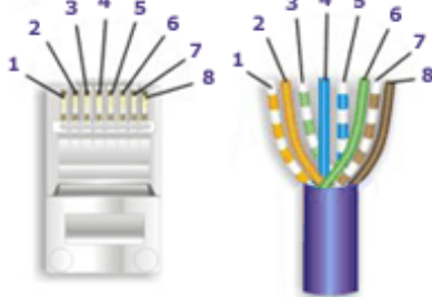
Pin assignments of an RJ45 connector
