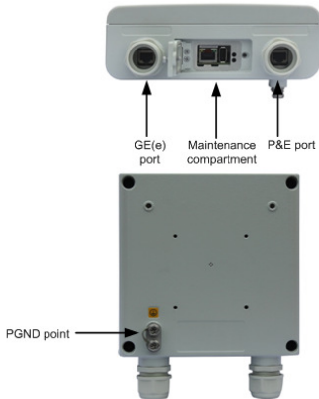
Figure 3-3 Port positions
