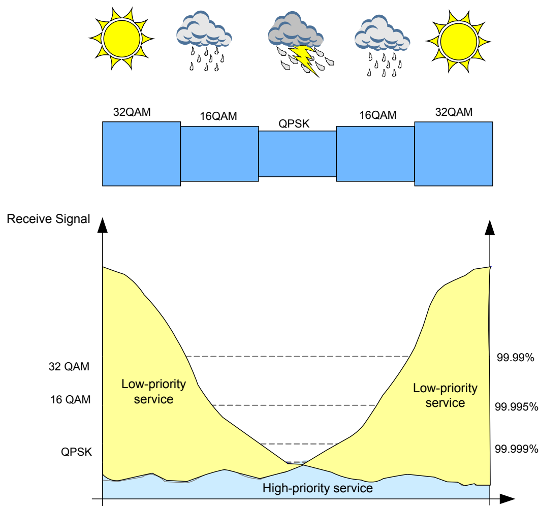
Figure 2-4 Adaptive modulation
