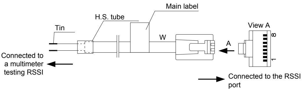
Figure 7-4 RSSI cable
