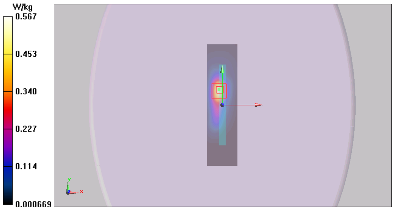
Figure 33 UMTS Band V with Test Position 2 Channel 4183
