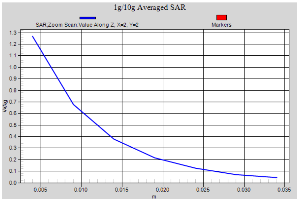
Figure 23 UMTS Band II with Test Position 1 Channel 9538
