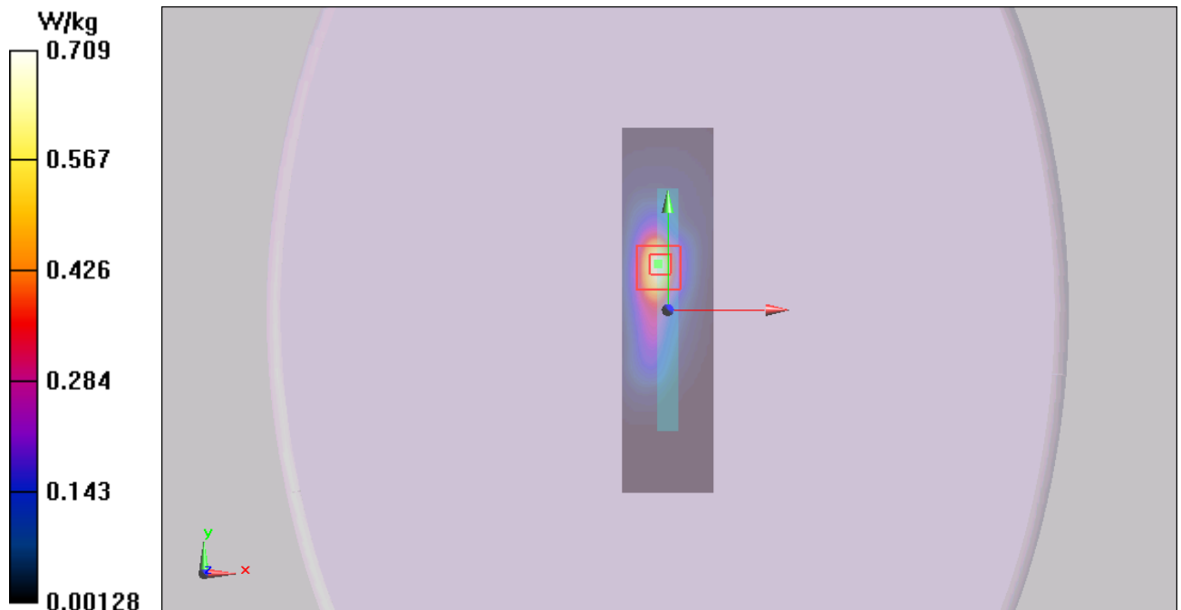
Figure 26 UMTS Band II with Test Position 2 Channel 9400
