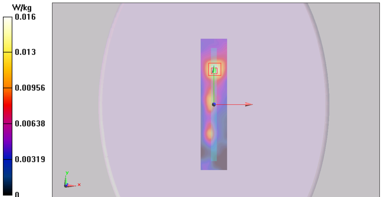
Figure 27 UMTS Band II with Test Position 6 Channel 9400
