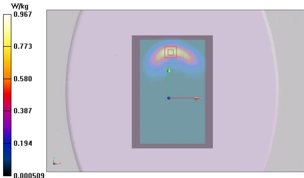
Figure 36 UMTS Band V with Test Position 1 Channel 4132
