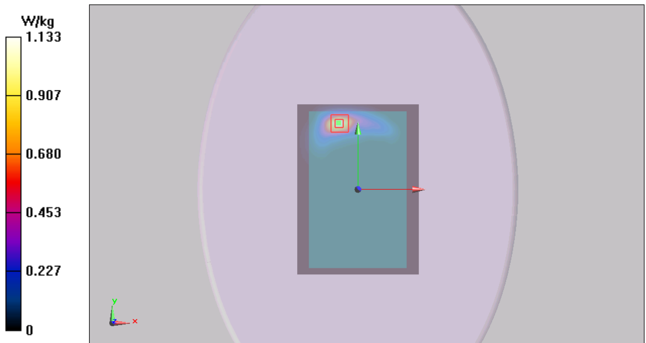
Figure 24 UMTS Band II with Test Position 1 Channel 9400
