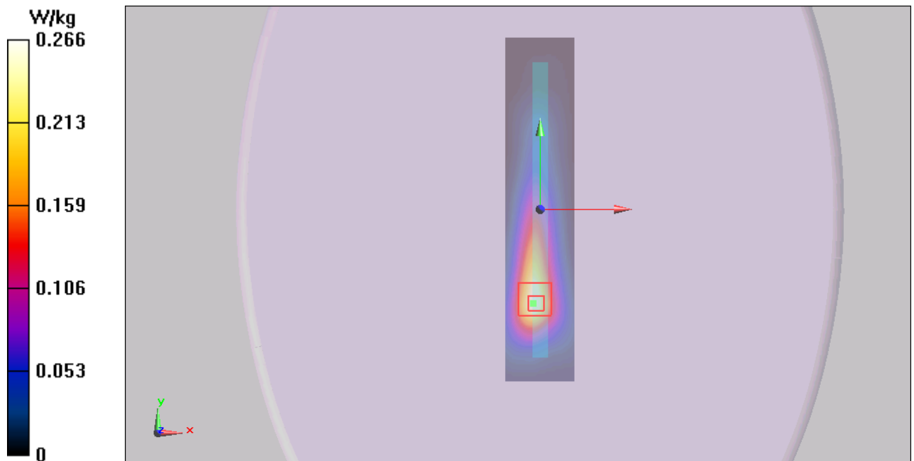
Figure 28 UMTS Band II with Test Position 5 Channel 9400
