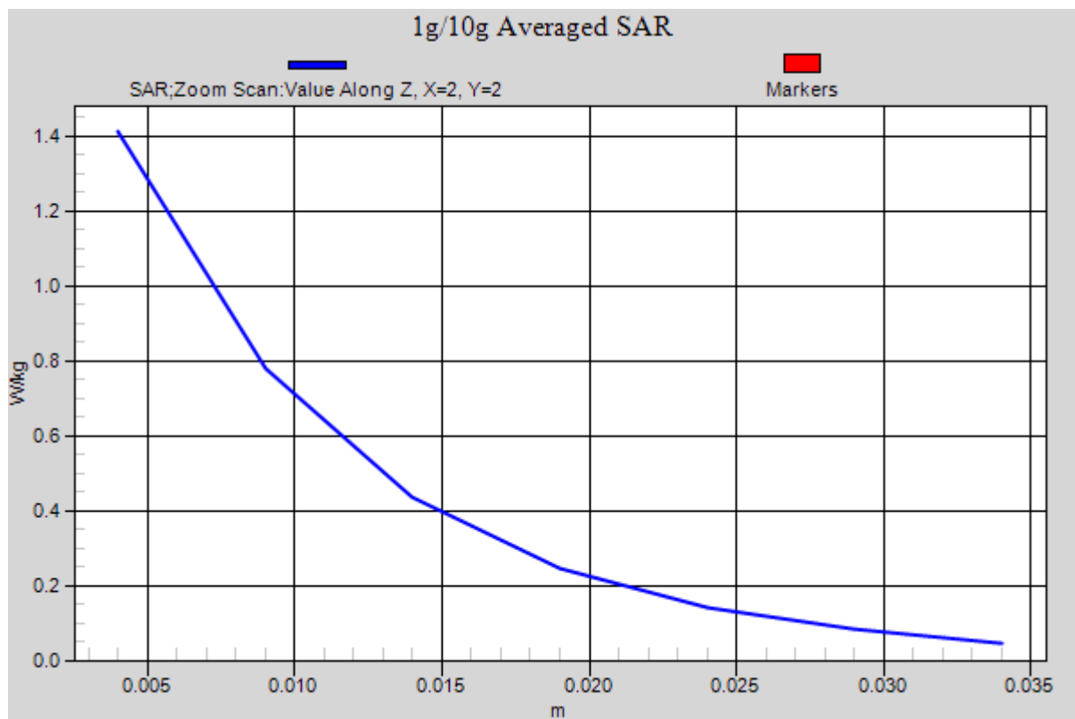
Figure 29 UMTS Band II with Test Position 1 Channel 9538
