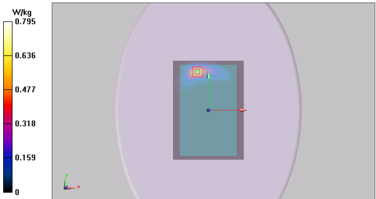
Figure 25 UMTS Band II with Test Position 1 Channel 9262
