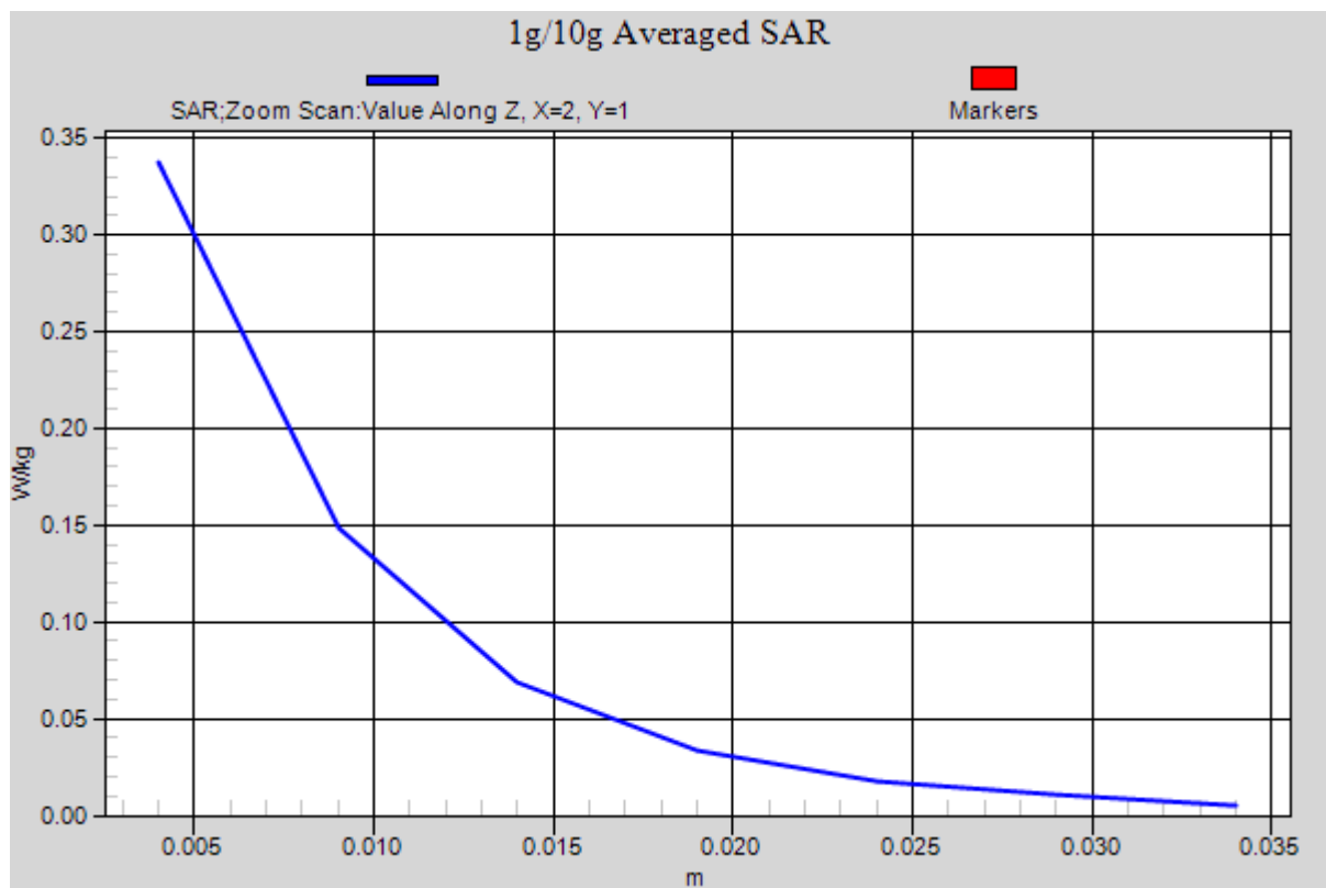
Figure 37 802.11b Test Position 1 Channel 6
