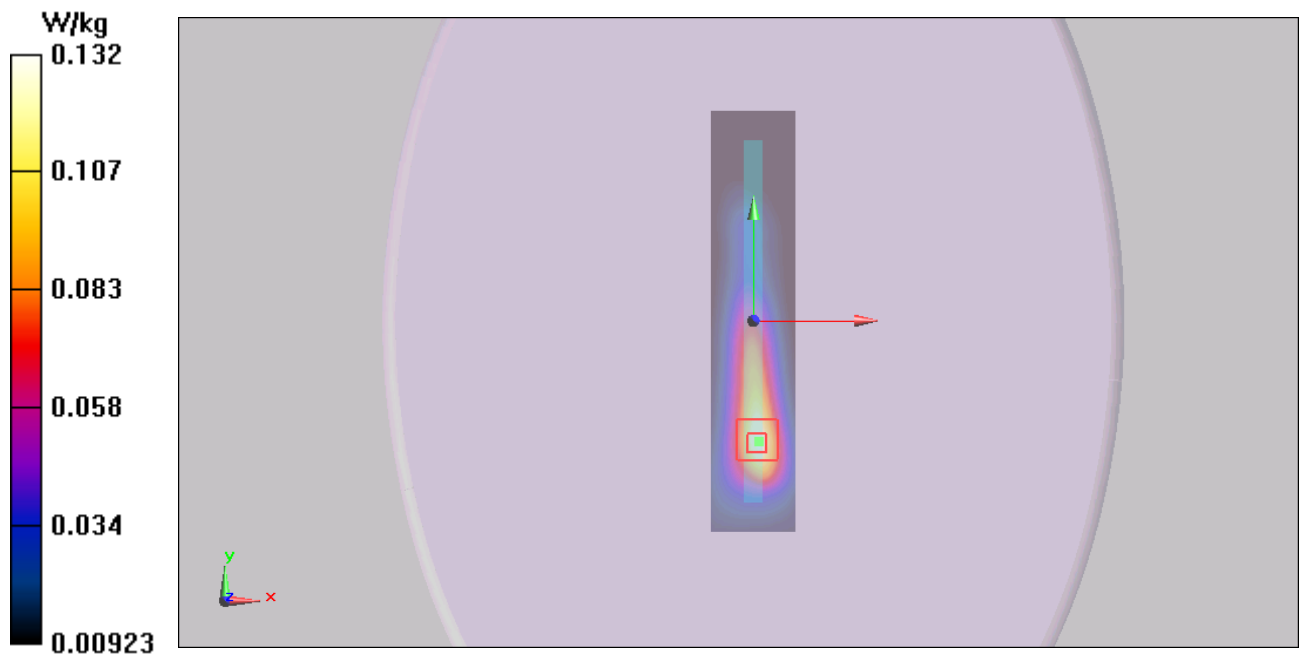
Figure 35 UMTS Band V with Test Position 5 Channel 4183
