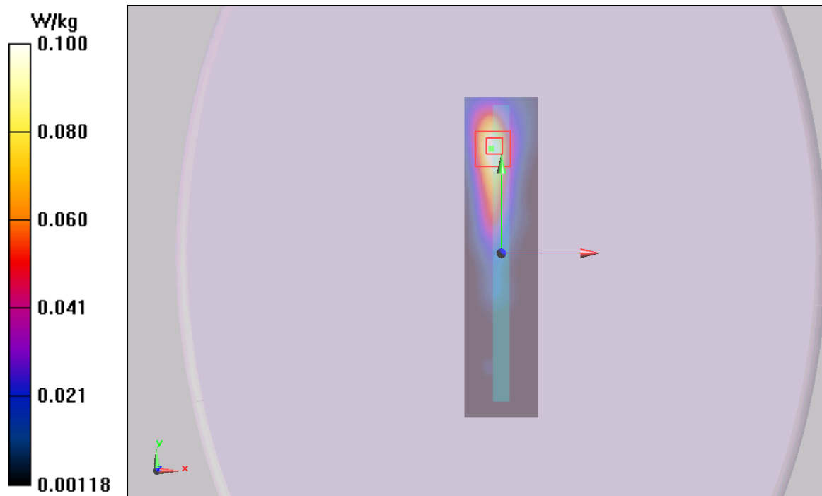
Figure 34 UMTS Band V with Test Position 4 Channel 4183
