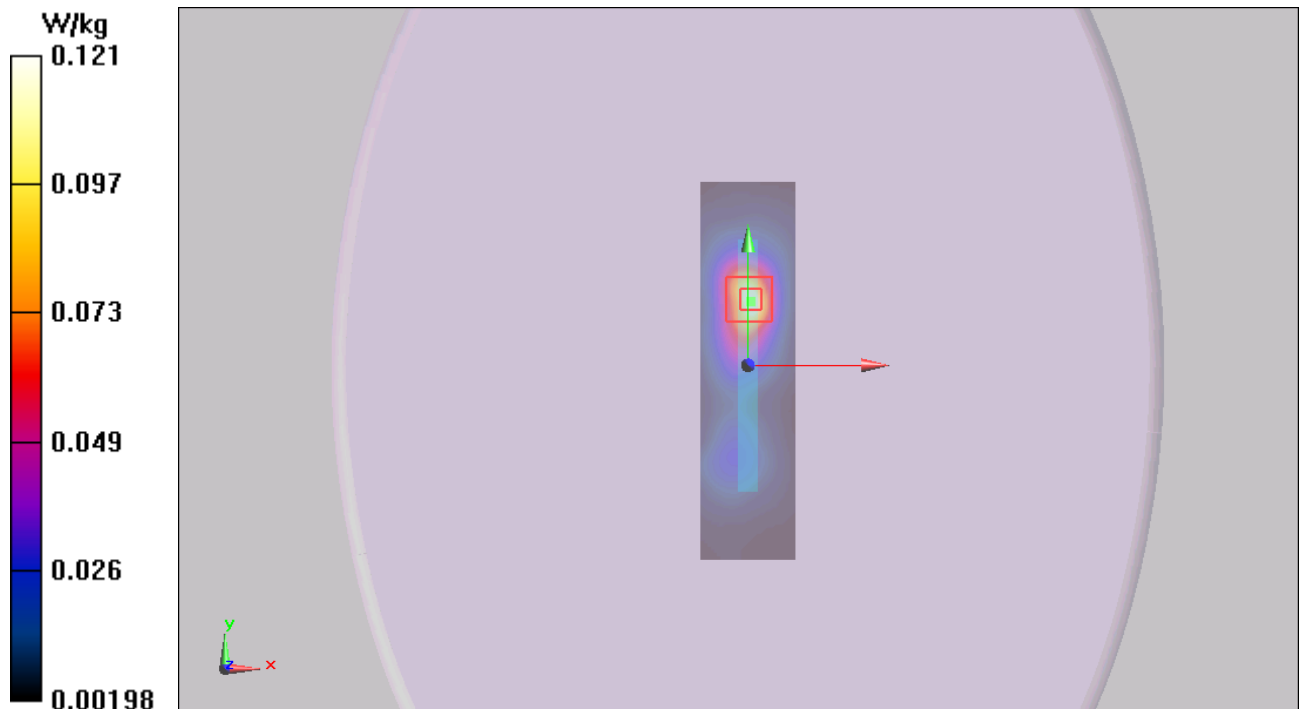
Figure 38 802.11b Test Position 4 Channel 6
