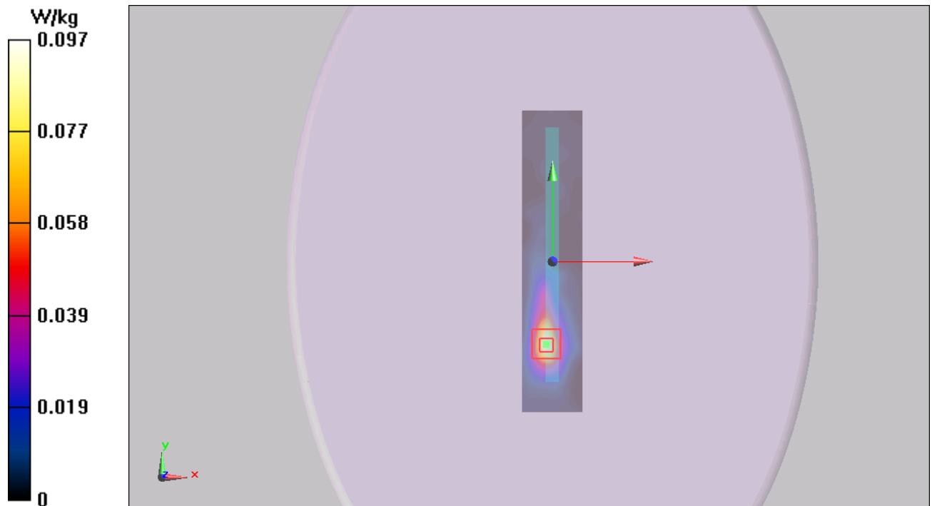
Figure 39 802.11b Test Position 5 Channel 6
