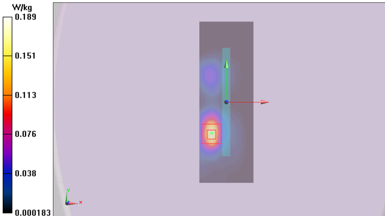
Figure 60 UMTS Band IV with Test Position 3 Channel 1413
