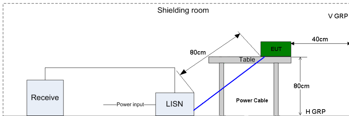
Figure 4. Test Set-up of conducted disturbance
