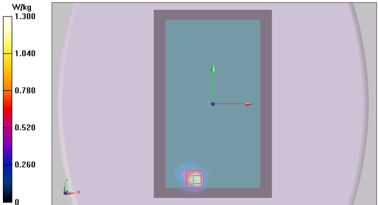
Figure 16 802.11b Test Position 1 Channel 11
