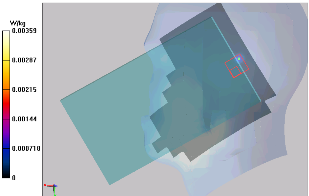
Figure 10 Right Hand Touch Cheek 802.11b Channel 6
