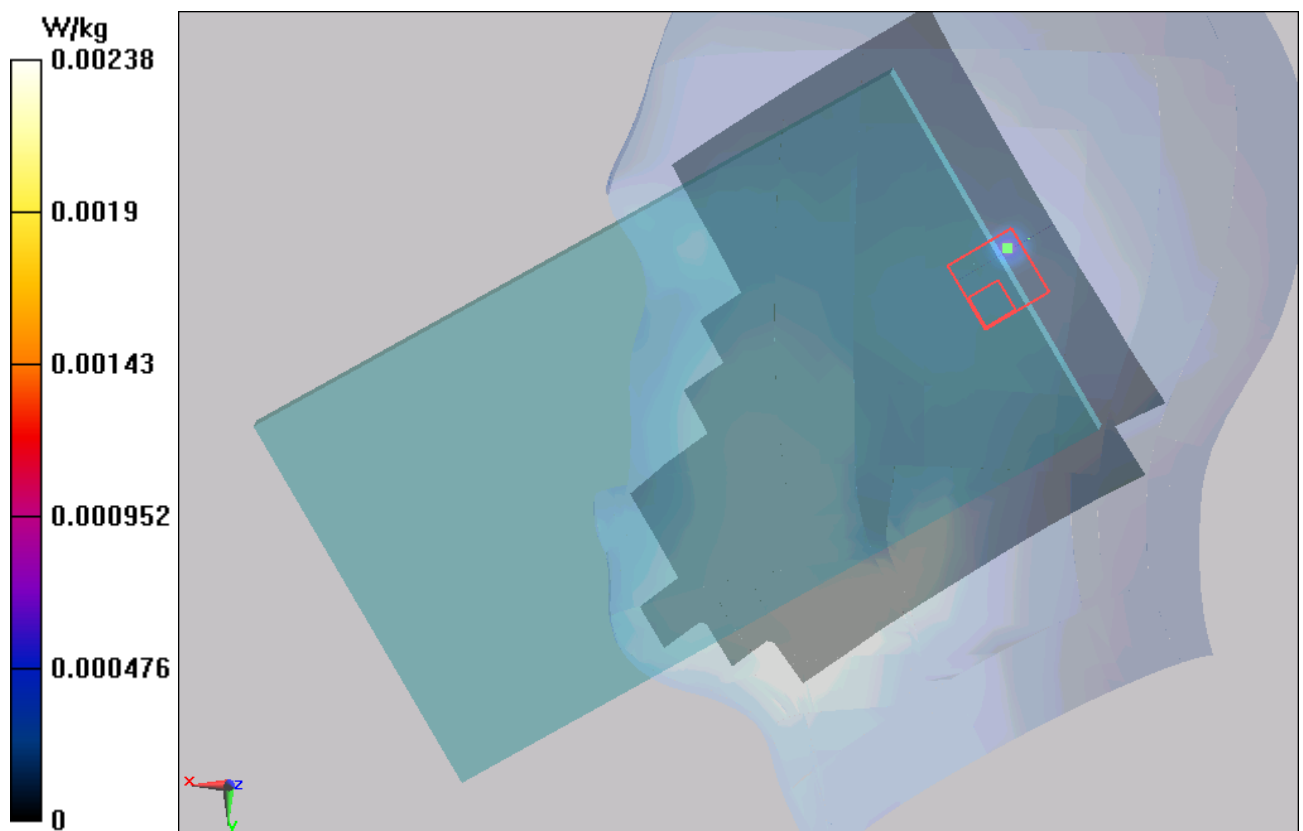
Figure 11 Right Hand Tilt 15° 802.11b Channel 6
