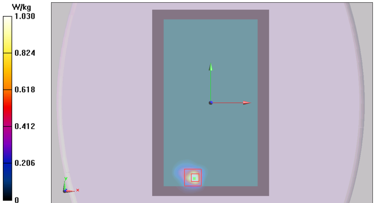
Figure 14 802.11b Test Position 1 Channel 1
