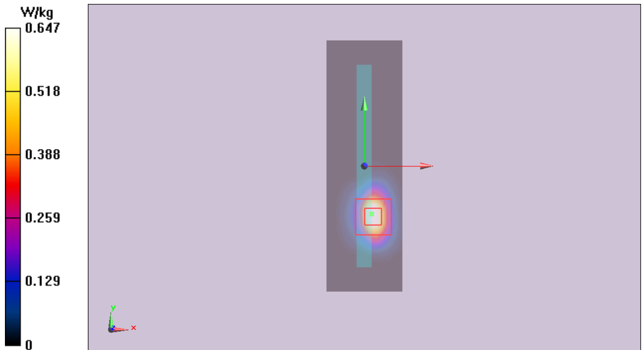
Figure 15 802.11b Test Position 2 Channel 6
