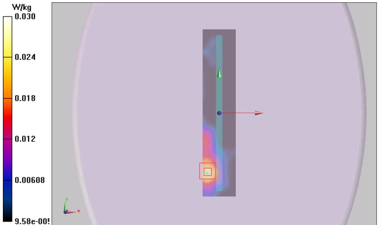
Figure 30 GSM 1900 GPRS (2TXslots) with Test Position 5 Channel 661
