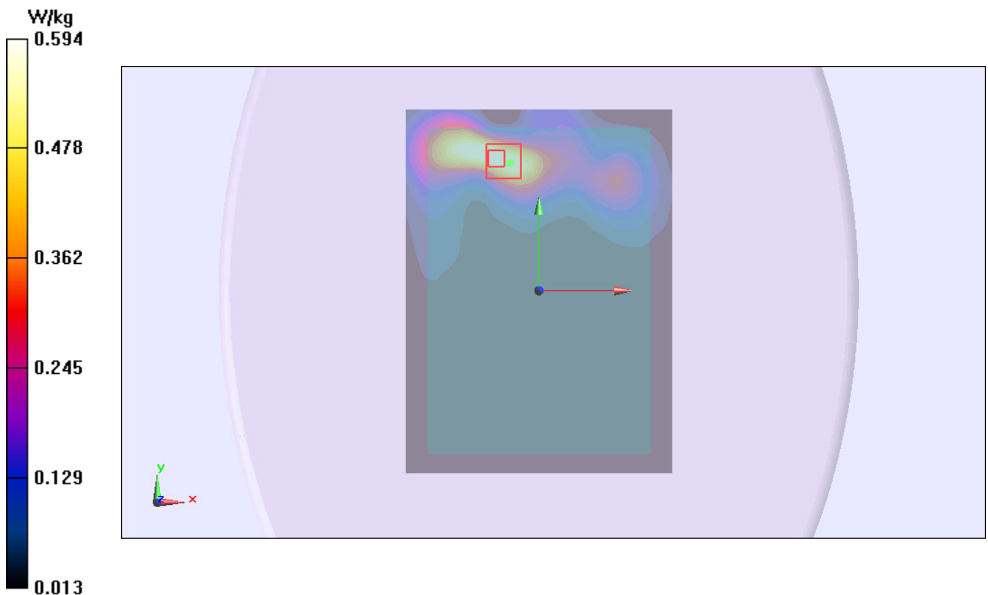
Figure 18 GSM 850 GPRS (2TXslots) with Test Position 1 Channel 128
