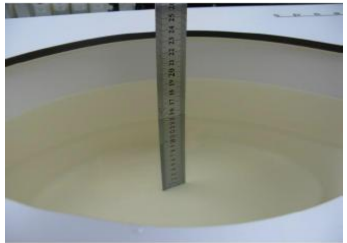
Photo 23: MSL2600MHz depth (15.1cm)
