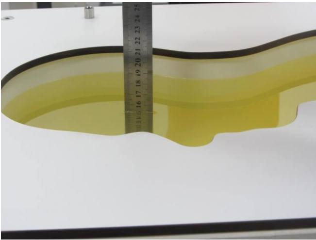
Photo 22: HSL2600MHz depth (15.0cm)
