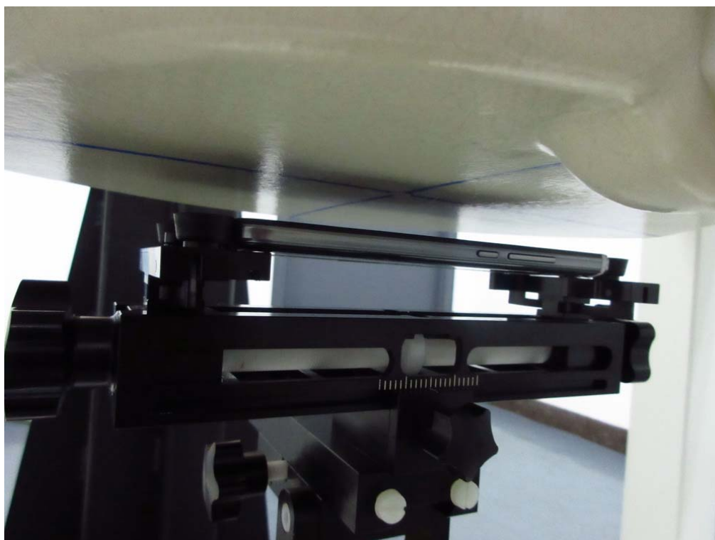
Test Position Rear 15mm
