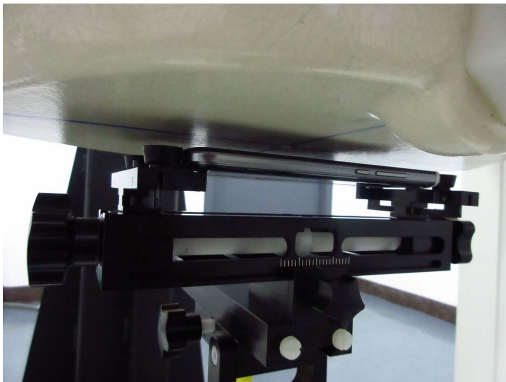
Test Position Rear 10mm
